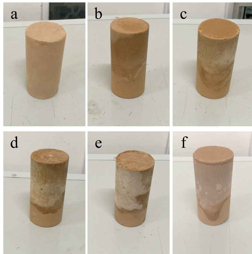
Figure 1. Remolded loess specimens treated with different concentrations of DAP. (a) Untreated; (b) 0.5 mol/L DAP; (c) 1.0 mol/L DAP; (d) 1.5 mol/L DAP; (e) 2.0 mol/L DAP; (f) 3.0 mol/L DAP.
