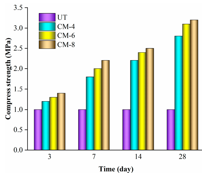
Figure 2. Compressive strength of cement-treated loess specimens.
