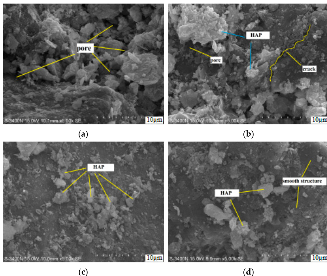
Figure 8. SEM images of loess specimens treated with different contents of DAP for 3 d of curing. (a) 0.5 mol/L; (b) 1.0 mol/L; (c) 1.5 mol/L; (d) 2.0 mol/L.
