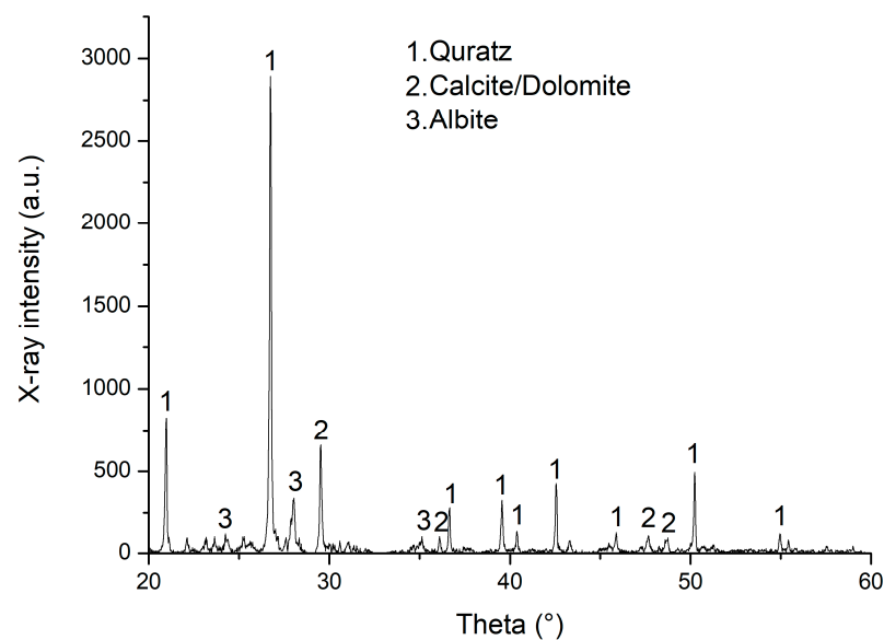
Figure 4. XRD patterns of untreated loess.
