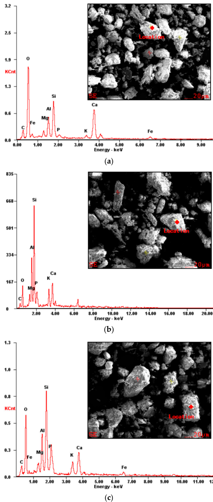
Figure 7. EDX results and SEM images (insets) of loess specimens treated with different contents of DAP. (a) 1.0 mol/L; (b) 2.0 mol/L; (c) 3.0 mol/L. The yellow and red crosses is other scanning location for EDX in the insert images, the red blocks is the correspond-ing scanning location of EDX.
