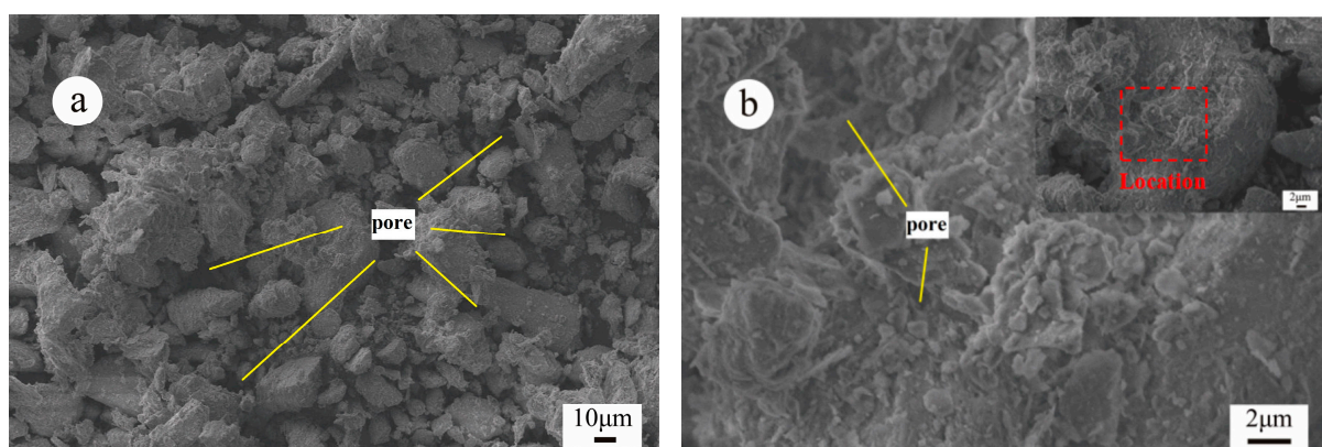
Figure 5. SEM images of untreated loess. (a) Pore structure in loess; (b) surface morphology of loess particles.
