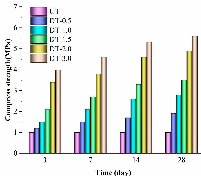
Figure 3. Compressive strength of DAP-treated loess specimens.
