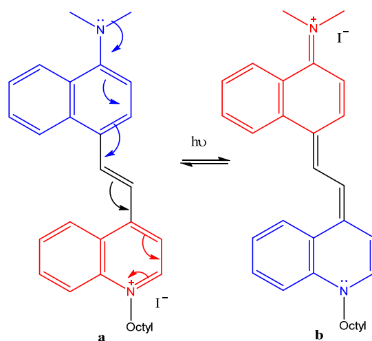
Figure 8. Ground state (benzoid form) (a) and excited state (quinoid form) (b) of the chromophore of compound ( D ).
