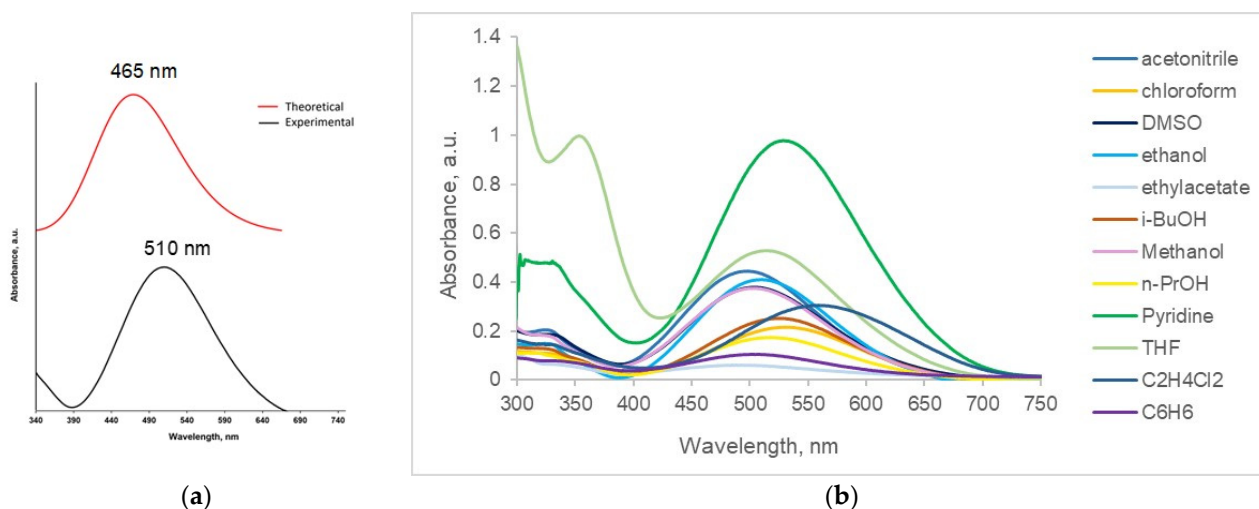
Figure 9. Theoretical (a) and experimental (b) UV-Vis spectra of compound ( D ) in ethanol.
