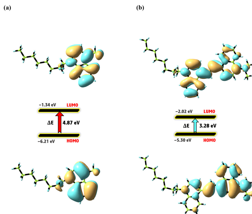
Figure 7. Distributions and energy surfaces of the molecular orbitals of compounds B (a) and D (b).
