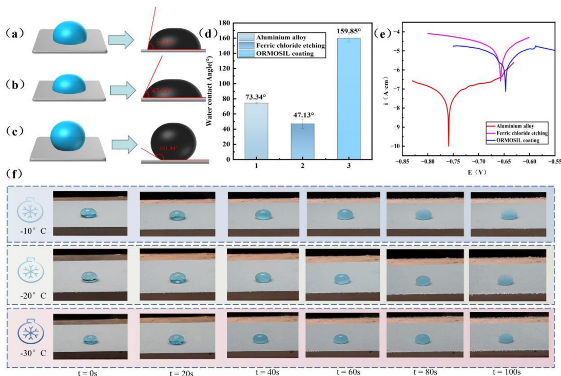
Figure 5. (a–c) Water contact angle images and measured values on aluminum alloy surfaces under different treatment conditions; (d) Bar chart of average water contact angles; (e) Potentiodynamic polarization curves; (f) Time-lapse images of icing-delay tests on ORMOSIL-coated samples at -10^{\circ}\text{C} , -20^{\circ}\text{C} , and -30^{\circ}\text{C} .
