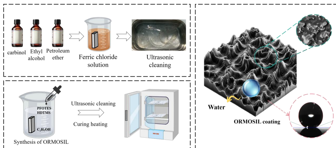
Figure 2. Illustration of the experimental procedure.
