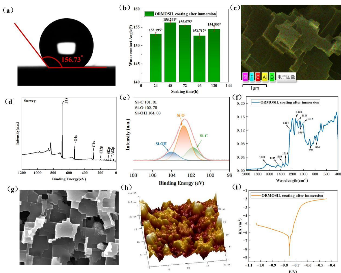
Figure 6. Characterization and performance tests of the ORMOSIL coating after jet fuel immersion: (a) water contact angle image showing the maximum value; (b) average water contact angle versus immersion time; (c) EDS elemental mapping; (d) XPS survey spectrum; (e) high-resolution Si 2p XPS spectrum; (f) FTIR spectrum; (g) SEM image; (h) AFM 3D surface morphology; and (i) polarization curve.
