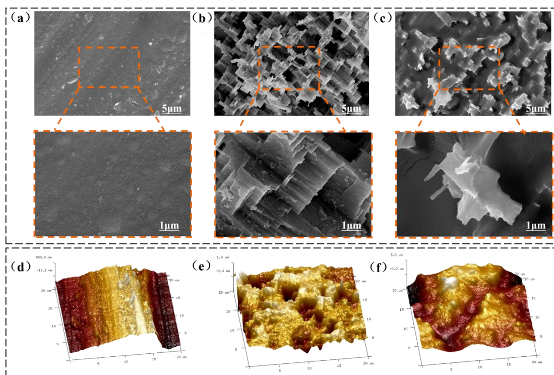
Figure 4. (a–c) SEM images of aluminum alloy, \text{FeCl}_3 -etched aluminum alloy, and the ORMOSIL-coated surface; (d–f) AFM 3D topography images of aluminum alloy, \text{FeCl}_3 -etched aluminum alloy, and the ORMOSIL-coated surface.
