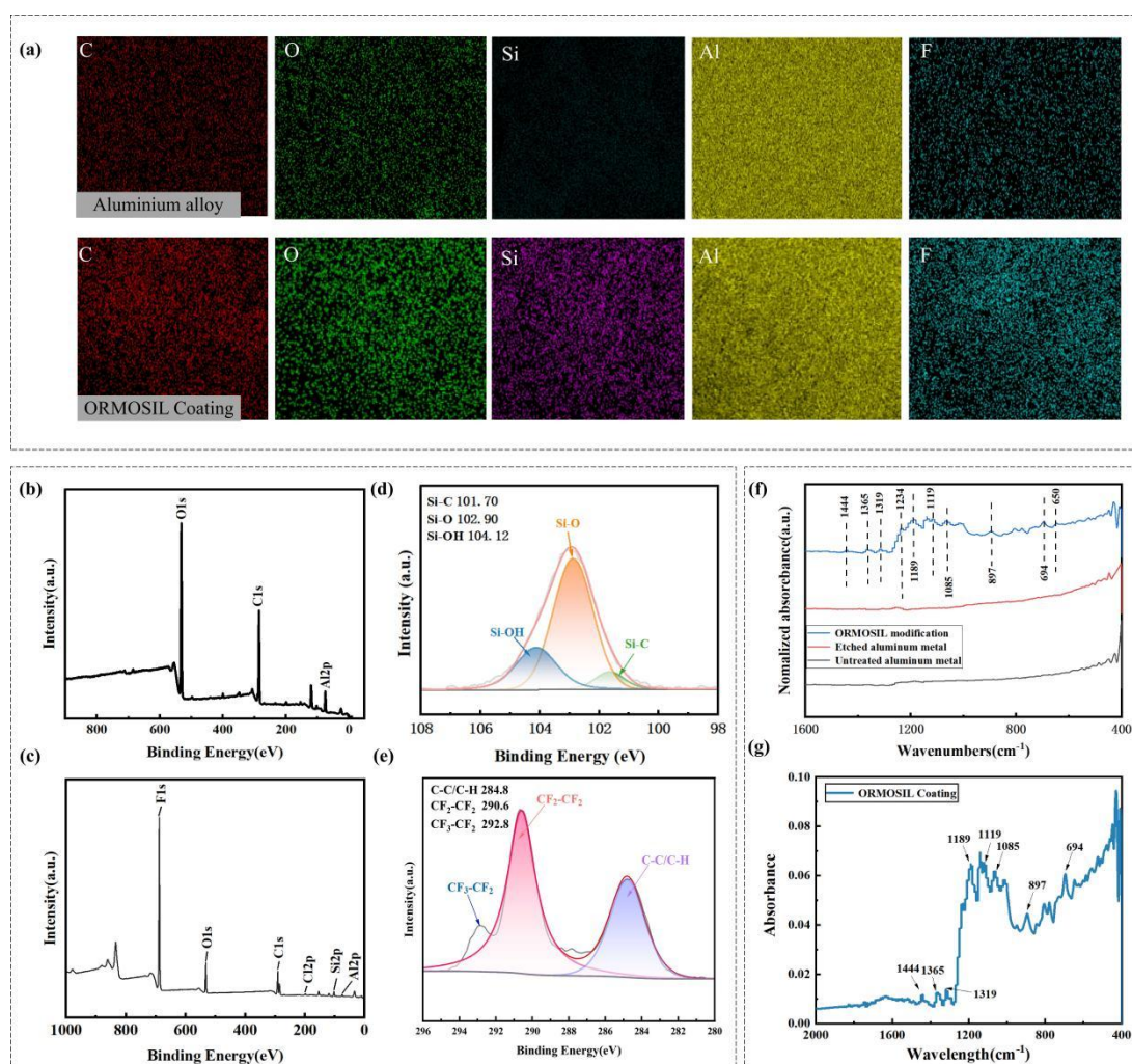
Figure 3. (a) EDS elemental mapping of aluminum alloy and ORMOSIL-coated samples; (b,c) XPS survey spectra; (d,e) High-resolution XPS spectra of Si 2p and C 1s; (f) FTIR spectrum; (g) magnified FTIR spectrum of the ORMOSIL coating.
