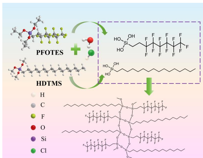
Figure 1. Schematic illustration of the hydrolysis and condensation of PFOTES and HDTMS to form the ORMOSIL siloxane network.
