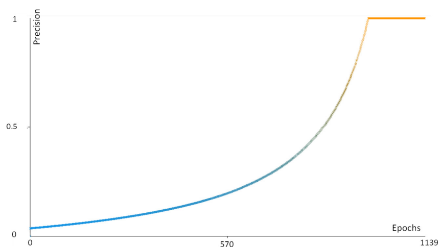
Figure A1. Precision versus epoch number (sample NM8).
