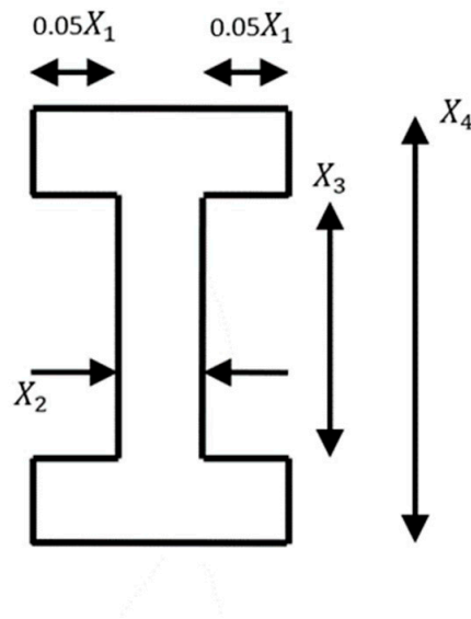
Figure 2. I Beam cross section.
