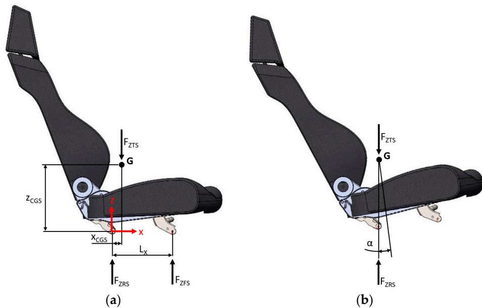
Figure 1. Car seat with forces on supports when measuring (a) the longitudinal x and (b) the vertical z coordinates of the CG.
