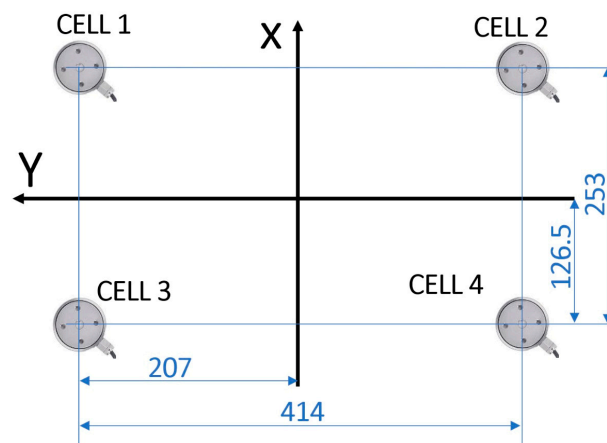
Figure 5. Distances of the four supports for weighing the signals when calculating the position of the CG in travel x and transverse y directions.
