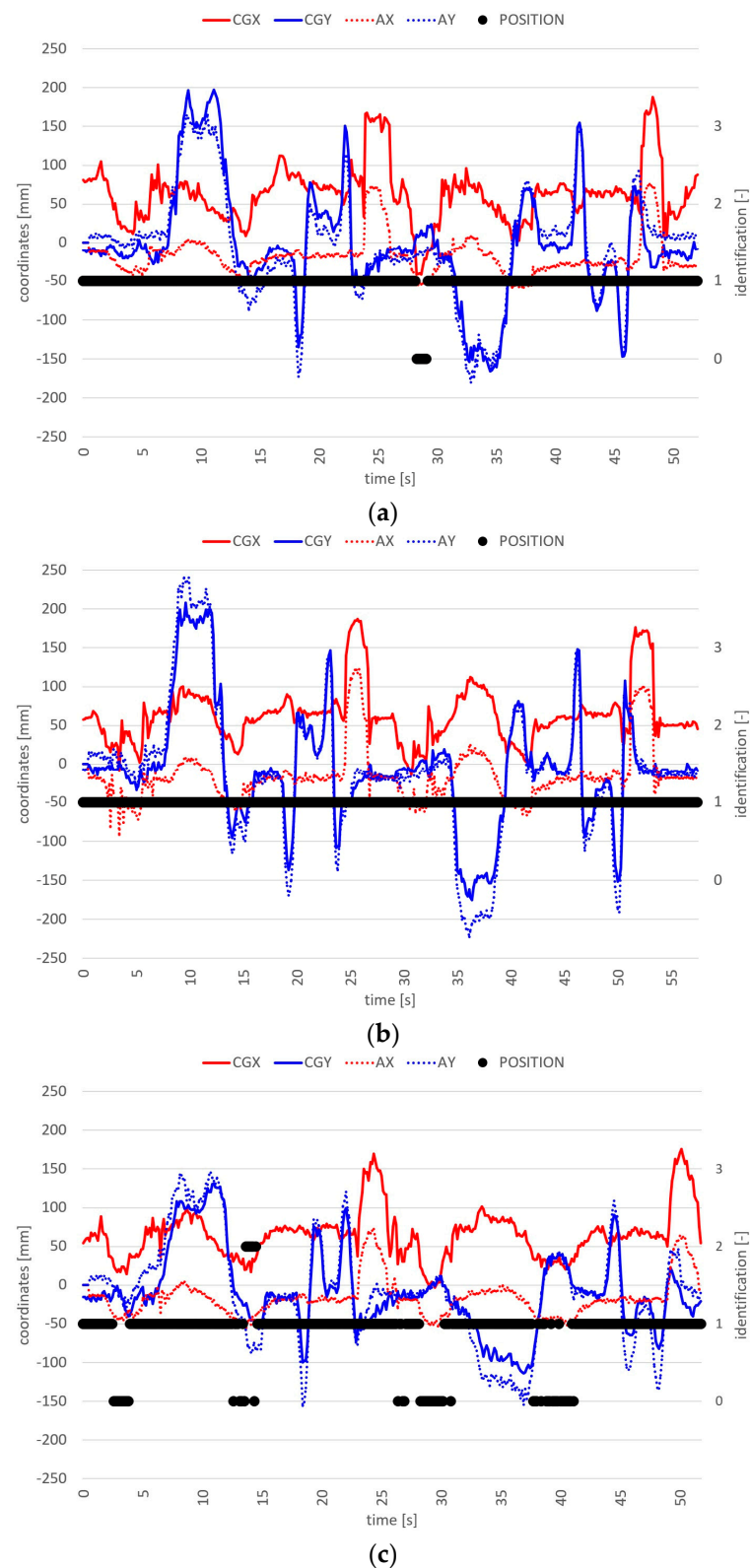
Figure 13. Second test of three, in forward-reclined OP for (a) 1st, (b) 2nd, and (c) 3rd drivers.
