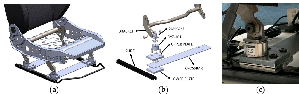
Figure 3. Assembly layout of the DYZ-101 load cells under the seat supports: (a) complete layout, (b) exploded view, and (c) assembled support.
