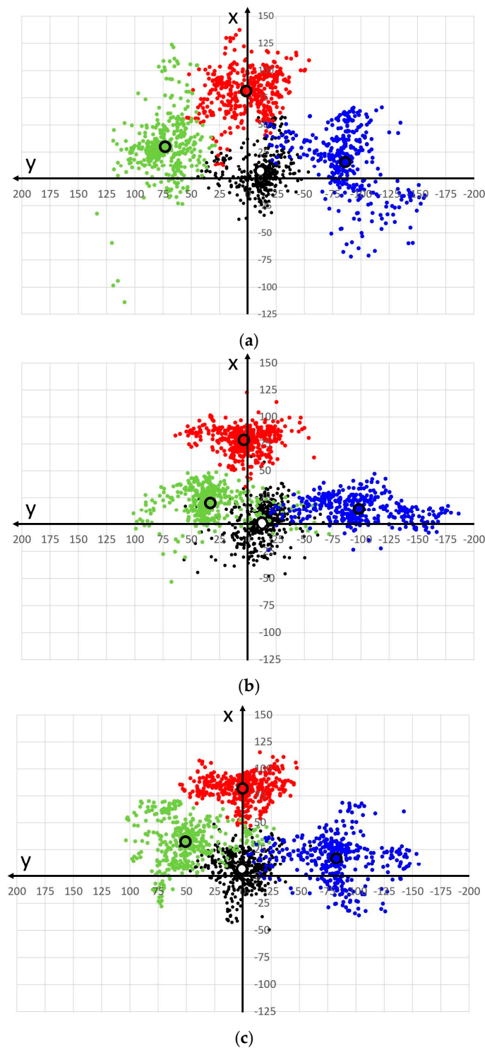
Figure 16. CG positions reduced by the scaled accelerations for the second test of three, in normal position (black), forward-(red), and left-(green) and right-reclined (blue) OPs, for (a) 1st, (b) 2nd, and (c) 3rd drivers.
