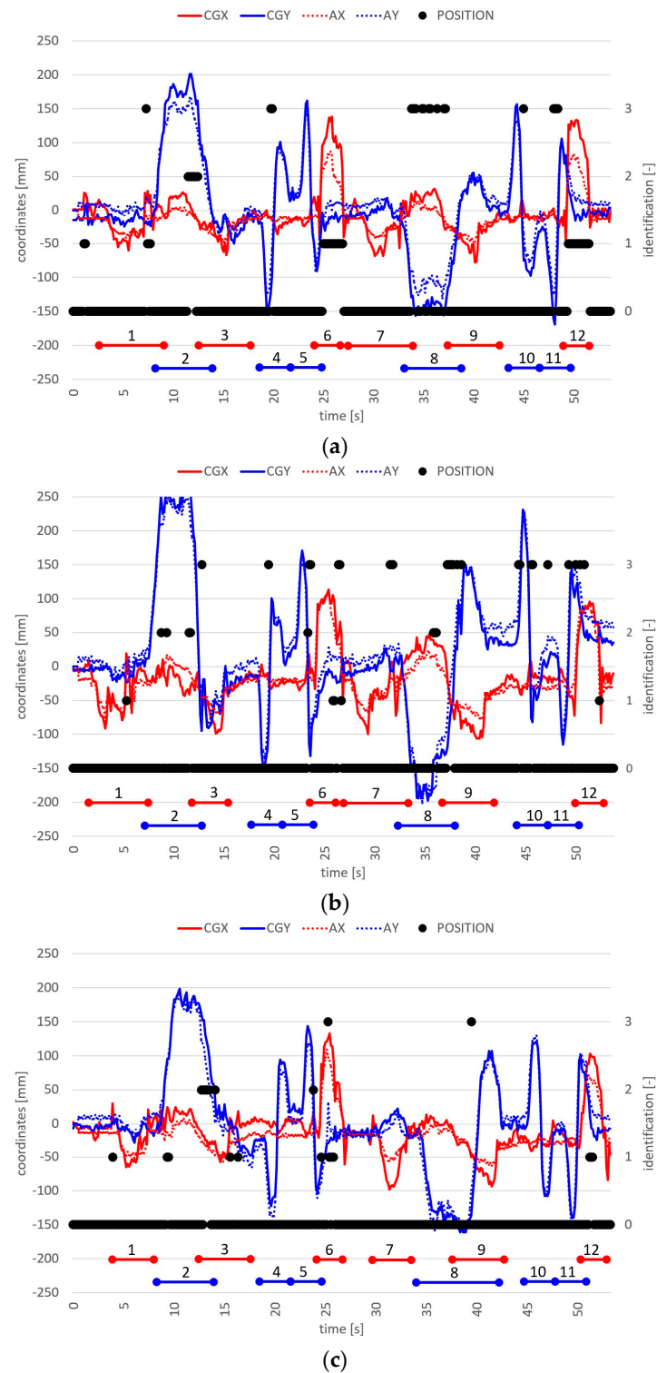
Figure 12. Second test of three, in normal position for (a) 1st, (b) 2nd, and (c) 3rd drivers.
