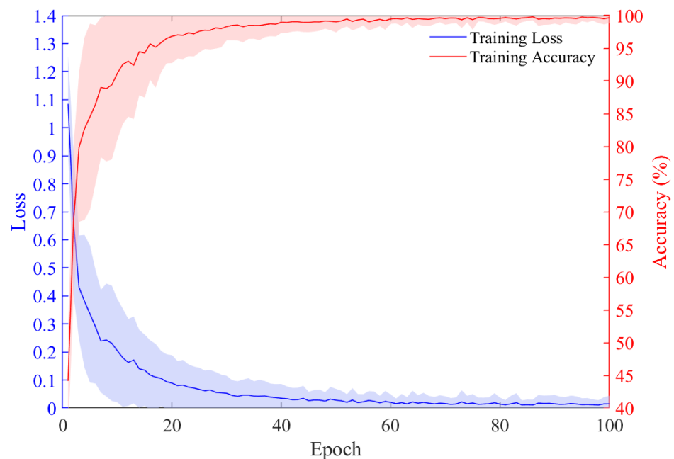
Figure 7. Average cross-entropy training loss and average training accuracy curves for 23 patients in the CHB-MIT dataset. The shaded region indicates the standard deviation.
