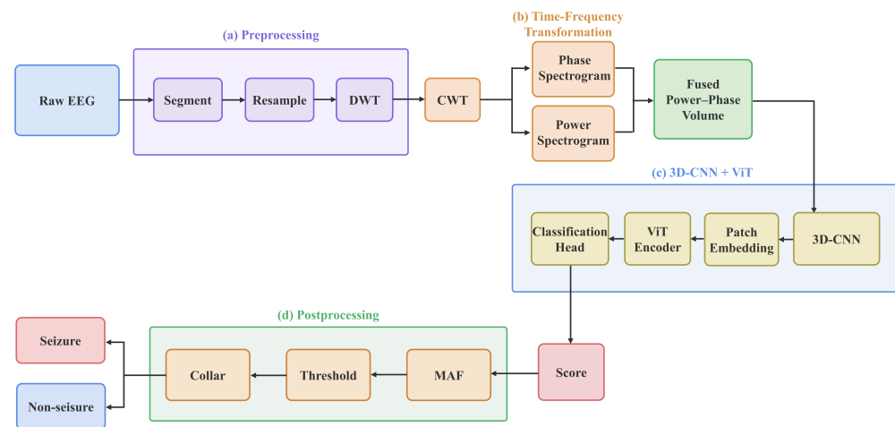
Figure 1. Workflow of the proposed seizure detection framework. The preprocessing module includes signal segmentation, EEG resampling, and the discrete wavelet transform (DWT). The time–frequency module uses the continuous wavelet transform (CWT) to generate phase and power spectrograms and to construct fused features. The deep learning module integrates a 3D-CNN, patch embedding, a ViT encoder, and a classification head. The postprocessing module consists of moving-average filtering (MAF), thresholding, and collar correction.
