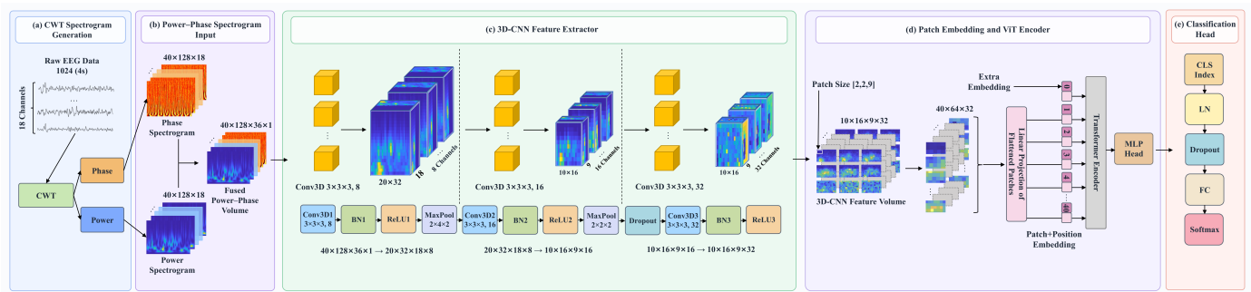
Figure 3. Schematic of the hybrid 3D-CNN-ViT architecture. (a) CWT power and phase spectrograms generated from raw 4-s, 18-channel EEG segments. (b) Power and phase spectrograms are represented as time–frequency volumes of size 40 \times 128 \times 18 and then concatenated along the depth dimension to form a fused power-phase volume of size 40 \times 128 \times 36 \times 1 . (c) The 3D-CNN feature extractor consists of three convolutional blocks. The first two are followed by batch normalization, ReLU activation, and 3D max pooling; dropout is inserted after the second block; the third block contains convolution, batch normalization, and ReLU activation only. (d) The convolutional feature volume is mapped into a token sequence by patch embedding and then passed, together with a learnable CLS token and positional encoding, into a single-layer ViT encoder. (e) The classification head outputs seizure and non-seizure probabilities through CLS indexing, layer normalization, dropout, a fully connected layer, and softmax.
