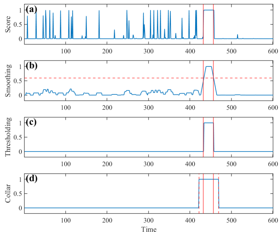
Figure 6. Illustration of the postprocessing procedure applied to the model output scores. (a) Raw output score sequence of the model. (b) Score sequence after smoothing with moving-average filtering (MAF), where the red horizontal dashed line indicates the threshold. (c) Binary decisions after thresholding. (d) Final detection results after additional collar correction. In the figure, the red vertical solid lines indicate expert-annotated seizure intervals, and the red vertical dashed lines indicate the collar-expanded detection boundaries.
