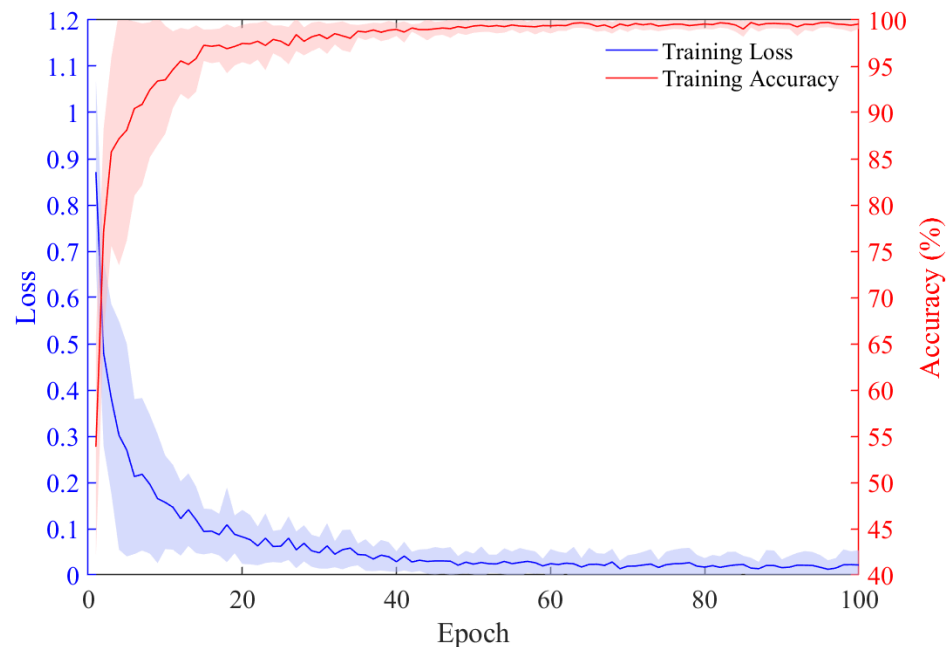
Figure 8. Average cross-entropy training loss and average training accuracy curves for 6 patients in the SH-SDU dataset. The shaded region indicates the standard deviation.
