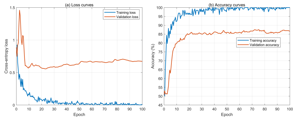
Figure 5. Training and validation loss/accuracy curves for CHB-MIT Patient 12. The held-out validation subset consisted of 200 seizure segments and 200 non-seizure segments that were not used for model parameter updating. The validation accuracy remained stable at approximately 86–87% in the later epochs.
