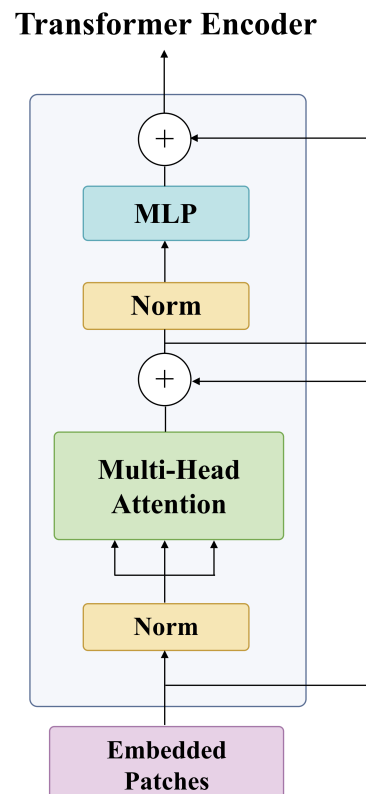
Figure 4. Schematic of the Transformer encoder. The encoder consists of a layer normalization module, a multi-head self-attention module, and a multilayer perceptron module.
