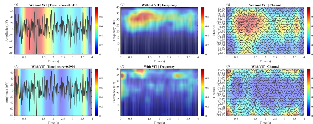
Figure 10. Grad-CAM visualization of a representative corrected false-negative seizure segment from Patient 12 in the CHB-MIT dataset. The seizure class was used as the target class. (a–c) Temporal, frequency–time, and channel–time Grad-CAM responses of the 3D-CNN-only model without the ViT branch, respectively. (d–f) Corresponding responses of the full 3D-CNN-ViT model. For both models, Grad-CAM was computed with respect to the last 3D-CNN activation feature map before patch embedding. In the full model, gradients were further backpropagated from the final seizure-class score through the ViT encoder and patch embedding module to this feature map. Warmer colors indicate larger positive contributions to the seizure-class decision.
