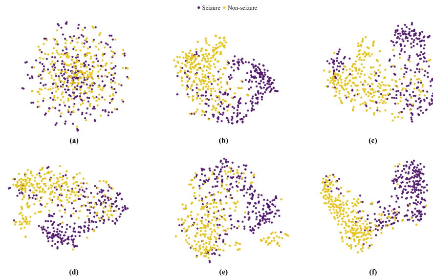
Figure 9. t-SNE visualization of feature representations at different stages of the proposed model using unseen testing samples from CHB-MIT Patient 12. A balanced subset containing all 275 seizure testing samples and 275 randomly selected non-seizure testing samples was used. (a) Original EEG. (b) Fused CWT input. (c) Feature representation after the first 3D max-pooling layer. (d) Feature representation after the second 3D max-pooling layer. (e) Deep 3D-CNN feature representation. (f) Final ViT feature representation. The final feature space shows clearer separation between seizure and non-seizure testing samples.
