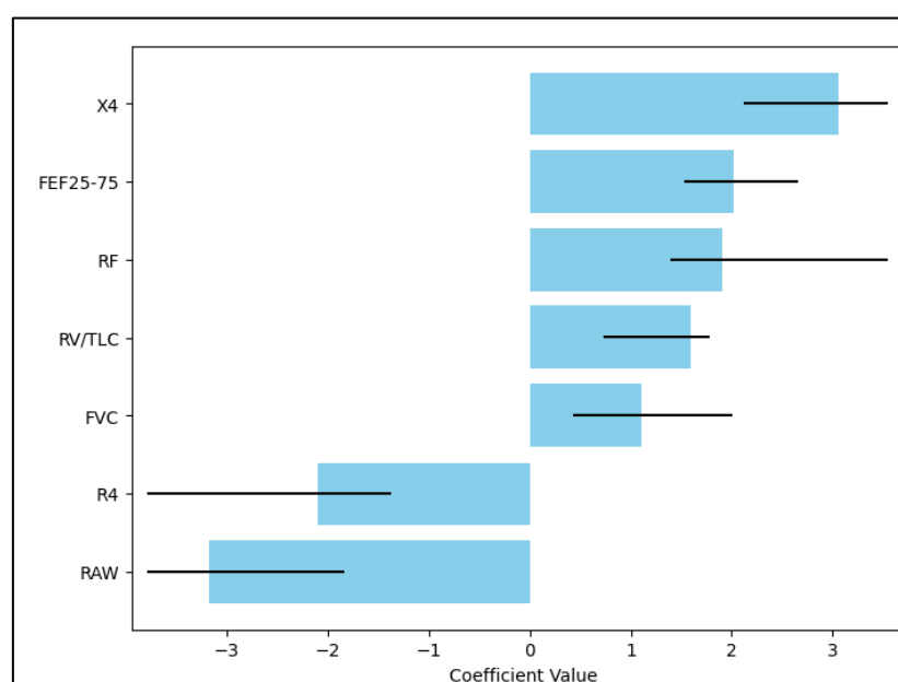
Figure 1. Multivariate regression.
