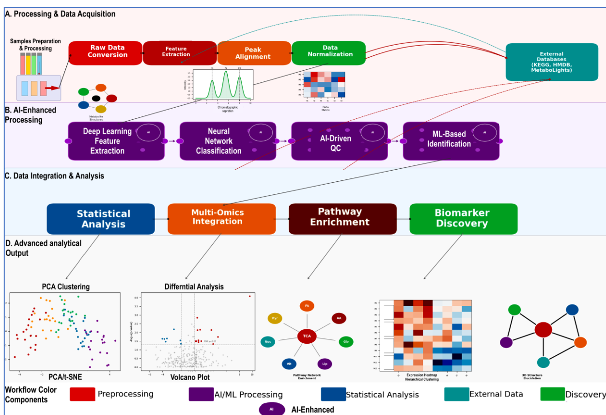
Figure 1. Integrated metabolomics analysis pipeline combining conventional preprocessing with artificial intelligence (AI) and machine learning (ML)–assisted analysis. (A) Preprocessing and data acquisition: Biological samples are extracted and analyzed by liquid chromatography–tandem mass spectrometry (LC–MS/MS). Chromatographic separation generates retention time–resolved ion signals that are converted into structured data matrices ( m/z –retention time features). Subsequent steps include raw data conversion, feature extraction (peak detection), retention time alignment, and normalization. External databases such as HMDB, KEGG, and MetaboLights support metabolite annotation and biological interpretation. (B) AI/ML-assisted processing layer: This layer comprises four interconnected computational modules (purple boxes): representation learning (e.g., deep learning–based feature extraction), classification (e.g., supervised models), data quality control that includes outlier detection and batch correction, and ML-assisted metabolite annotation. These modules enhance robustness and scalability while supporting reproducible downstream analysis. (C) Data integration and analysis: Statistical analysis includes univariate and multivariate approaches with appropriate multiple-testing correction (e.g., false discovery rate [FDR]). Data integration incorporates correlation networks and data fusion across complementary datasets such as transcriptomics or proteomics where available. Pathway enrichment analysis uses curated resources that may include KEGG, Reactome, and WikiPathways to contextualize metabolic alterations. Biomarker discovery applies feature selection and receiver operating characteristic (ROC) analysis with appropriate validation strategies. Red arrows indicate external database queries and iterative annotation refinement. (D) Analytical outputs and disease-relevant interpretation: Outputs include dimensionality reduction such as principal component analysis [PCA] and t-distributed stochastic neighbor embedding [t-SNE] as well as volcano plots for differential abundance analysis (FDR-adjusted p < 0.05 ; |\log_2 \text{fold change}| > 1 ). Pathway network visualization highlights the central role of the tricarboxylic acid (TCA) cycle and its connections to glycolysis, amino acid metabolism, lipid metabolism, nucleotide metabolism, and cofactor/vitamin pathways. Additional outputs include hierarchical clustering heatmaps and molecular structure annotation or elucidation that are supported by spectral evidence. AI/ML-assisted components improve analytical scalability and support reproducible identification of disease-associated metabolic signatures while maintaining rigorous statistical control.
