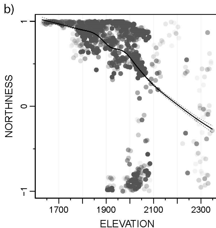
Figure 3. (a) Radial histogram indicating the number of Papaver occidentale individuals according to the slope aspect. The small surrounding ticks indicate single individuals and the black solid line gives a smooth approximation, calculated with a GAM. (b) Northness (N-S slope aspect, values from -1 : south to 1 : north) as a function of elevation (meters), for all P. occidentale individuals in the studied area (grey dots). The black line shows a smooth approximation of the mean (GAM fit, with a 95% confidence interval).
