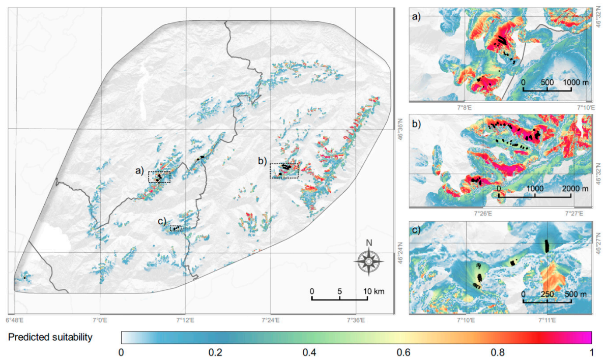
Figure 4. Modelled current habitat suitability of Papaver occidentale in the Western Swiss Prealps. White areas are less suitable, red and purple are the most suitable. Three areas are zoomed on the right panel (a, Vanil Noir region; b, Spillgerte region; c, Gummfluh region). The black dots indicate the locations of P. occidentale (presences).
