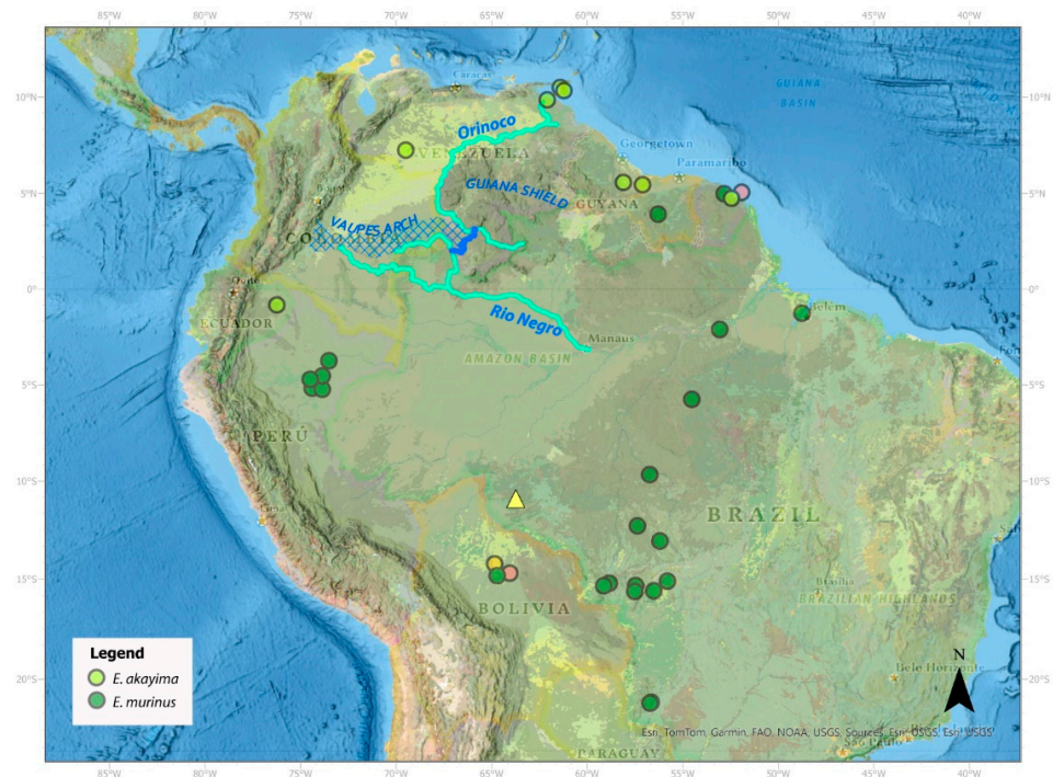
Figure 5. Distribution of E. akayima and E. murinus samples in this study. The light-yellow dot represents E. notaeus of the Beni ecotype (formerly E. beniensis ). The orange dots represent E. notaeus of the Dark Spotted Anaconda ecotypes (formerly E. deschauenseei ). Notice the substantial distance between the mouth of the Amazon where the Dark Spotted Anaconda general distribution is and one of our samples found in the Bolivian Beni. The yellow triangle shows the location of a recent Yellow Anaconda reported in Rondonia, Brazil [94]. The Casiquiare river is presented in dark blue, connecting the Orinoco river (turquoise) with the Rio Negro (turquoise), which is a tributary of the Amazon. The Vaupes arch indicates where waters from the north and the south were divided in geological time.
