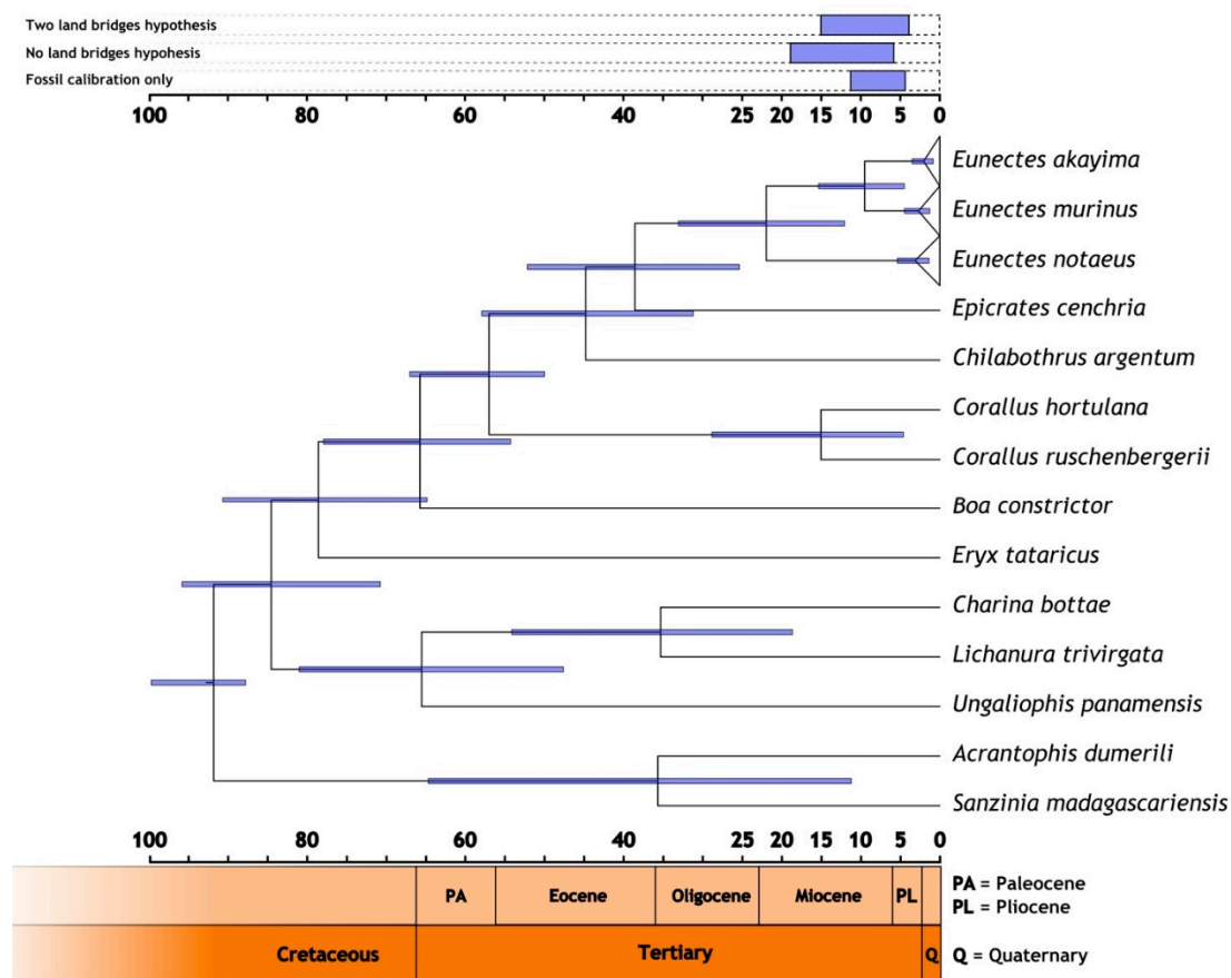
Figure 4. Calibrated species tree depicting inferred lineage splits, assuming the scenario of one land bridge. Node bars on the tree represent the 95% highest posterior density (HPD95%) divergence interval of each node. Legend at the top shows the split of the E. akayima and E. murinus under the three other scenarios that we tested for.
