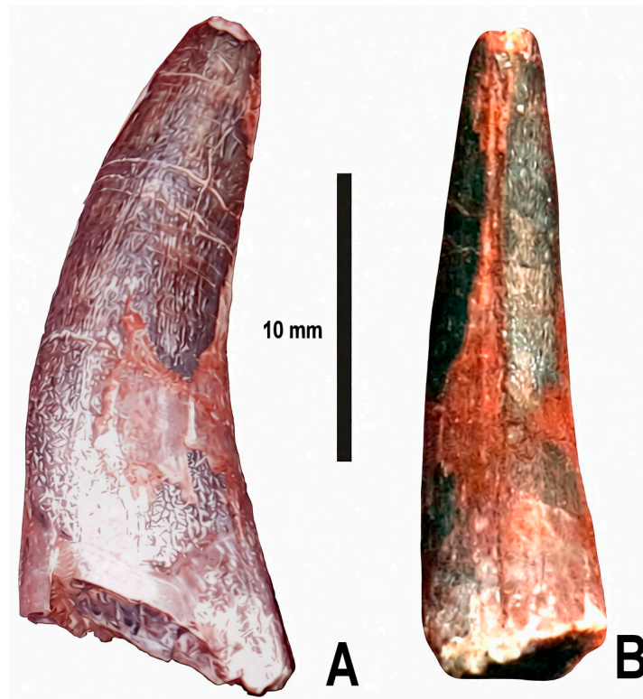
Figure 4. Morphotype B, worn tooth (PRC 465): (A) labial view; (B) distal view. Enamel wrinkling is still visible but serrations have become indistinct.
