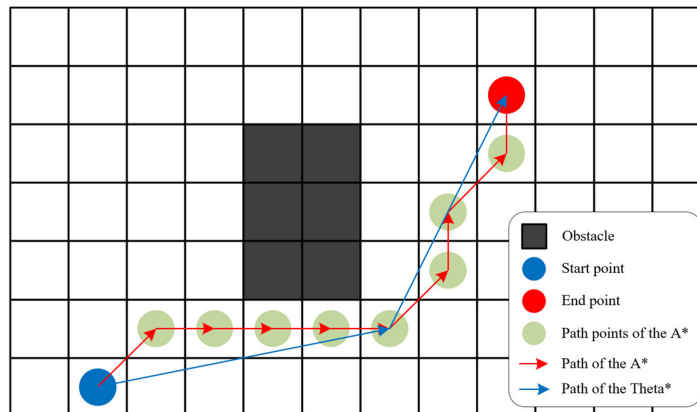
Figure 2. Optimization of the Theta* algorithm for the A* algorithm.
