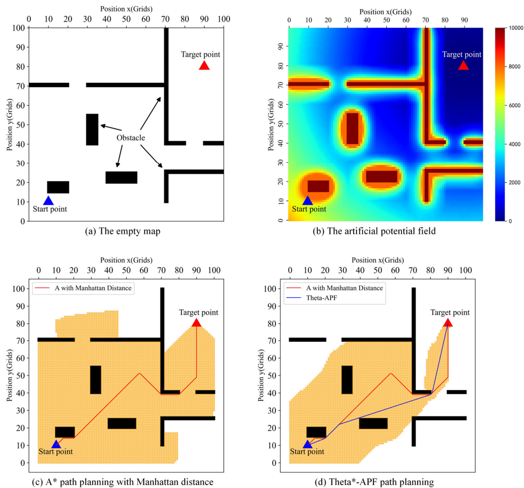
Figure 8. Simulation of Theta*-APF algorithm path planning.
