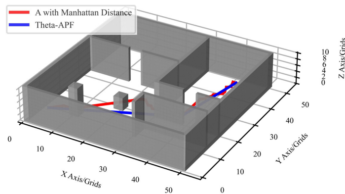
Figure 11. Path planning in a 3D environment.
