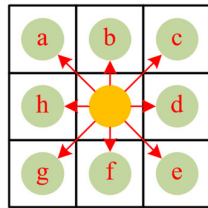
Figure 1. Traditional A* algorithm with 8-neighborhood search.
