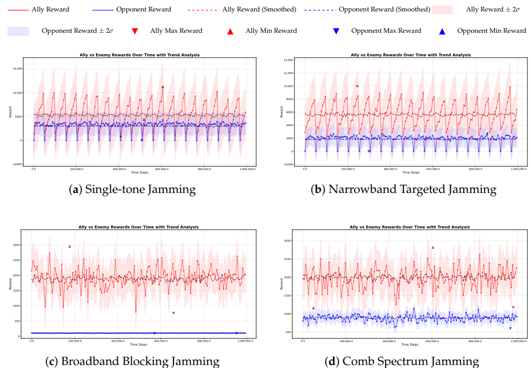
Figure 6. Ablation study on individual jamming types. Rewards of ally (red) and opponent (blue) are shown with smoothed curves (dashed) and variability bands ( \pm 2\sigma ). Takeaway: broadband blocking generally imposes the strongest degradation in ally reward among single-type jamming baselines, while single-tone jamming shows comparatively weaker overall impact in our setting.
