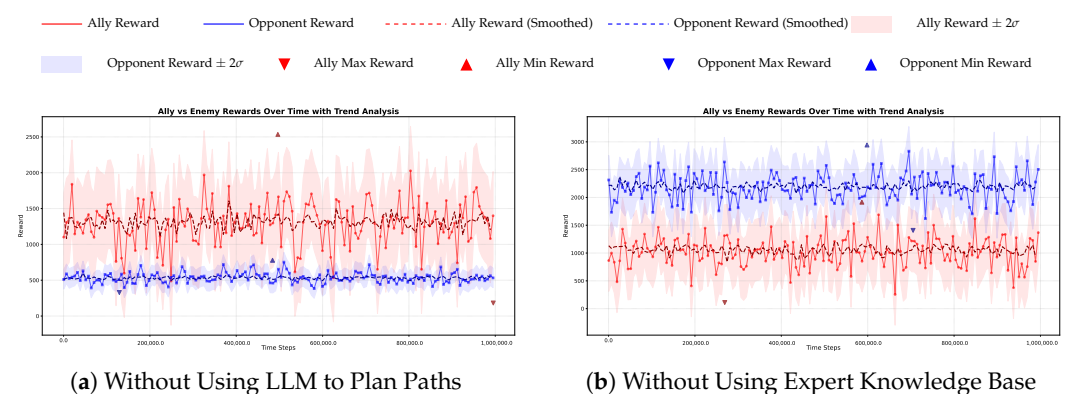
Figure 7. Ablation Study on the Contribution of LLM-Based Path Planning and Expert Knowledge Base Anti-Interference. The red and blue curves represent the rewards obtained by the ally and opponent sides in the game, respectively.
