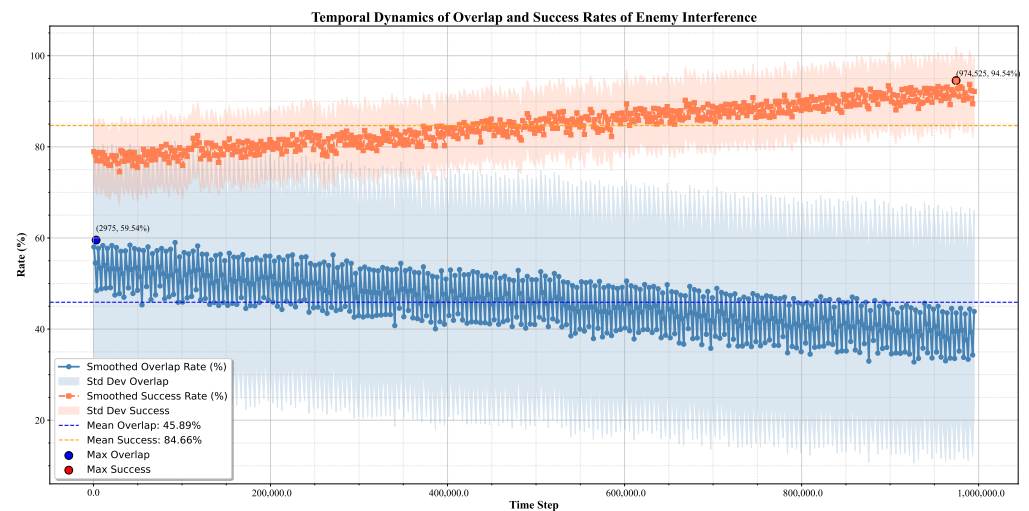
Figure 5. Evolution of frequency overlap and jamming success rate. Curves are smoothed by a moving average with sparse sampling; error bars indicate standard deviation. Takeaway: overlap gradually decreases while the jamming success rate increases, consistent with the opponent switching to broader-band or comb-spectrum strategies in later stages.
