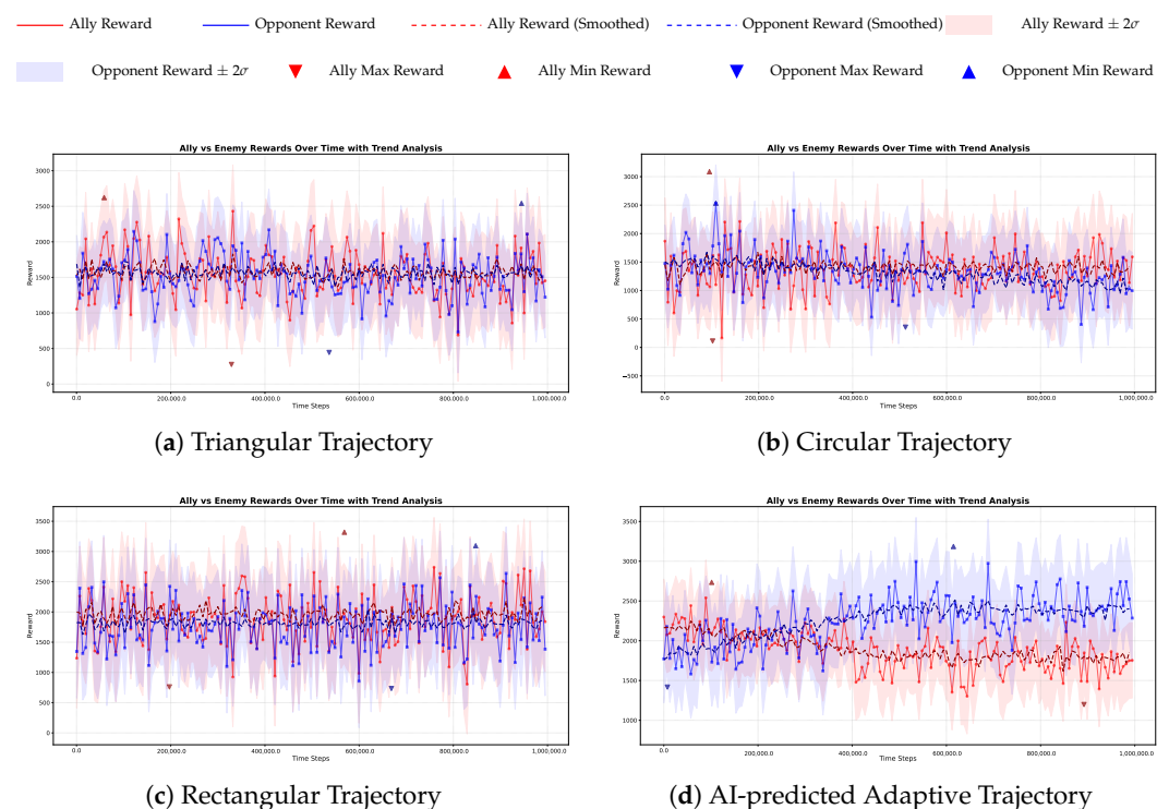
Figure 3. Reward trends under different opponent trajectories. Solid lines show raw rewards and dashed lines show smoothed rewards; shaded regions indicate \pm 2\sigma . Takeaway: compared with fixed geometric trajectories, the LLM-adaptive trajectory tends to yield higher opponent rewards (i.e., stronger adversarial pressure as measured in UAV-FPG under Equation (6)), improving stress-testing of ally policies within the proposed environment.
