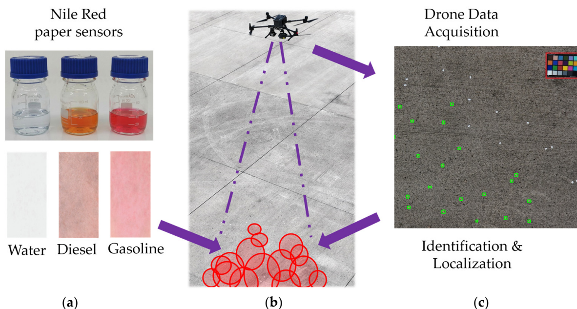
Figure 1. Graphical abstract of the Passive Smart Dust concept. (a) Colorimetric paper-based test strips with Nile red embedded in a polymer respond specifically to different liquid fuels. (b) The test strips were deployed in the field, and their colorimetric response was recorded by a UAV at a 20-m altitude. (c) Potential contamination sites were identified and geolocated using a custom image processing algorithm.
