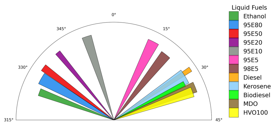
Figure 5. Hue distribution of Nile red test papers after exposure to different liquid fuels under laboratory conditions. Hue values are expressed in degrees, with the angular position indicating the mean hue of each fuel type. The thickness of each sector represents the spread (variability) of the recorded values across replicates. Figures and a table with more solvents are shown in the supplement (Figures S5 and S6).
