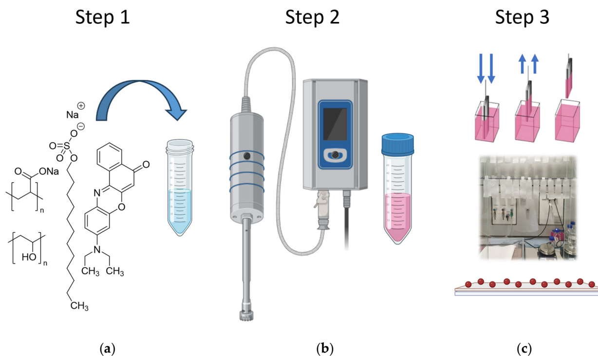
Figure 3. Production steps for sensor test paper manufacturing. (a) All components were added gradually under continuous stirring and held at 60 °C for 30 min. (b) Ultrasonic treatment was applied to ensure homogeneous distribution and to disperse the dye solids. (c) Pretreated cellulose strips were dip-coated in the emulsion for 20 s and dried overnight under ambient conditions by suspension in a fume hood. Created with BioRender.com.
