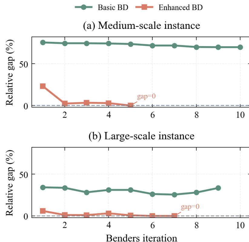
Figure 2. Early-stage BD Gap changes under different algorithms.
