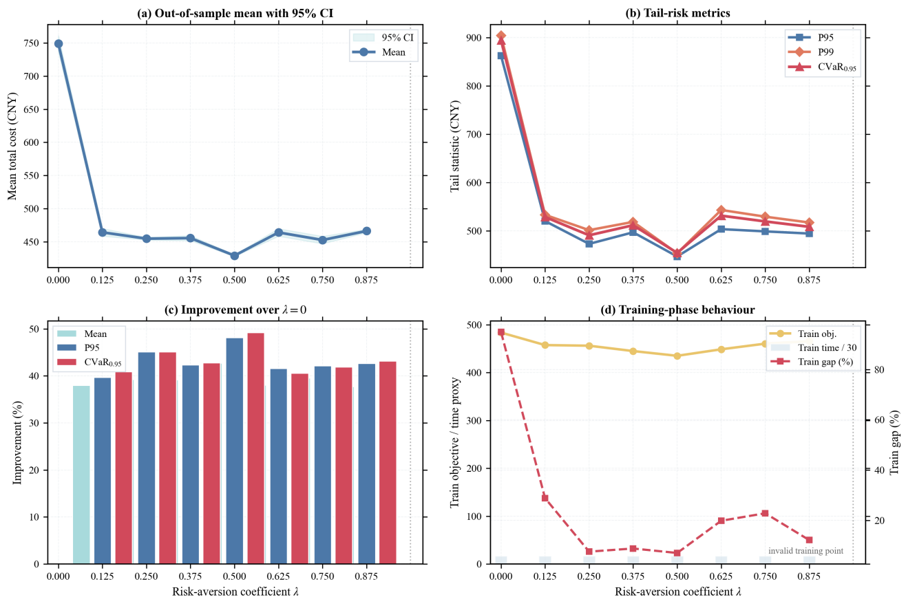
Figure 7. Sensitivity analysis of the risk preference coefficient.
