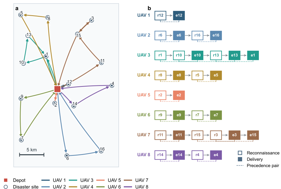
Figure 4. Optimized UAV scheduling solution: (a) spatial flight paths; (b) reconnaissance–delivery task chains.
