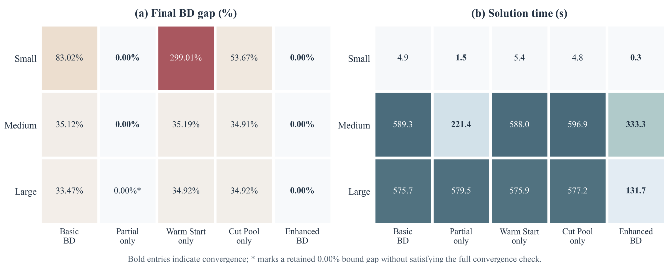
Figure 3. Cross-scale ablation results of Benders acceleration strategies. In panel (a), darker red indicates a larger final BD gap; in panel (b), darker blue indicates a longer solution time. Bold entries indicate convergence.
