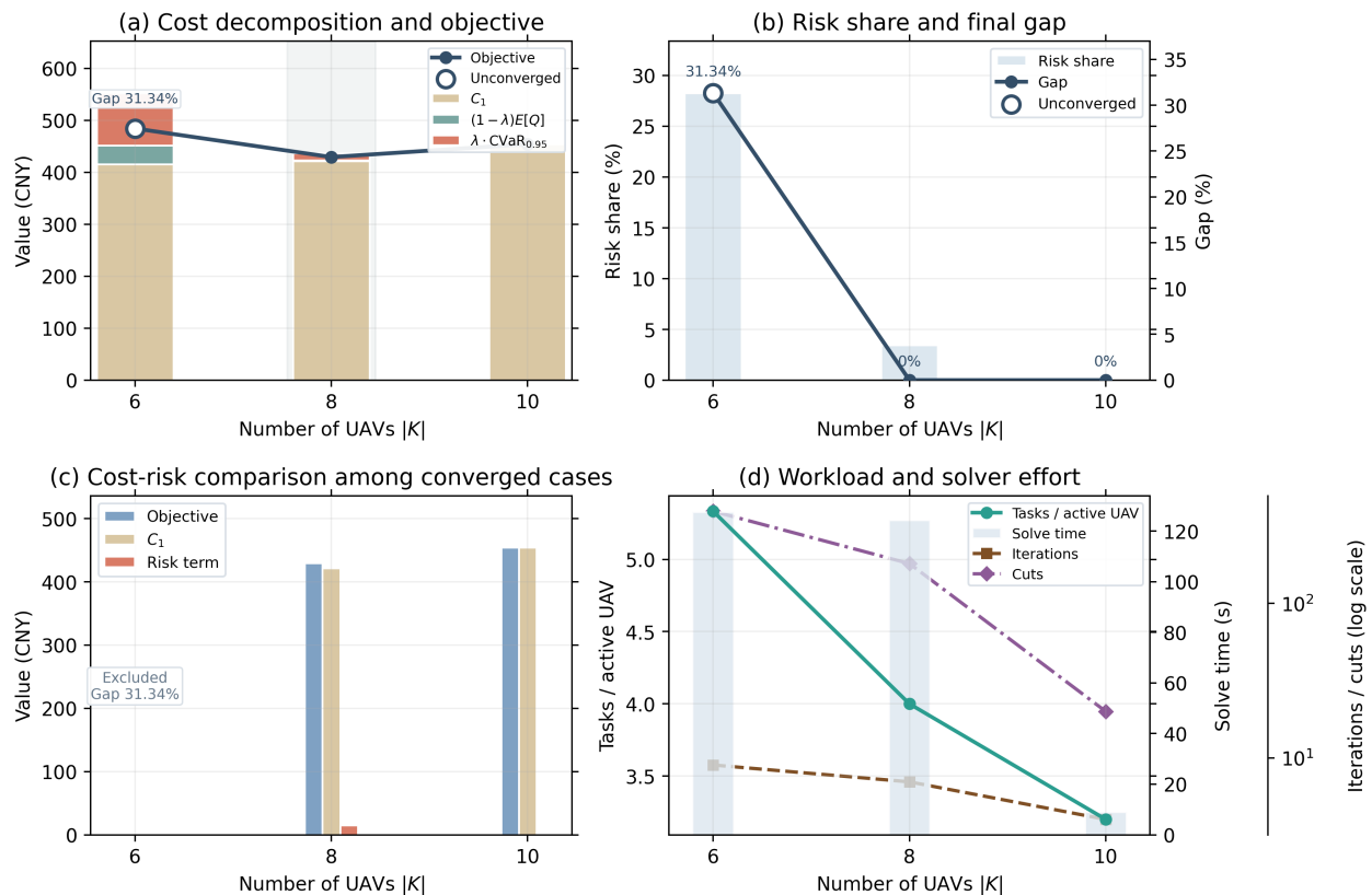
Figure 6. Sensitivity analysis of fleet size.
