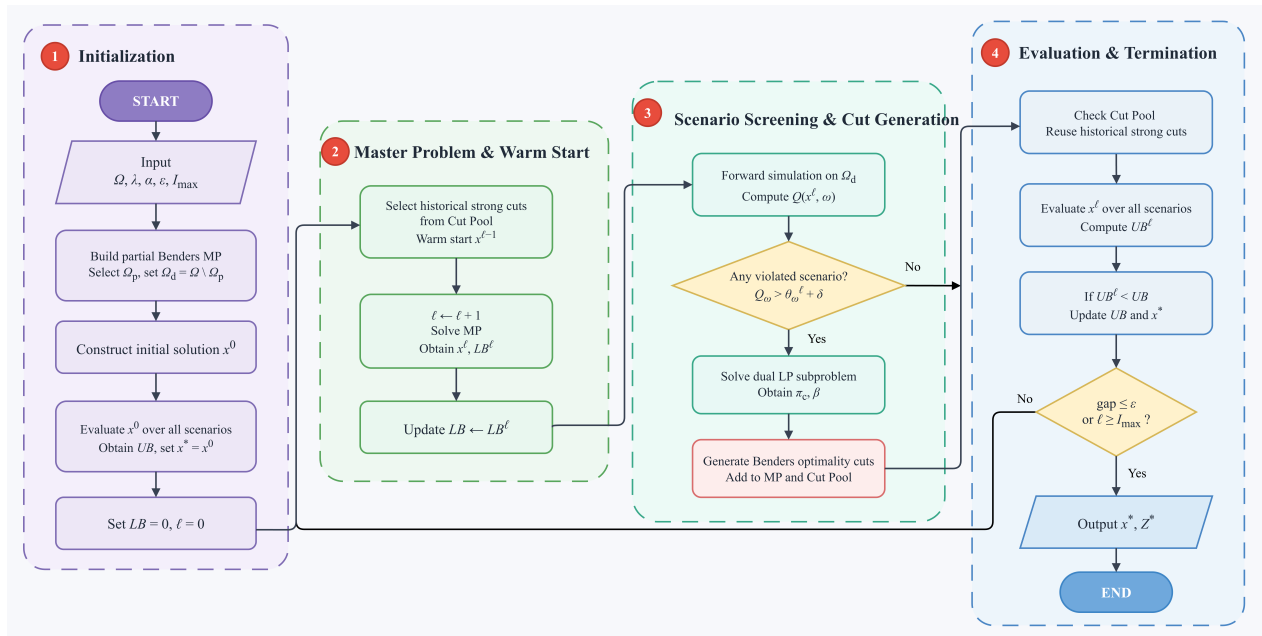
Figure 1. Flowchart of the hybrid Benders decomposition algorithm. The superscript * denotes the incumbent best solution.
