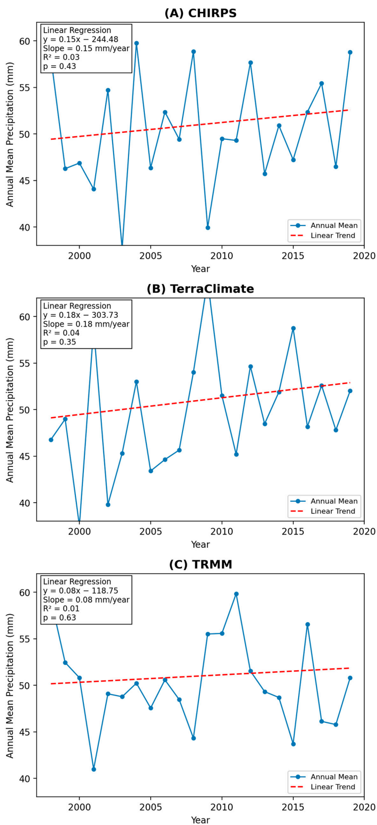
Figure 4. Linear trend analysis of annual mean precipitation derived from (A) CHIRPS, (B) TerraClimate, and (C) TRMM datasets for the period 1998–2019. The regression equation, coefficient of determination ( R^2 ), and p -value are shown in each panel.
