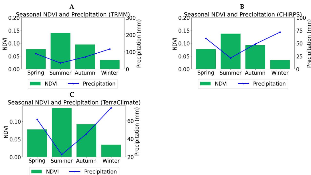
Figure 9. The relationship between seasonal total precipitation (mm) and Landsat NDVI values in the study area ((A): TRMM, (B): CHIRPS, (C): TerraClimate).
