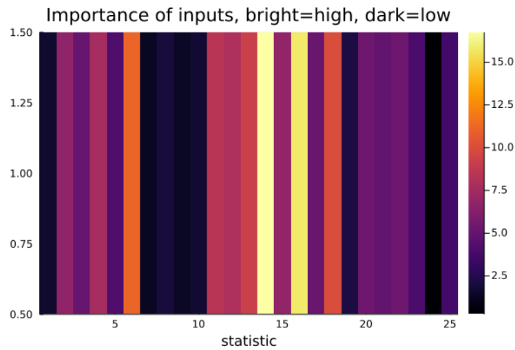
Figure 1. Importance of statistics, jump-diffusion model.
