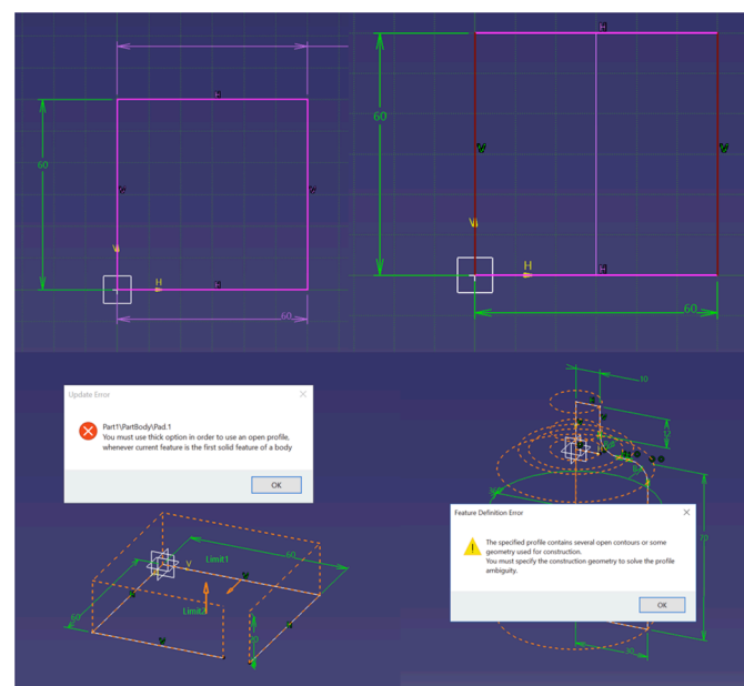
Figure 3. An example of the diagnostic error replication strategy: demonstrating an over-constrained sketch and its resulting topological conflicts to cultivate students’ troubleshooting heuristics.
