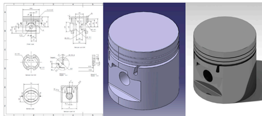
Figure 2. An authentic PBL task: Transitioning from a 2D orthographic drawing to the final 3D parametric model of a complex piston.
