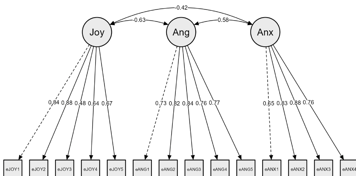
Figure 2. Results of the CFA Model (Split-Half Sample 2).
