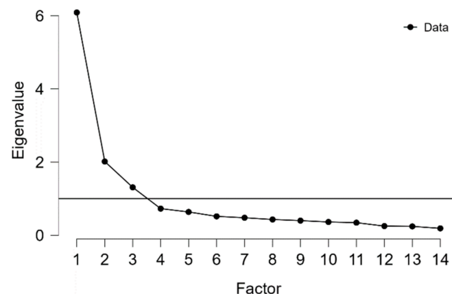
Figure 1. Scree plot of the PES-Home.
