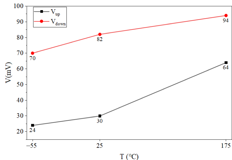
(a) Overshoot voltage and undershoot voltage
