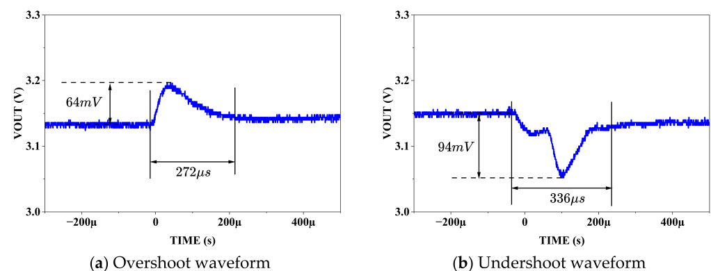
Figure 20. Load transient response test results ( T = 175\text{ }^{\circ}\text{C} ).
