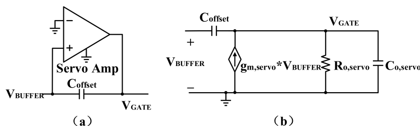
Figure 11. Small-signal model of the servo operational amplifier and offset capacitor. (a) servo operational amplifier; (b) small-signal model.
