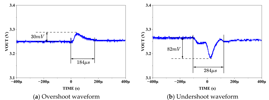
Figure 19. Load transient response test results ( T = 25\text{ }^{\circ}\text{C} ).
