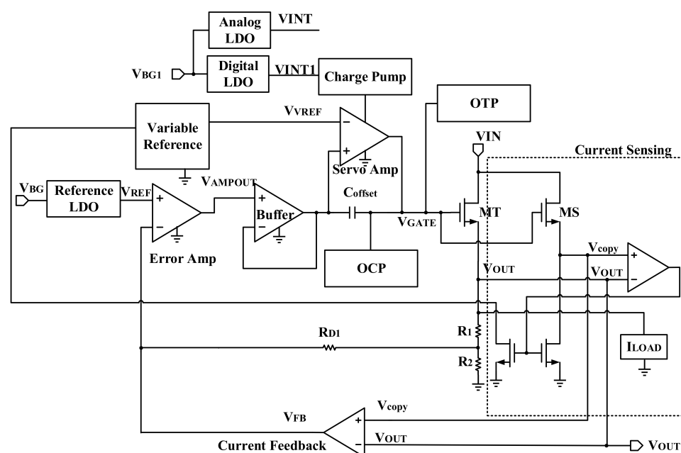
Figure 3. Structure of the LDO circuit.
