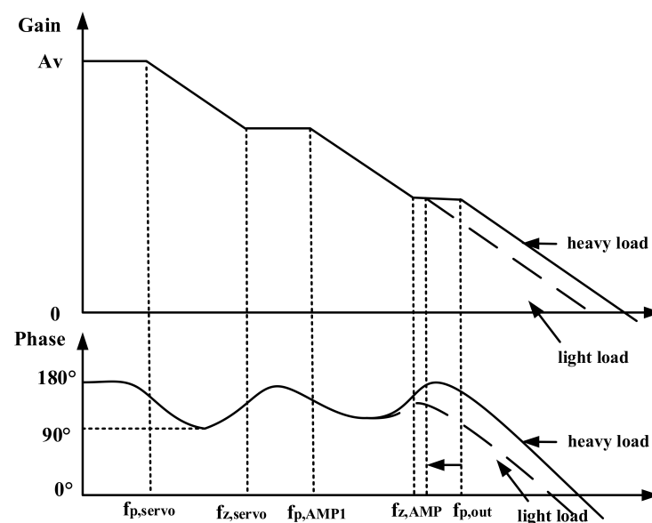
Figure 12. Pole-zero distribution of the LDO loop.
