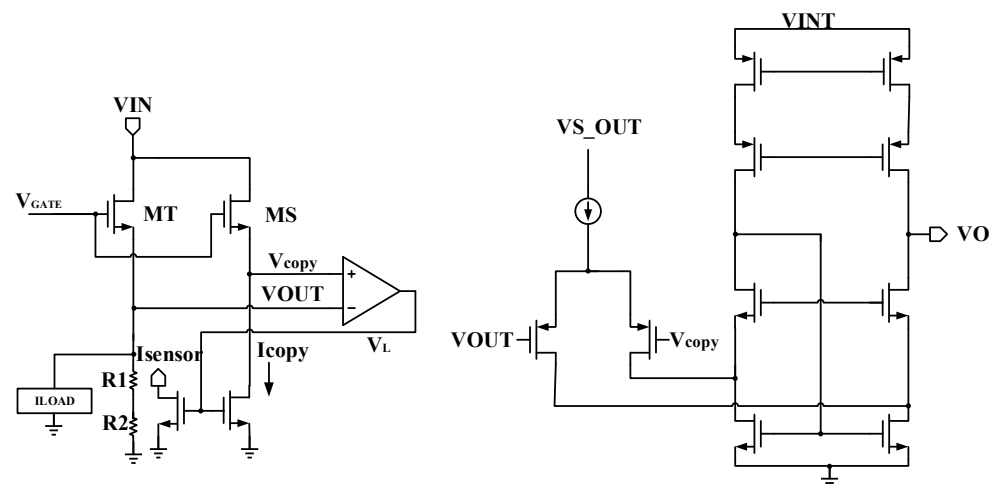
(a) Schematic of the current sensing circuit (b) Schematic of the clamping operational amplifier
