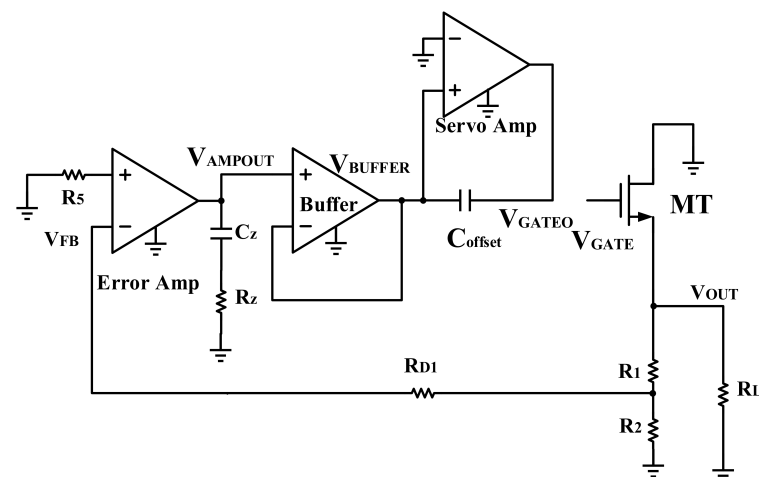
Figure 9. LDO equivalent loop.
