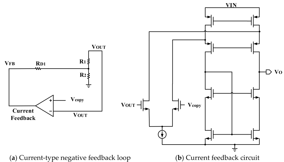
Figure 8. Current feedback circuit diagram.
