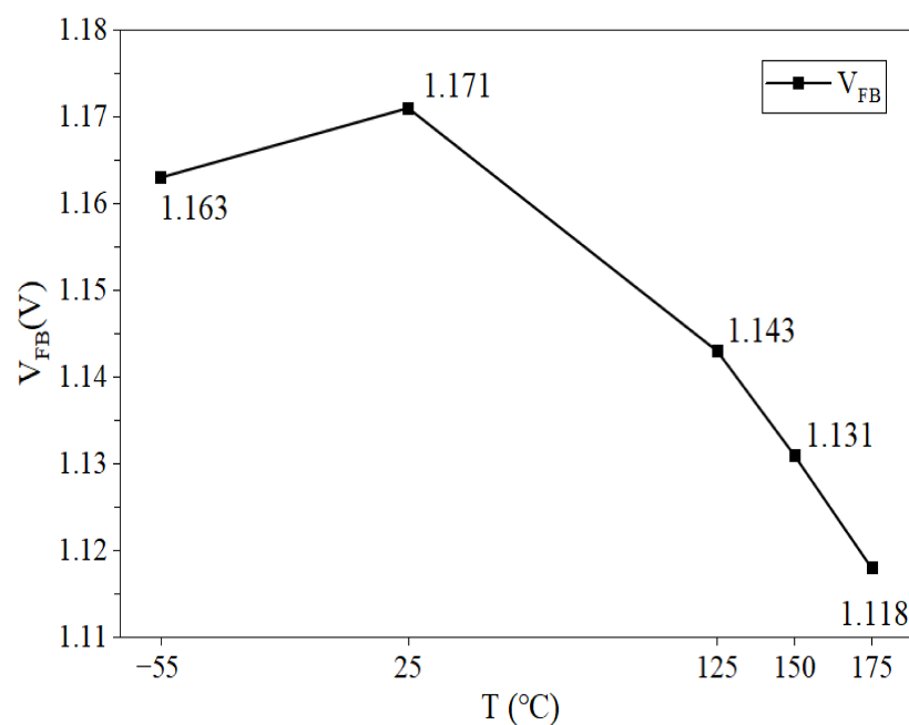
Figure 17. Temperature characteristics of the measured feedback voltage V_{FB} .
