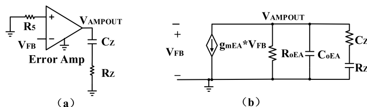
Figure 10. Small-signal model of the error amplifier with compensation capacitor and resistor. (a) error amplifier; (b) Small-signal model of the error amplifier.
