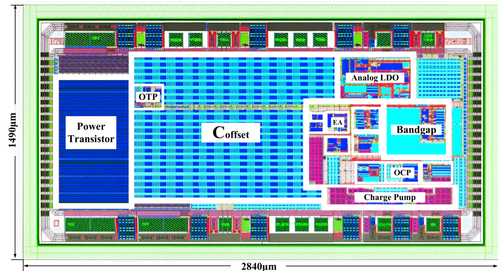
Figure 13. Overall layout.
