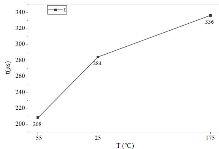
(b) Maximum recovery time
