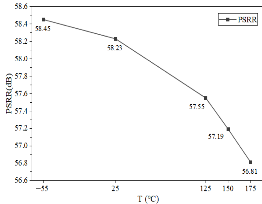
Figure 22. Temperature characteristics of PSRR test results.
