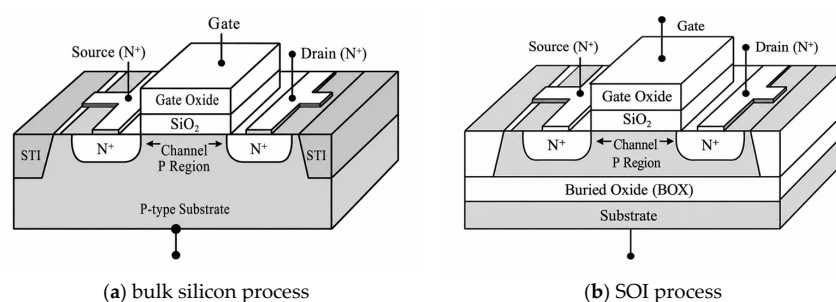
Figure 1. MOSFET structure.
