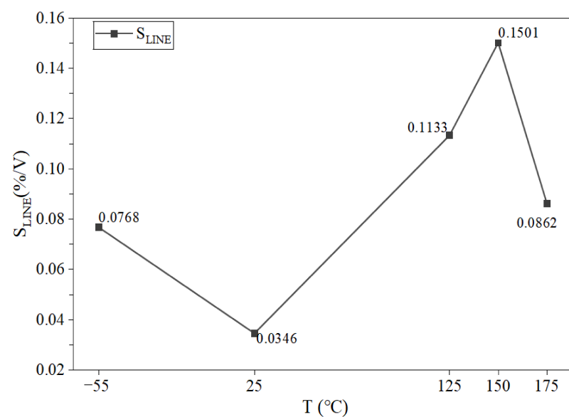
Figure 15. Temperature characteristics of line regulation test results.
