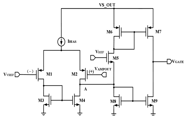
Figure 5. Schematic diagram of the servo operational amplifier.
