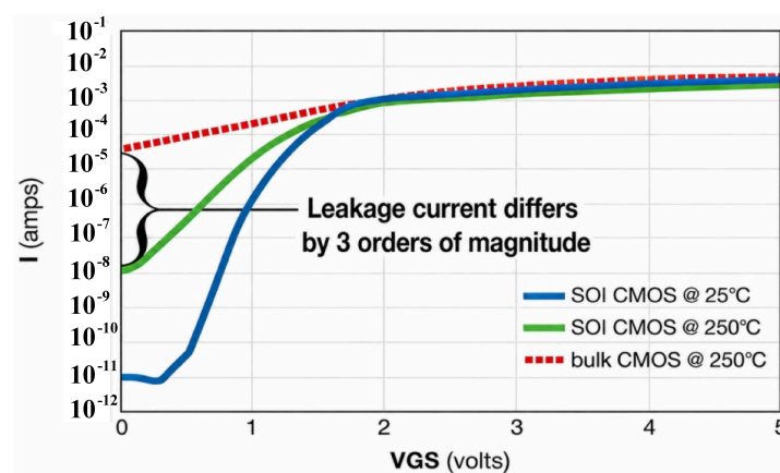
Figure 2. High-temperature leakage behavior of SOI and bulk-silicon devices.
