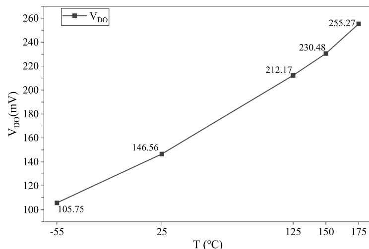
Figure 14. Temperature characteristics of dropout voltage test results.
