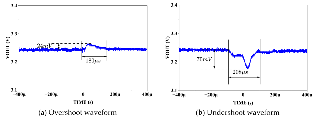
Figure 18. Load transient response test results ( T = -55\text{ }^{\circ}\text{C} ).
