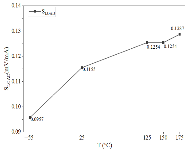
Figure 16. Temperature characteristics of load regulation test results.
