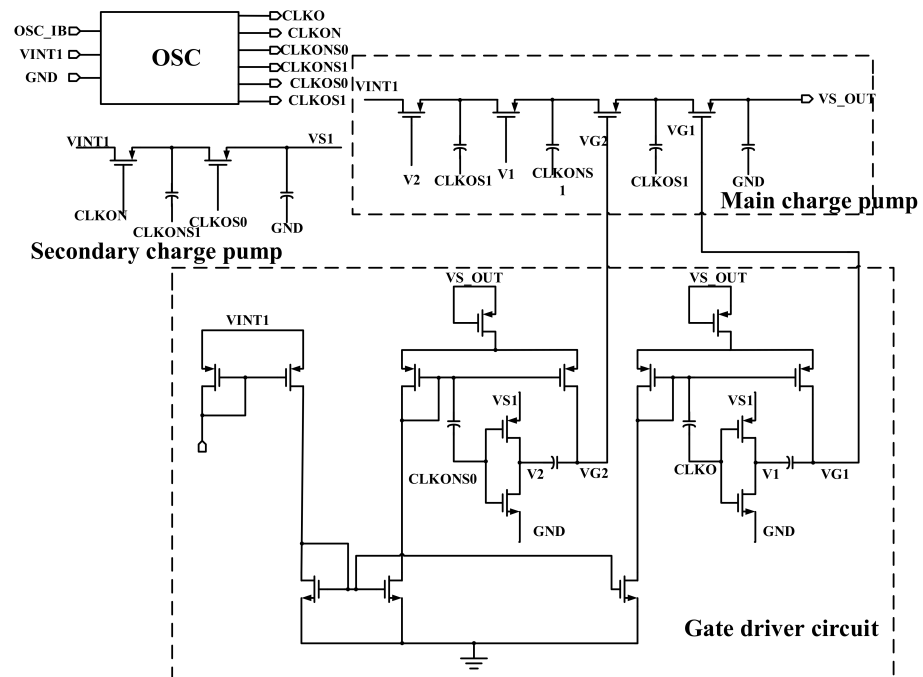
Figure 4. Schematic diagram of the charge pump circuit.
