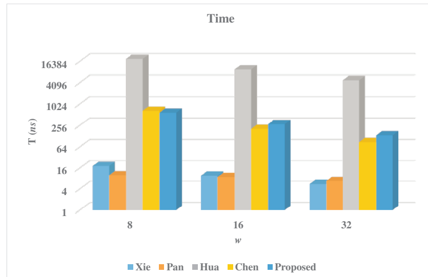
Figure 10. Comparison of time results.
