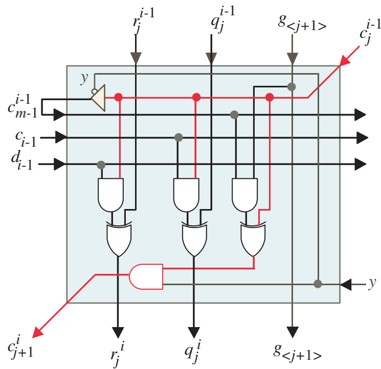
Figure 7. Light blue PE details of SISO two-dimensional systolic array.
