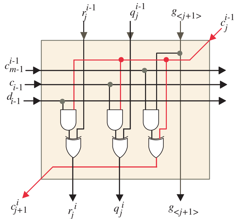
Figure 8. Light Orange PE details of SISO two-dimensional systolic array.
