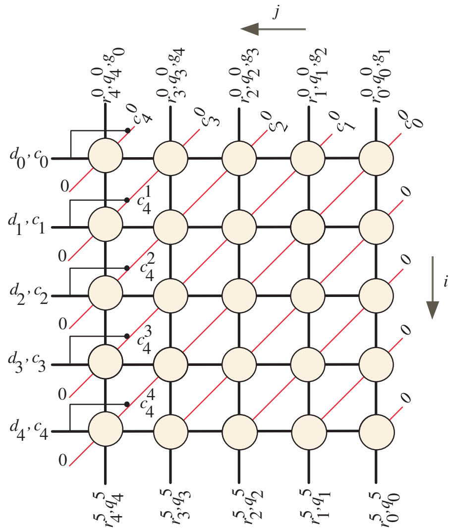
Figure 1. Dependence graph for the combined multiplication-squaring algorithm for m = 5 .
