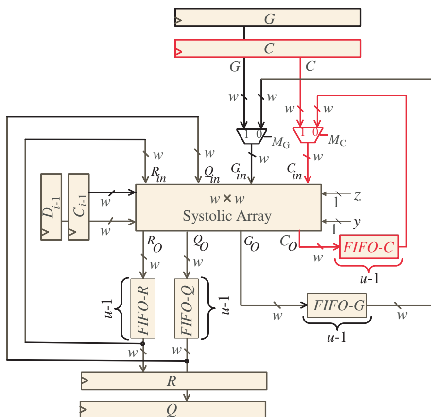
Figure 5. Word-based two-dimensional SISO systolic processor.
