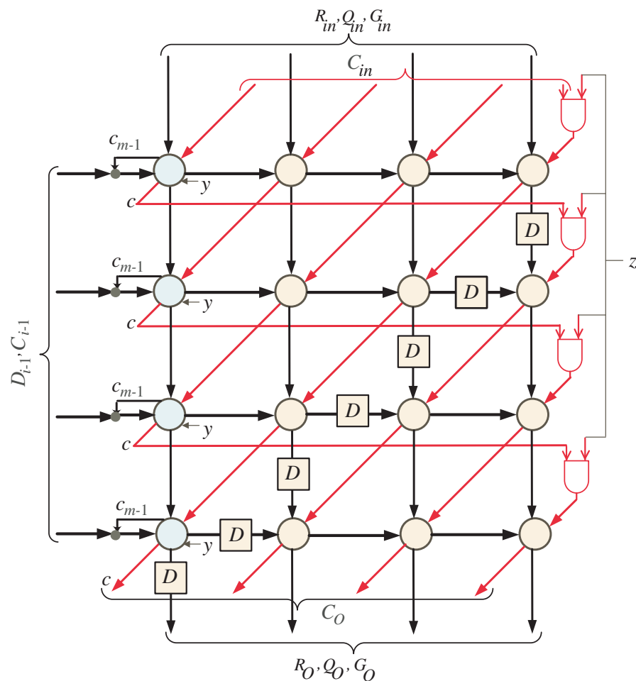
Figure 6. Word-based two-dimensional SISO systolic array.
