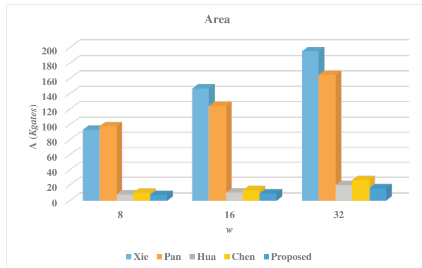
Figure 9. Comparison of area results.
