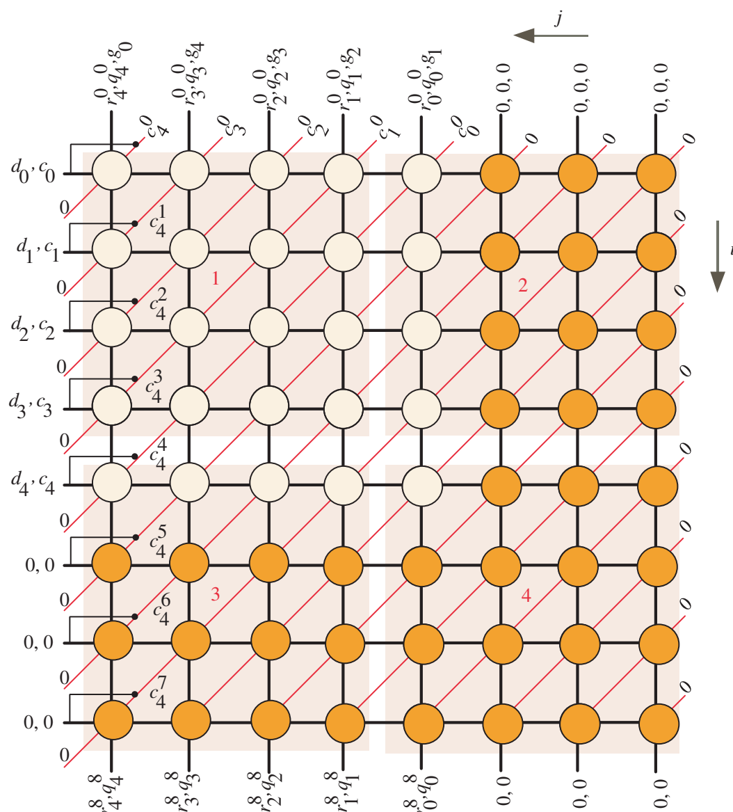
Figure 3. Scheduling time for the case when m = 5 and w = 4 .
