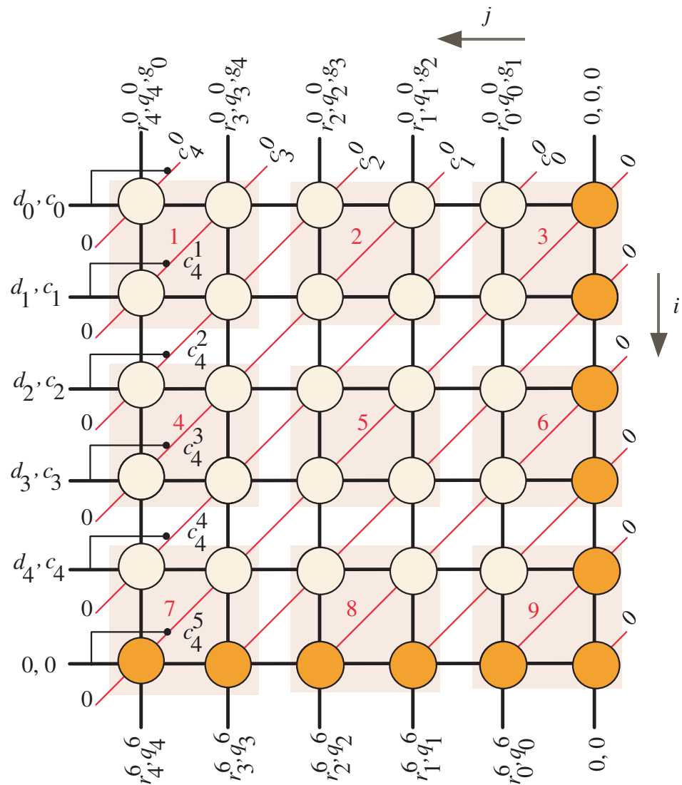
Figure 2. Scheduling time for the case when m = 5 and w = 2 .
