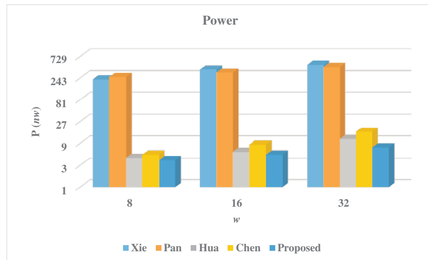
Figure 11. Comparison of consumed power results.
