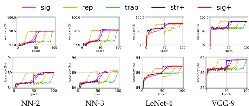
Figure 3. [Shallow model with learning rate warmup.] Accuracy curve over epochs for MNIST (first row), and Fashion-MNIST (second row) by SGD with different learning rate annealings: sigmoid function without warmup (sig), twice-repeated sigmoids (rep), trapezoid with 10%-epoch warmup (trap), staircase with the warmup (str+), and our sigmoid with the warmup (sig+): The per-epoch average of validation accuracy over 10 trials is shown in the y-axis where the range of accuracy is fixed for each data-set. Epoch (0, 1, 2, ..., 100) is shown in the x-axis.
