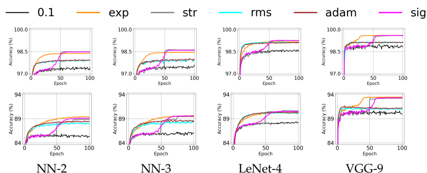
Figure 2. [Shallow model with learning rate decay.] Accuracy curve over epochs for MNIST (first row), and Fashion-MNIST (second row) by SGD with different learning rate annealings: constant learning rate \eta = 0.1 , exponential (exp), staircase (str), RMSprop (rms), Adam (adam), and sigmoid (sig): The per-epoch average of validation accuracy over 10 trials is shown in the y-axis where the range of accuracy is fixed for each data-set. Epoch (0, 1, 2, ..., 100) is shown in the x-axis.
