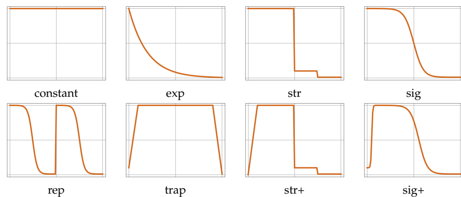
Figure 1. (y-axis) Learning rate over (x-axis) epochs by ( top row ) conventional annealing methods: constant learning rate \eta = 0.1 , exponential function (exp) [55], staircase (str) [40] with \eta = 0.1, 0.01, 0.001 , and sigmoid function (sig), and ( bottom row ) warmup methods: twice-repeated sigmoids (rep), trapezoid with 10%-epoch warmup (trap) [60], staircase with the warmup (str+), and our sigmoid with the warmup (sig+).
