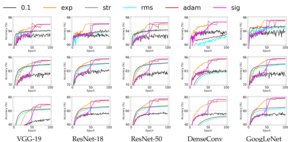
Figure 4. [DNNs with learning rate decay.] Accuracy curve over epochs for SVHN (first row), CIFAR-10 (second row), and CIFAR-100 (third row) by SGD with different learning rate annealings: constant learning rate \eta = 0.1 , exponential (exp), staircase (str), RMSprop (rms), Adam (adam), and sigmoid (sig): Per-epoch average of validation accuracy over 10 trials is shown in the y-axis where the range of accuracy is fixed for each data-set. Epoch (0, 1, 2, ..., 100) is shown in the x-axis.
