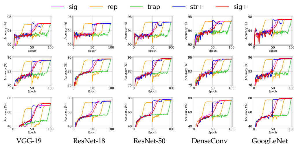
Figure 5. [DNNs with learning rate warmup.] Accuracy curve over epochs for SVHN (first row), CIFAR-10 (second row), and CIFAR-100 (third row) by SGD with different learning rate annealings: sigmoid function without warmup (sig), twice-repeated sigmoids (rep), trapezoid with 10%-epoch warmup (trap), staircase with the warmup (str+), and our sigmoid with the warmup (sig+): Per-epoch average of validation accuracy over 10 trials is shown in the y-axis where the range of accuracy is fixed for each data-set. Epoch (0, 1, 2, ..., 100) is shown in the x-axis.
