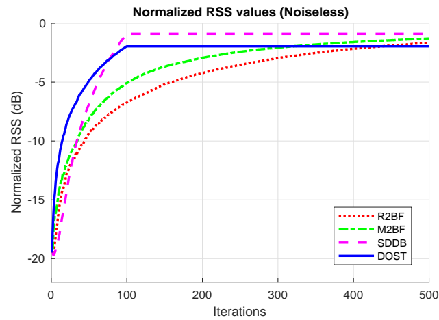
Figure 2. Evolution of the distributed beamforming gain in a noiseless setting for N = 100 nodes.
