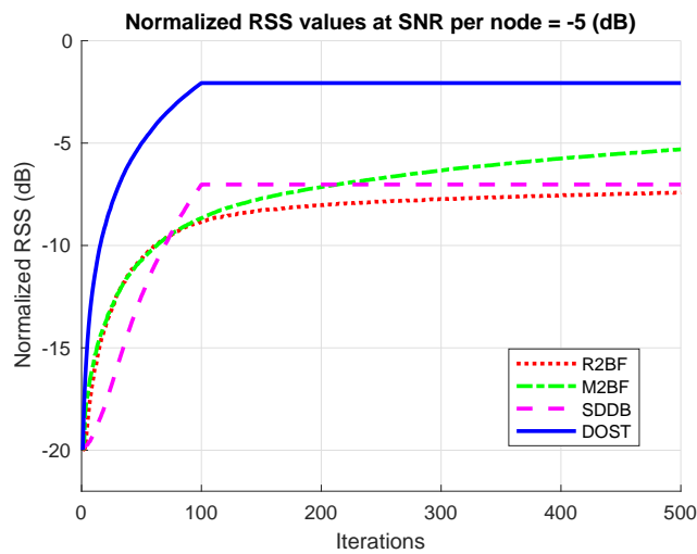
Figure 3. Evolution of the distributed beamforming gain for N = 100 nodes at SNR per node -5 dB.
