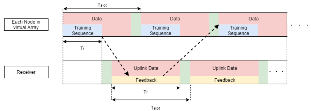
Figure 8. DBS frame structure with a slow feedback link.
