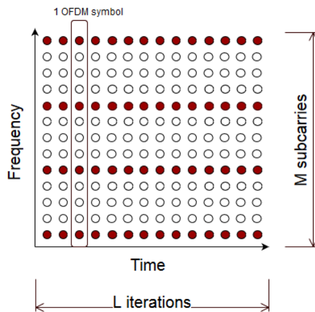
Figure 5. Proposed comb type pilot arrangement for channel estimation over OFDM grid.
