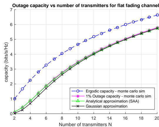
Figure 9. Ergodic capacity and 1% outage rates (b/s/Hz) versus number of nodes for narrowband flat fading channel at SNR = −5 dB.
