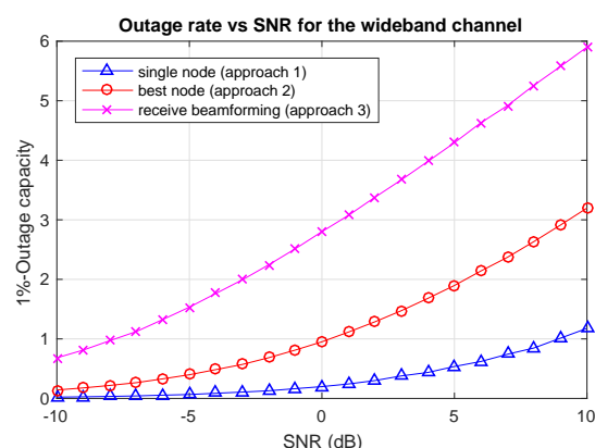
Figure 11. 1% outage rates vs. per node SNR for wideband channels using 10% of the 20 MHz uplink bandwidth with single node, best node and ideal receive beamforming with using N = 10 nodes.
