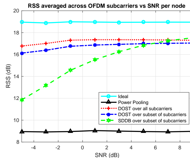
Figure 7. Received signal strength averaged over OFDM subcarriers vs. SNR per node for N = 10 nodes.
