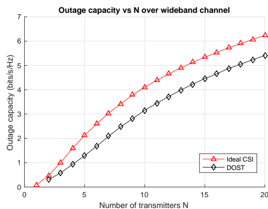
Figure 10. 1% outage rates (b/s/Hz) vs N for wideband channel at average SNR = −5 dB.
