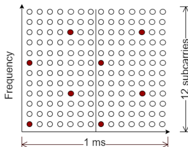
Figure 6. Standard 2D-grid type pilot placement is not well matched to a DBS OFDM downlink.
