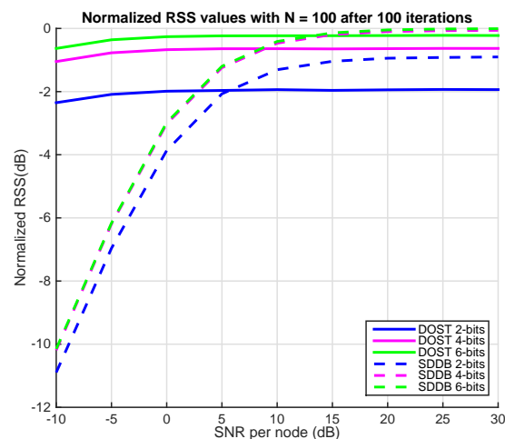
Figure 4. Beamforming gains for SDDB and DOST for different number of feedback bits normalized to the optimal beamforming gain, N .
