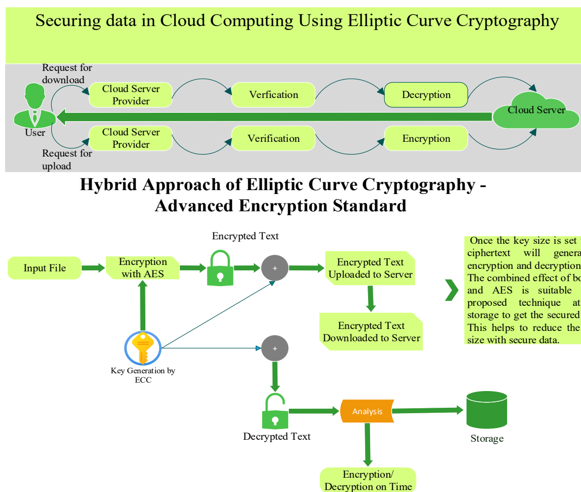
Figure 5. Representation of ECC and AES algorithm.
