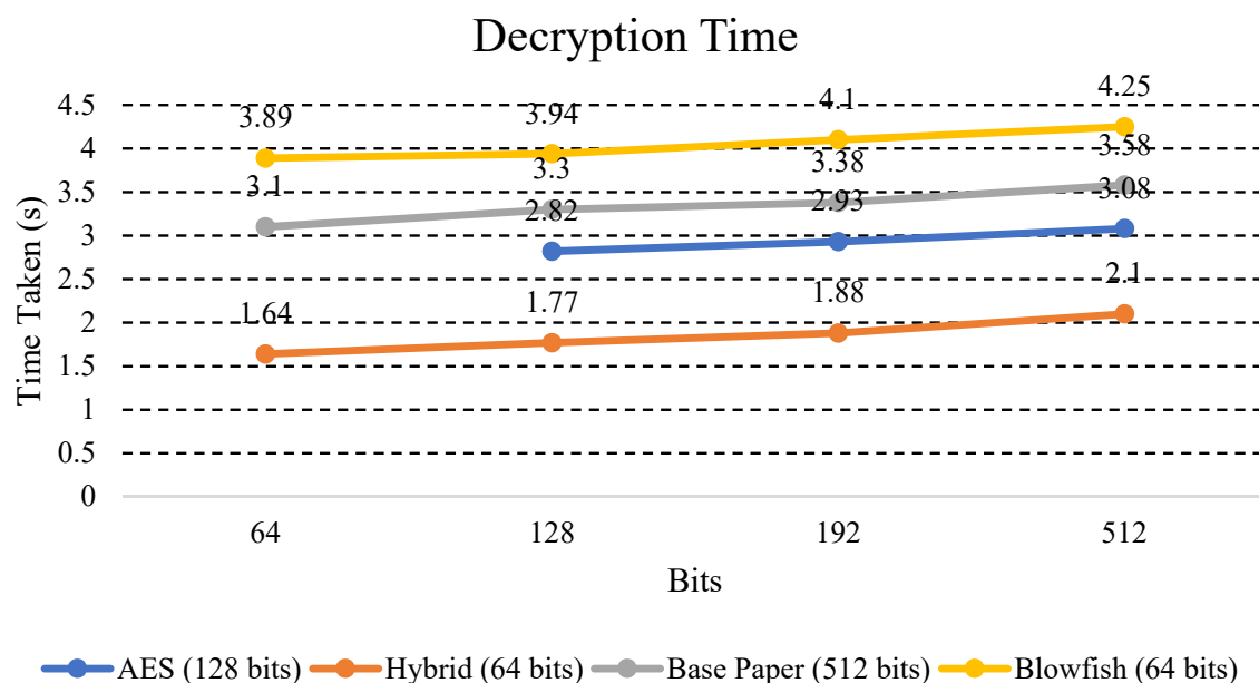
Figure 10. Comparison graph for decryption time in hybrid and other existing algorithms using different key sizes.
