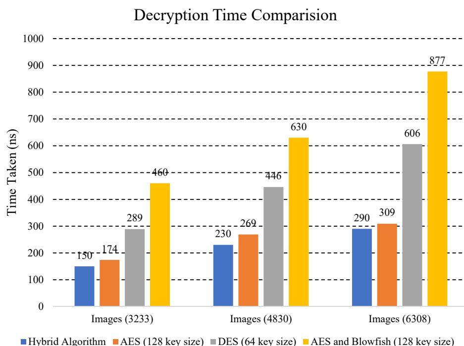
Figure 8. Decryption time comparison of different algorithms.
