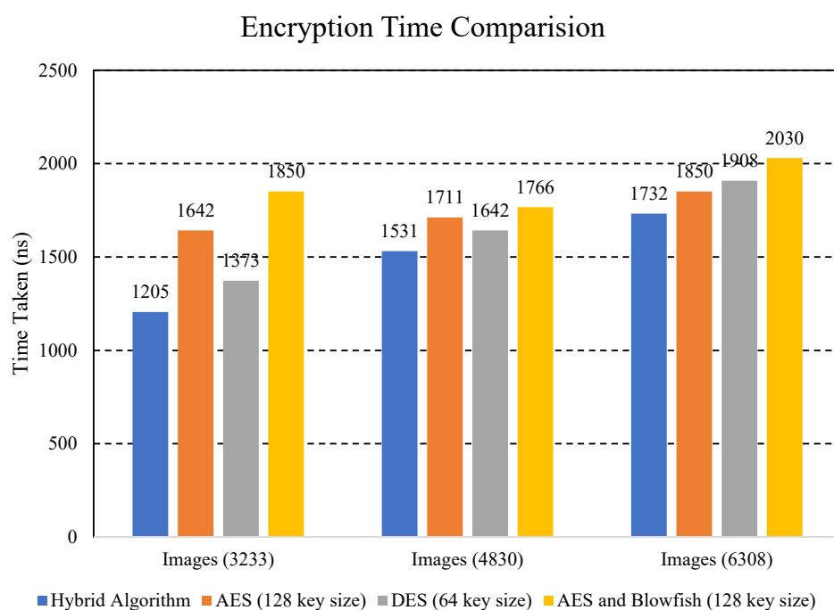
Figure 7. Encryption time comparison of different algorithms.
