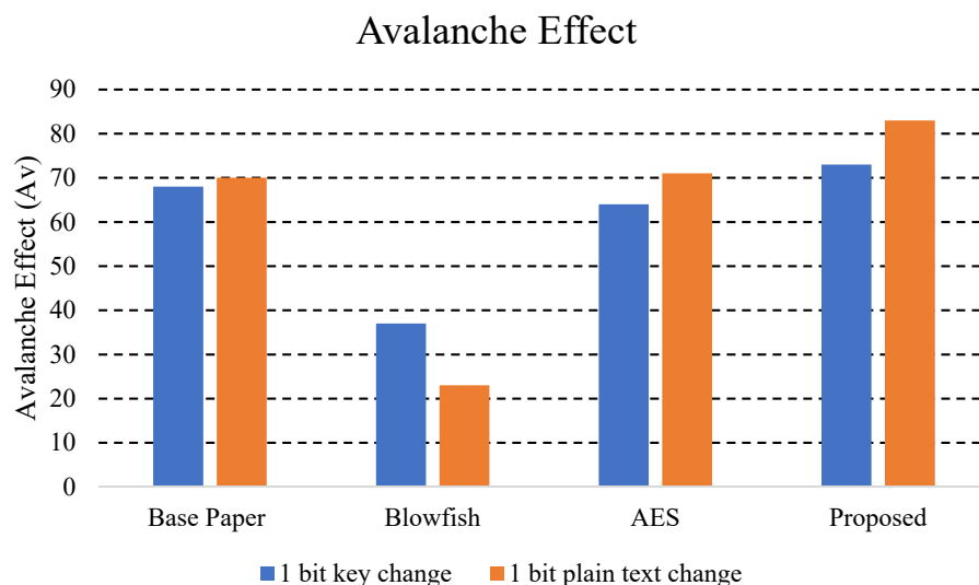
Figure 11. Comparison of Avalanche effect with other schemes.
