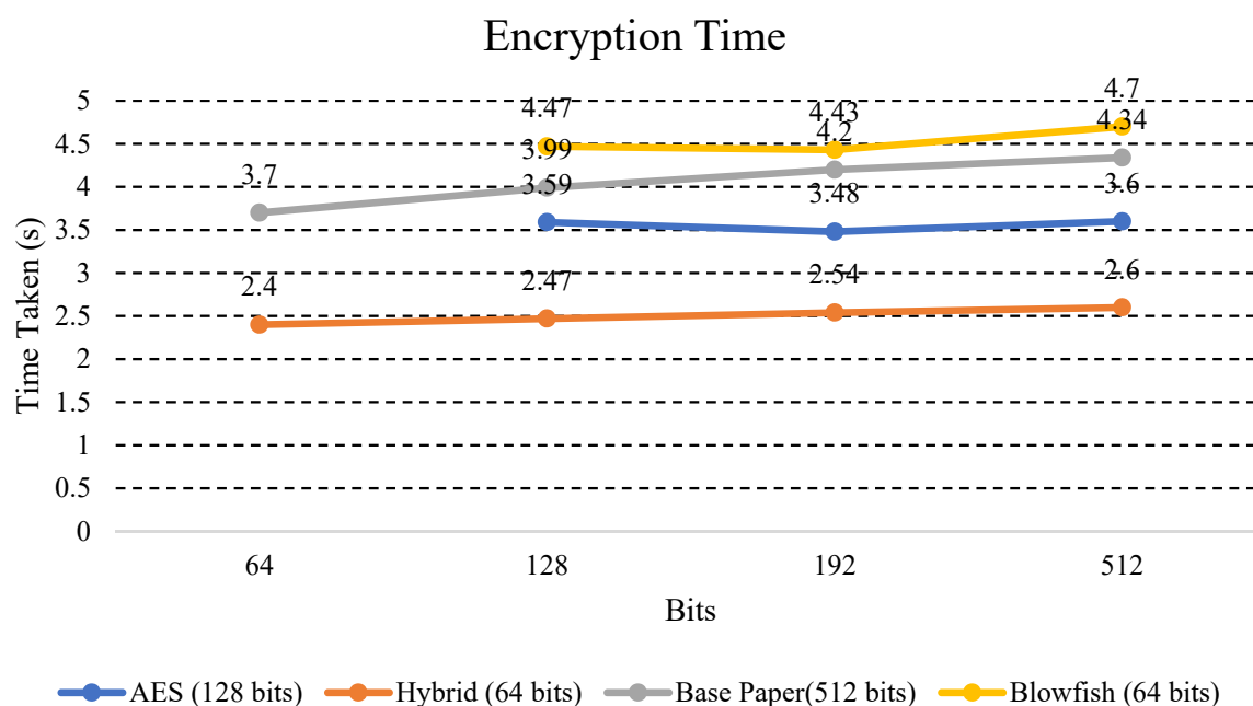
Figure 9. Comparison graph for encryption time in hybrid and other existing algorithms using different key sizes.
