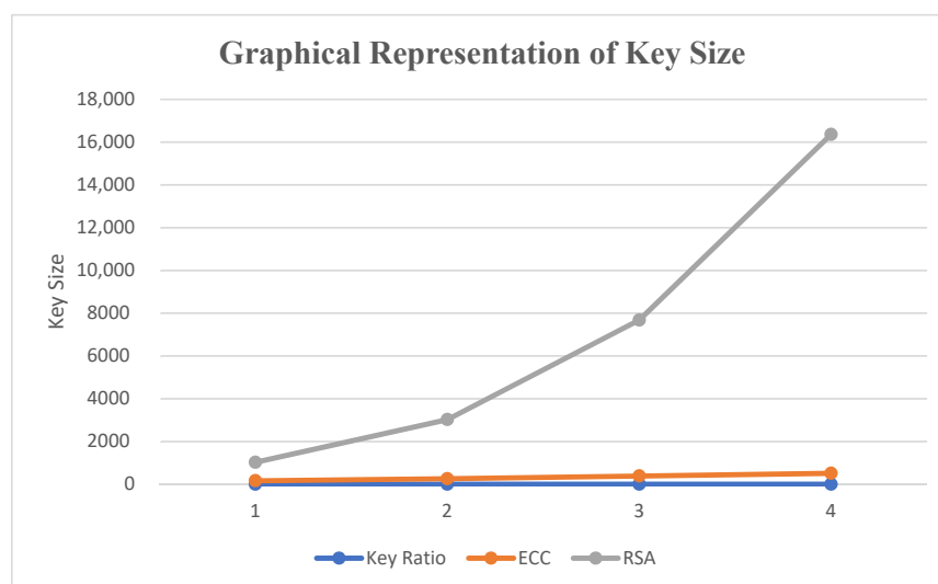
Figure 6. Graphical representation of key sizes.
