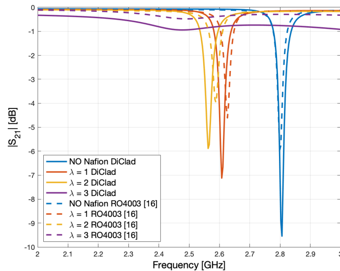
Figure 3. Evaluation of the substrate impact on the sensitivity of a humidity chipless sensor in low-humidity conditions. Simulation of a 2.8 GHz ELC resonator covered by Nafion 117 on DiClad ( \epsilon_r = 2.33 ) and Rogers RO4003 ( \epsilon_r = 3.28 ) [16] laminates.
