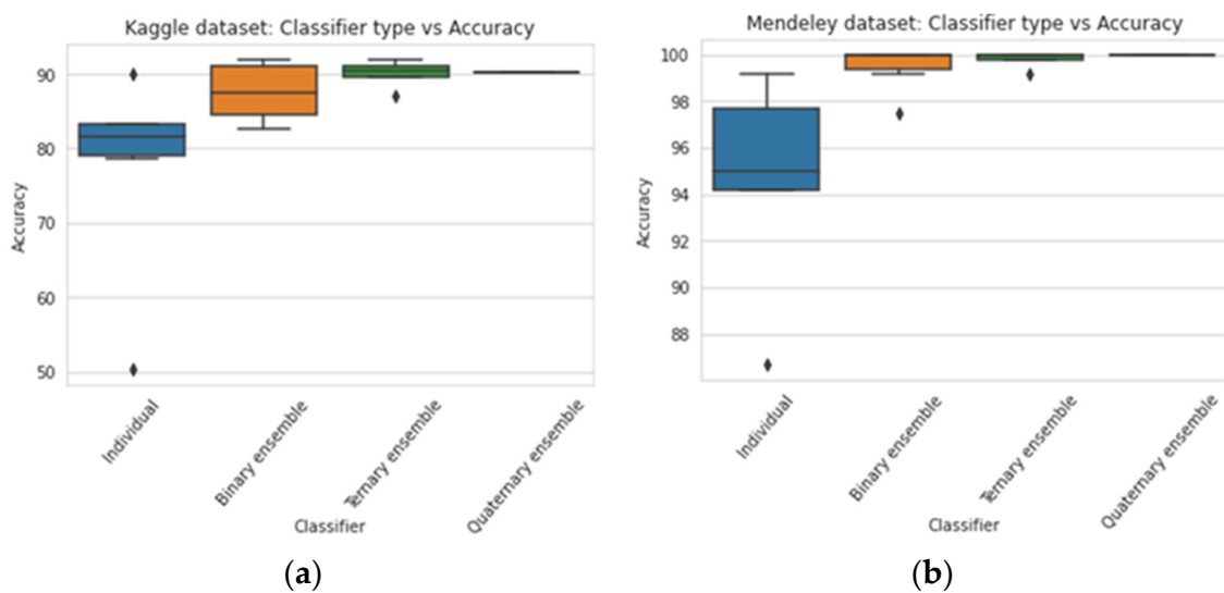
Figure 11. Range of accuracies of various classification models for (a) Kaggle and (b) Mendeley.
