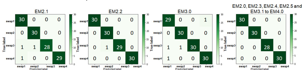
Figure 10. Confusion matrices of the ensemble classifiers for the Mendeley rice N deficiency dataset.
