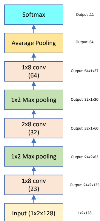
Figure 8. CNN3.
