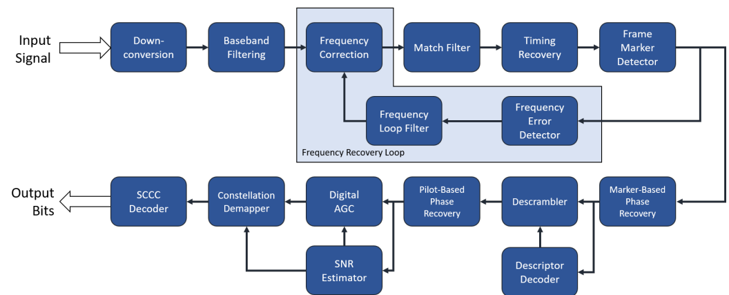
Figure 2. Receiver Architecture.
