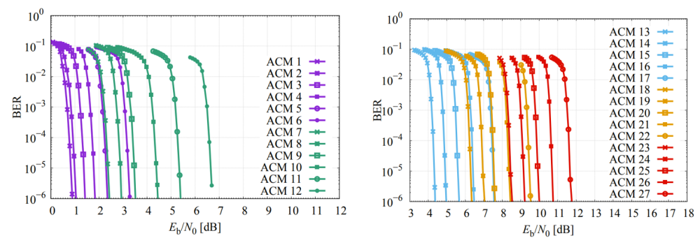
Figure 6. Ideal BER on Linear AWGN Channel for PSK Modulations (left) and APSK Modulations (right)—as defined in [36].
