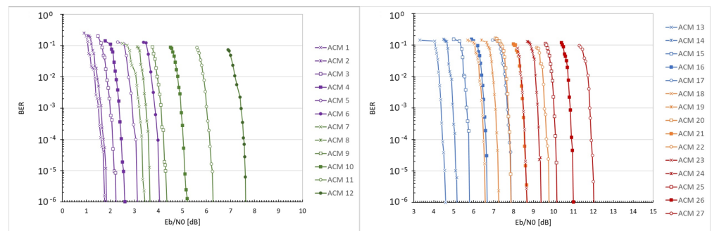
Figure 9. BER curves on linear AWGN channel, drawn for GPU3 implementation.
