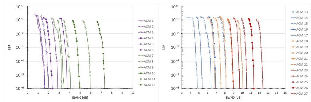
Figure 8. BER curves on linear AWGN channel, drawn for GPU2 implementation.
