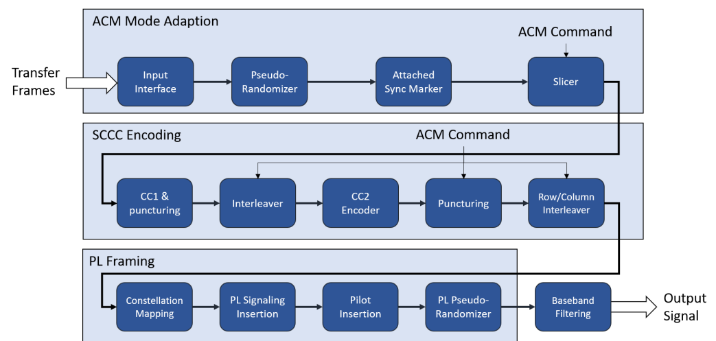
Figure 1. Transmitter Architecture.
