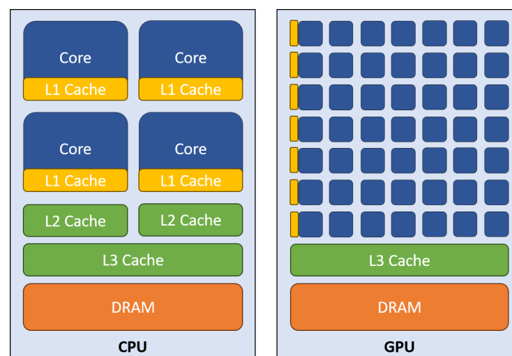
Figure 3. General CPU architecture (left) compared with general GPU architecture (right).
