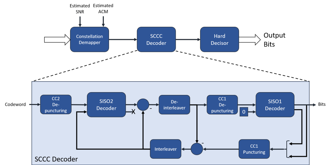
Figure 5. Implemented Back-End Architecture.
