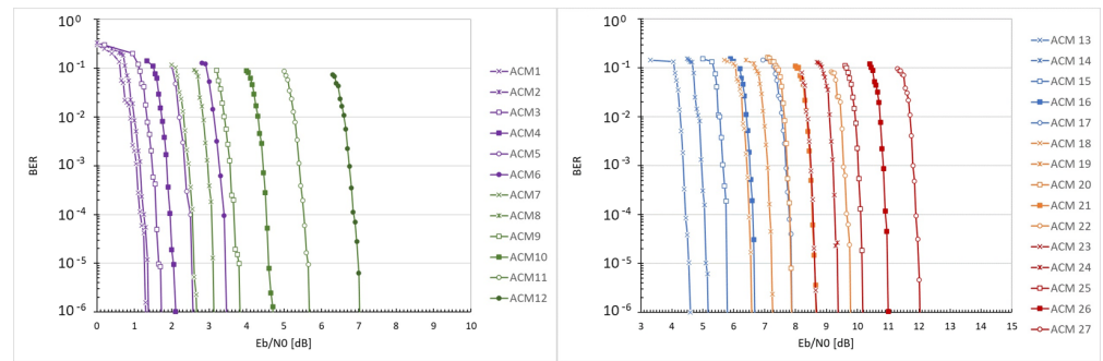
Figure 7. BER curves on linear AWGN channel, drawn for GPU1 implementation.
