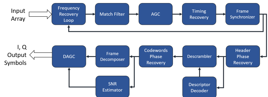
Figure 4. Implemented Front-End Architecture.
