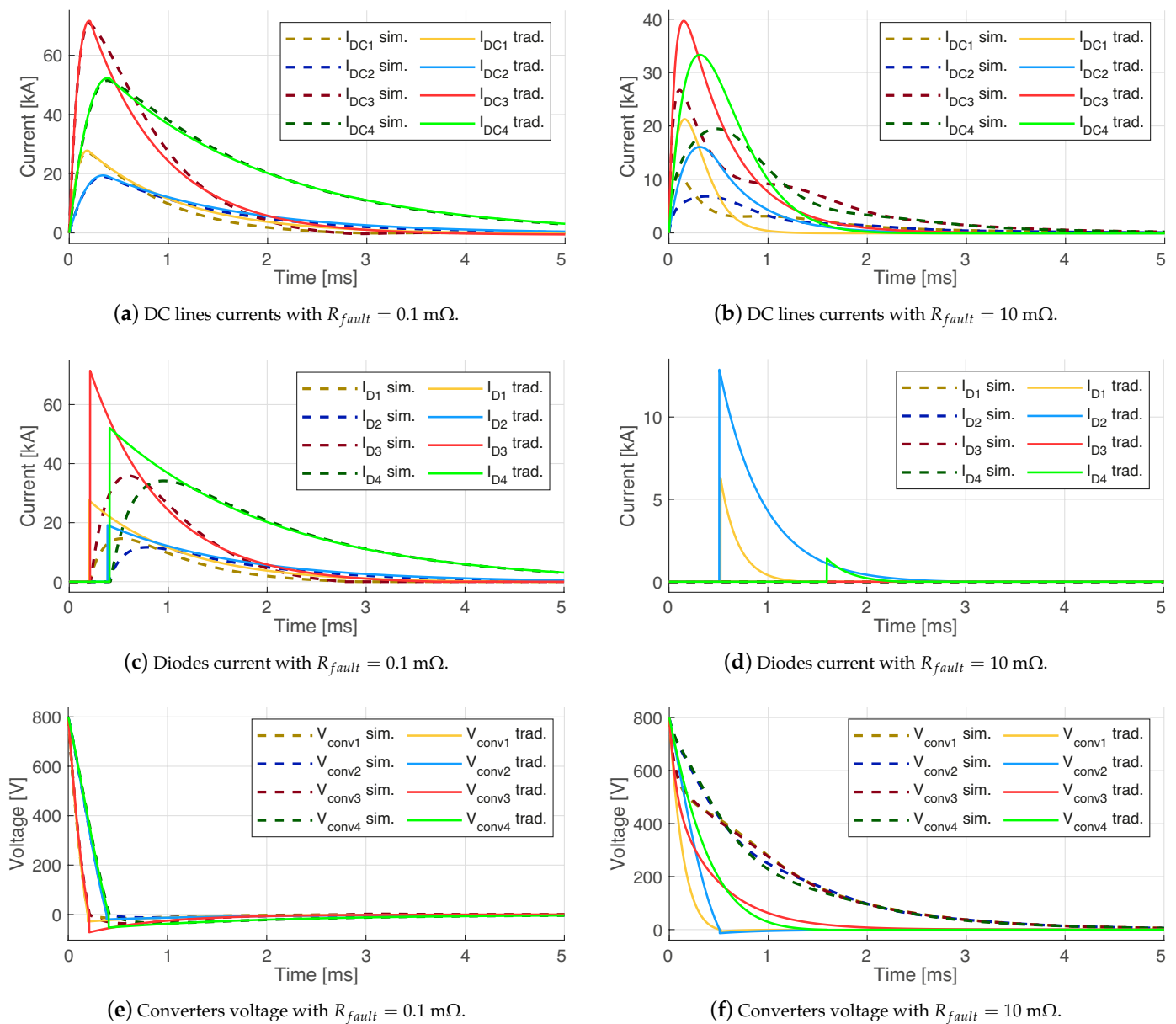
Figure 4. Comparison between traditional DC fault analysis and simulation results.
