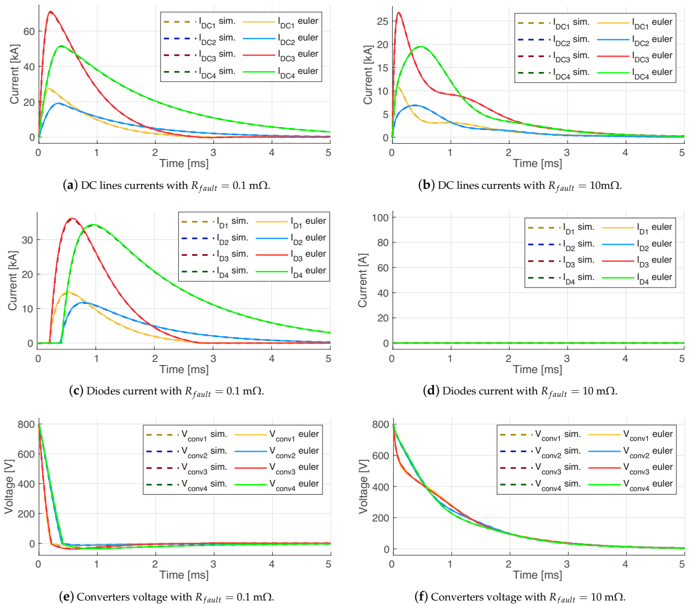
Figure 7. Comparison between proposed method using the general approach and simulation results.
