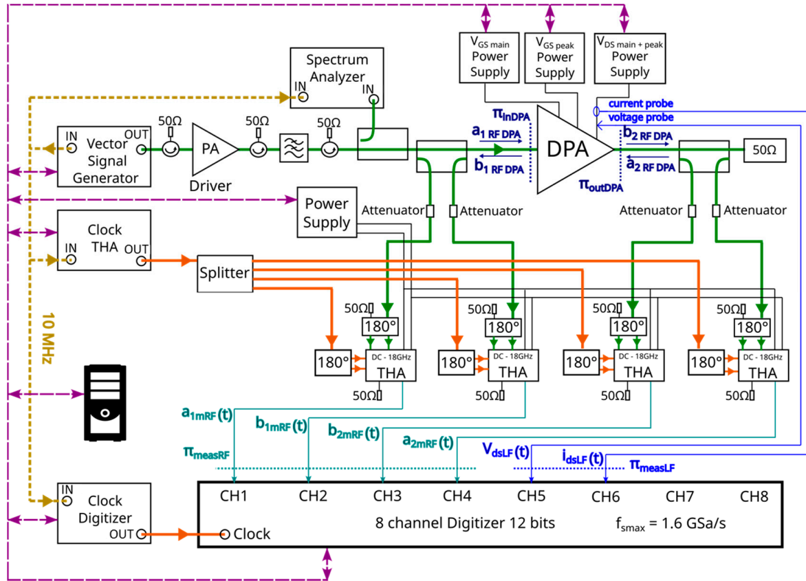
Figure 14. Six-channel time-domain measurement system for power measurements of non-linear devices, driven by the 10 MS/s 16-QAM modulated voltage and injected in the \pi_{inDPA} plane.
