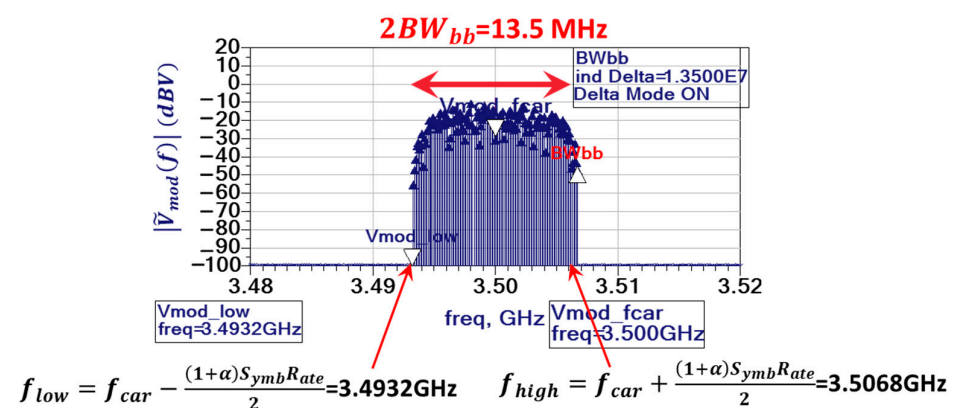
Figure 2. |\tilde{V}_{\text{mod}}(f)| Spectra in the 50 \Omega load after PRM-HB simulation.
