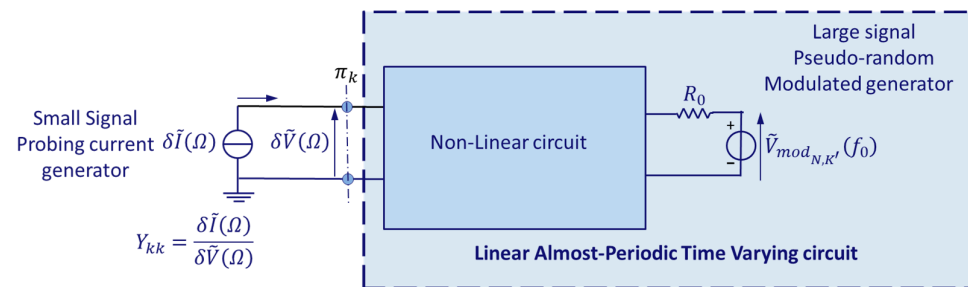
Figure 10. Principle of non-linear LPTV local stability analysis.
