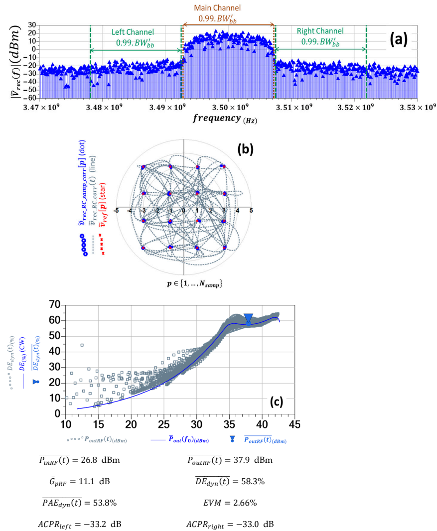
Figure 13. Main results of the PRM-HB simulation of the DPA driven by CW and modulated 16-QAM EMF for A_{car} = 4.45 V (Subfigure (a): |\tilde{V}_{rec}(f)| spectrum—Subfigure (b): 16 QAM reference vector diagram \tilde{v}_{ref}[p] overlaid with the corrected 16 QAM Vector Diagram \tilde{v}_{rec\_RC\_samp\_corr}[p] and the received RC filtered Trajectory \tilde{v}_{rec\_RC\_corr}(t) —Subfigure (c): Dynamic drain efficiency ( DE_{dyn}(t) (%)) versus dynamic output power ( P_{outRF}(t) (dBm)) from PRM-HB simulation overlaid with the CW drain efficiency ( DE(\%) ) versus output power ( \bar{P}_{out}(f_0) (dBm)) from HB simulation).
