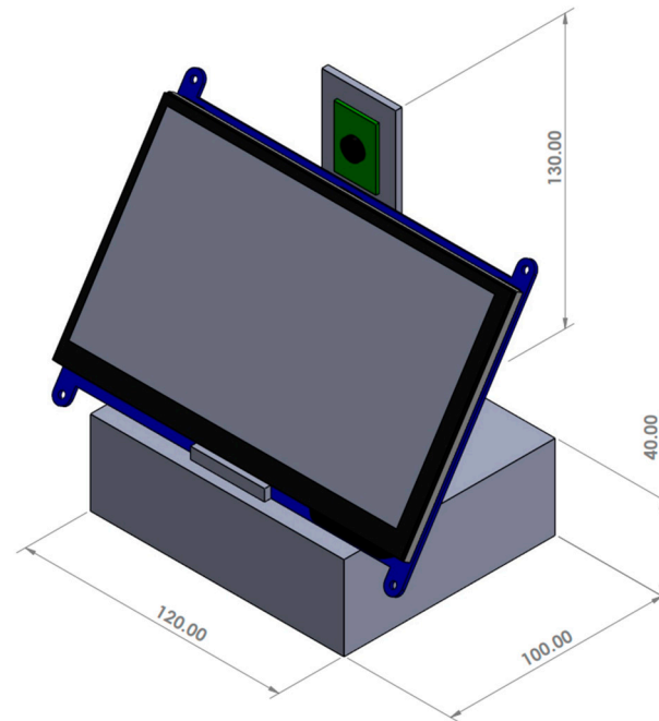
Figure 8. Three-dimensional design of face-aware capture system enclosure with measurements in millimeters (mm).
