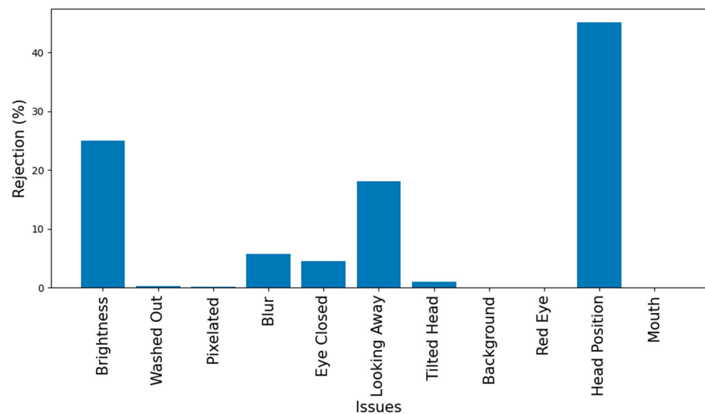
Figure 11. Issues with rejected images of pilot data collection.
