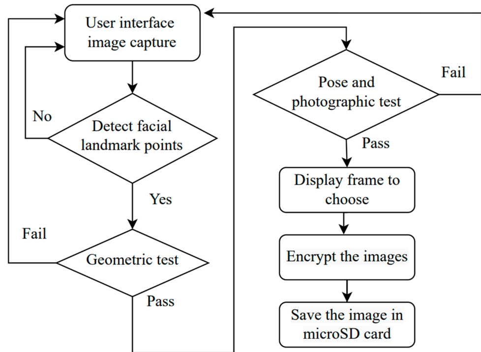
Figure 3. Overview of face-aware capture system software.
