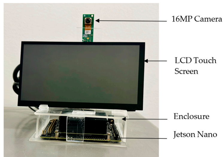
Figure 7. Components of face-aware capture system: The Jetson Nano processor, LCD touchscreen, and a 16 MP camera.
