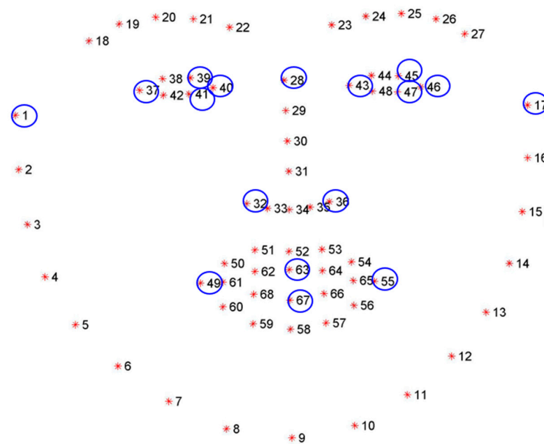
Figure 5. The empirically selected subset (circled in blue) of 68 landmark points used to analyze face quality parameters.
