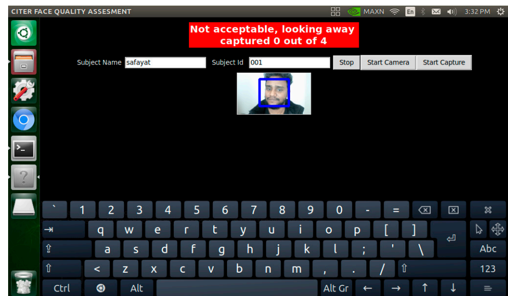
Figure 6. The user interface was developed to give feedback to the user with the bounding box (blue color) for head alignment.
