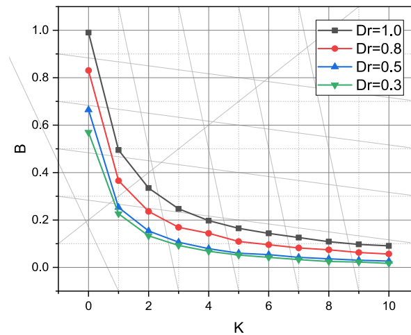
Figure 5. Calculated trajectories of dependence B = f(K, D_r) .
