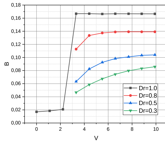
Figure 4. Calculated trajectories of dependence B = f(V, D_r, L = 2) .
