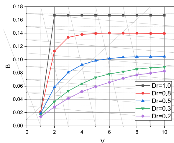
Figure 3. Calculated trajectories of dependence B = f(V, D_r, L = 1) .
