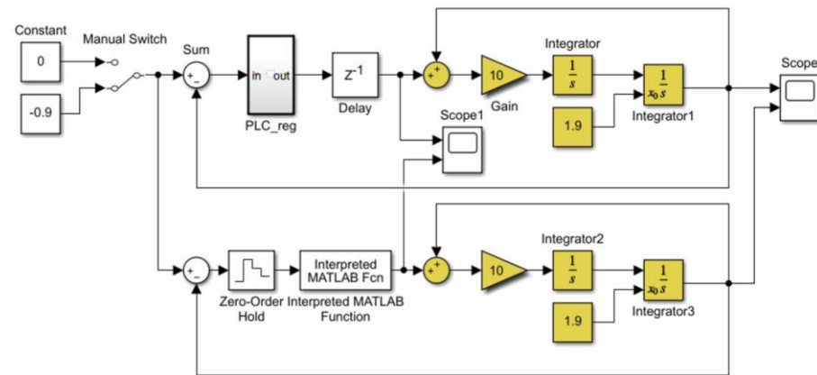
Figure 1. Simulink model of the control loop for an analog unstable second-order object (highlighted in yellow).
