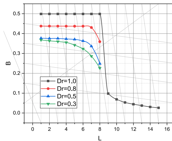
Figure 2. Calculated trajectories of dependence B = f(L, D_r) .
