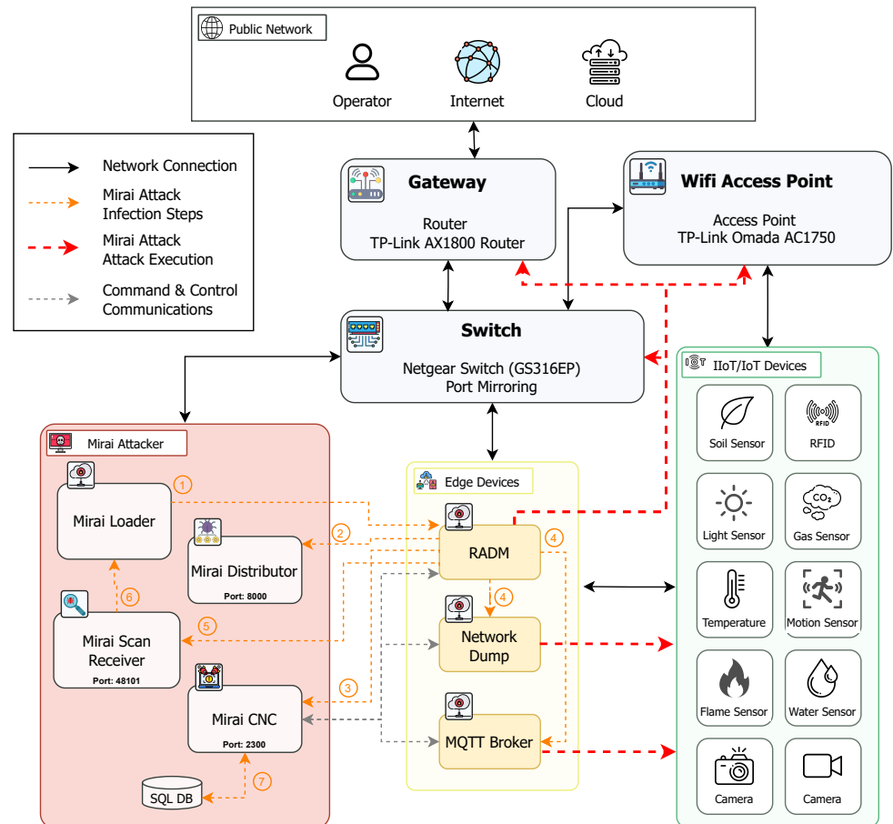
Figure 7. Attack framework for Mirai attack execution in the testbed.
