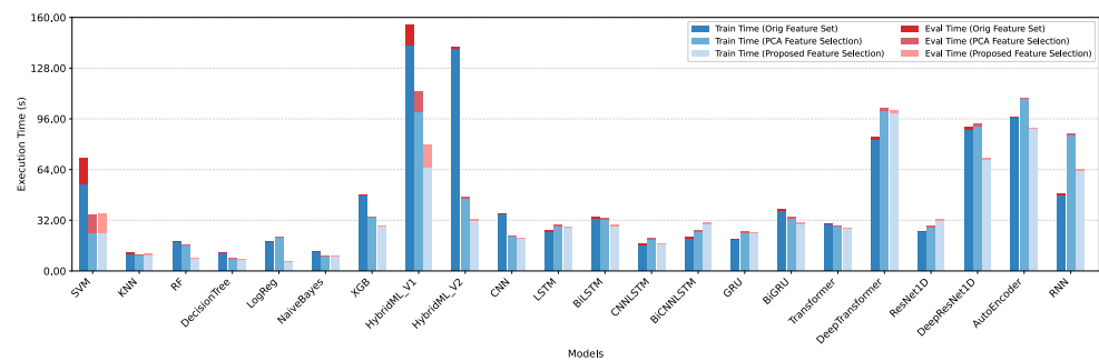
Figure 18. Impact of feature selection on training and evaluation time in 50-class classification.
