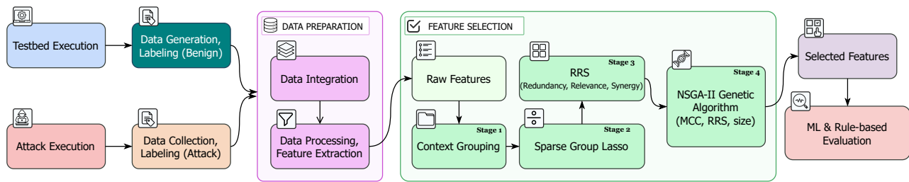
Figure 8. Proposed data generation workflow and feature engineering.
