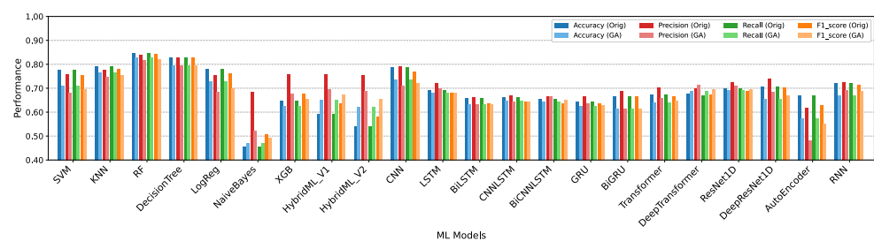
Figure 15. Impact of feature selection on 50-class classification performance.
