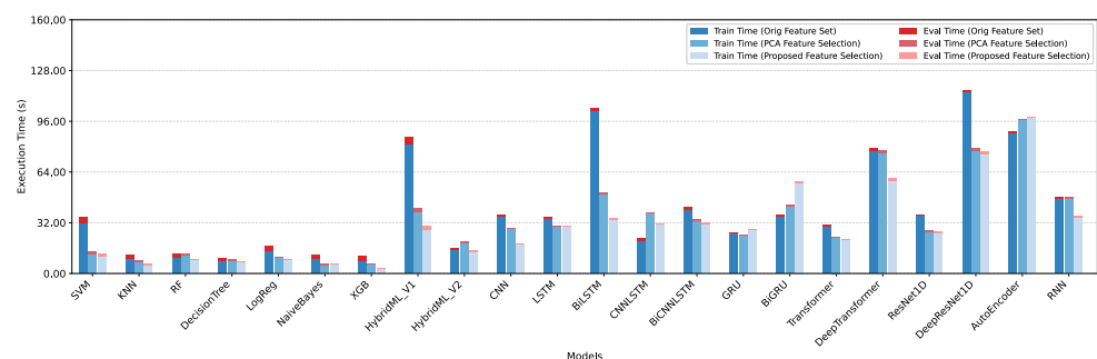
Figure 16. Impact of feature selection on training and evaluation time in binary classification.
