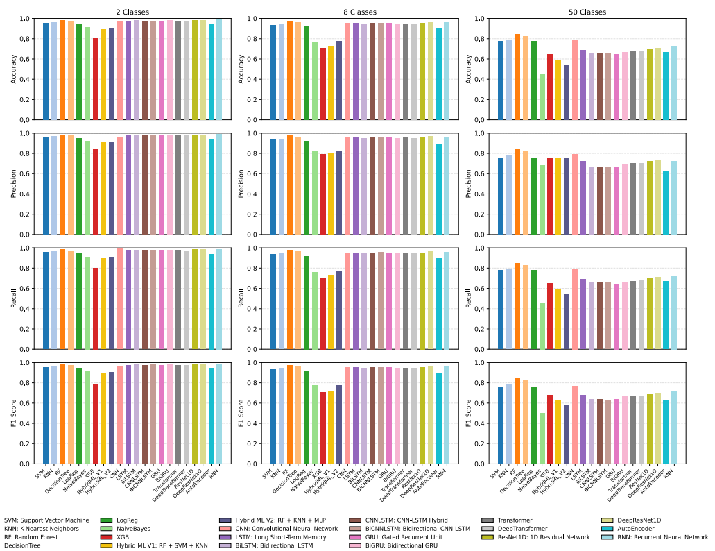
Figure 12. Results for anomaly detection on proposed dataset using different ML and DL techniques.
