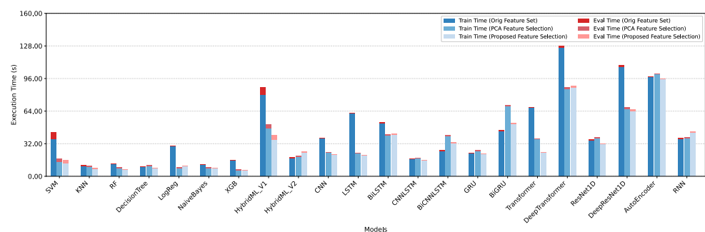
Figure 17. Impact of feature selection on training and evaluation time in eight-class classification.
