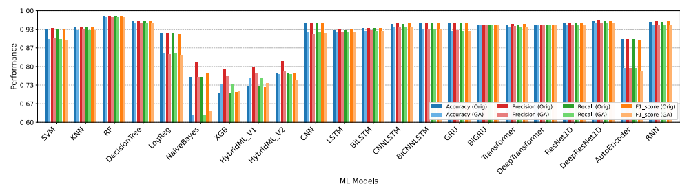
Figure 14. Impact of feature selection on eight-class classification performance.
