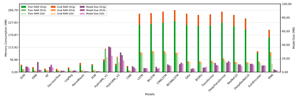
Figure 19. Impact of feature selection on resource usage in binary classification.
