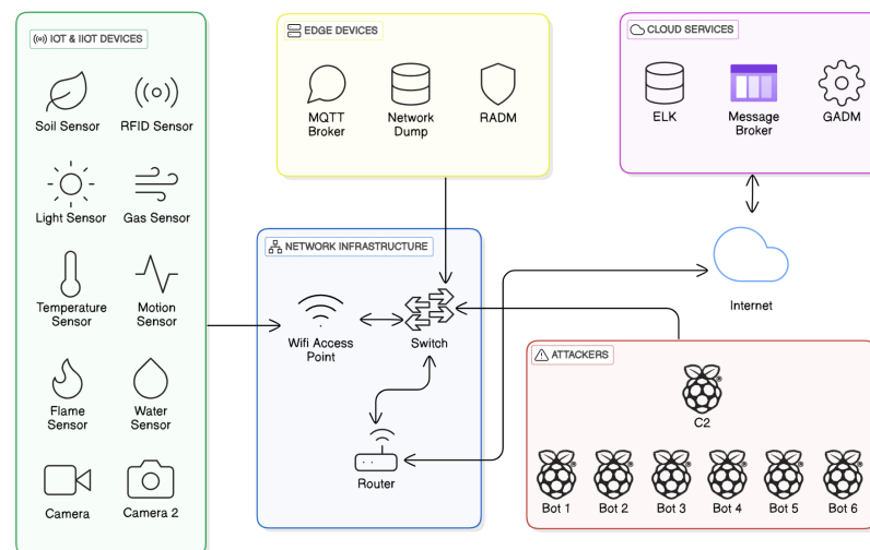
Figure 2. DataSense testbed overall architecture.
