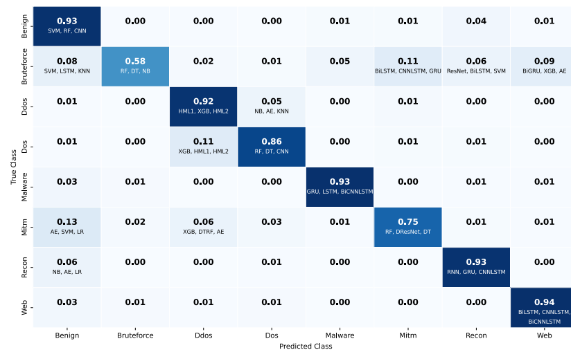
Figure 22. Aggregated confusion matrix showing misclassifications accross different models in eight-class scenario.
