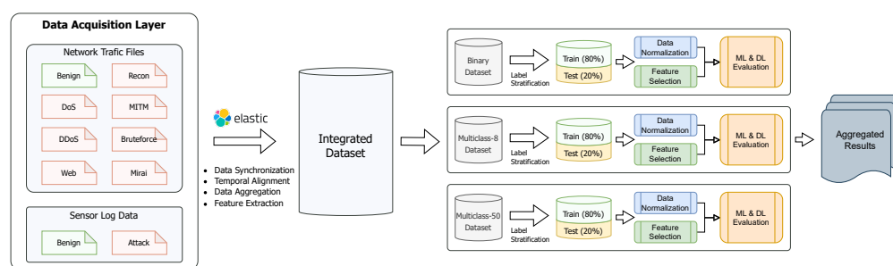
Figure 11. Datasense evaluation pipeline for anomaly detection in IIoT environments.
