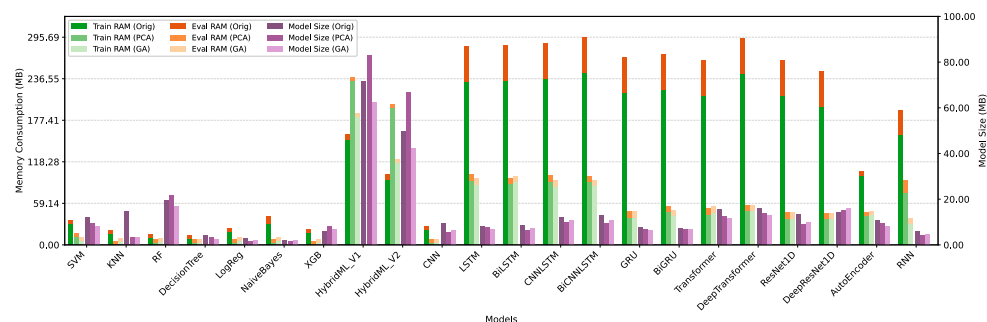
Figure 20. Impact of feature selection on resource usage in eight-class classification.
