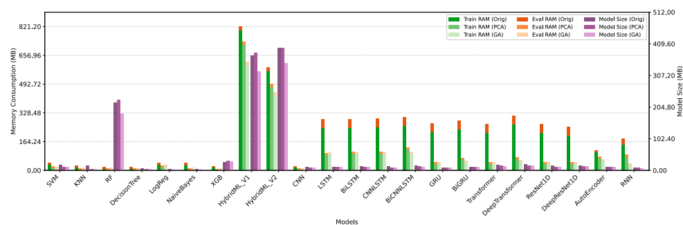
Figure 21. Impact of feature selection on resource usage in 50-class classification.
