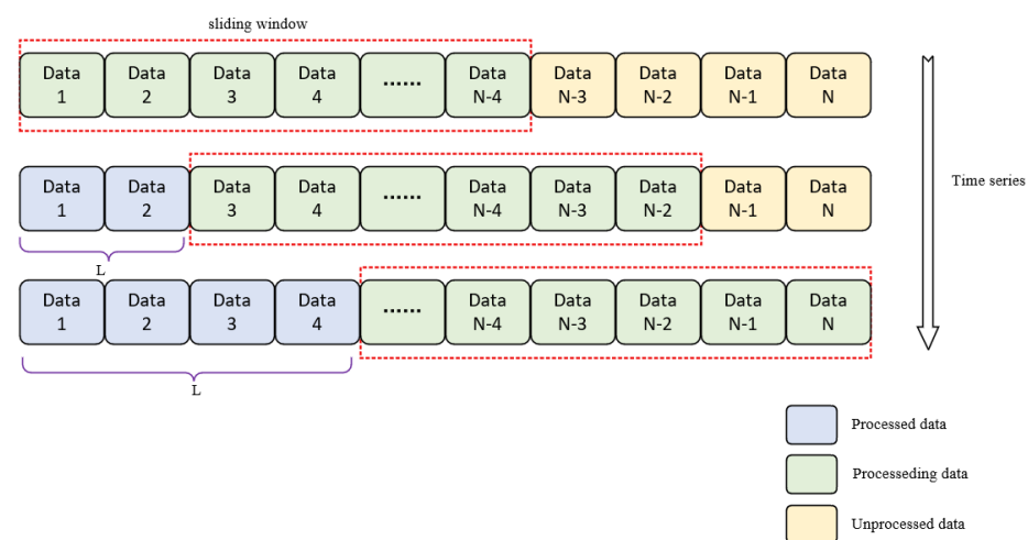
Figure 3. Feature-based sliding window mechanism.
