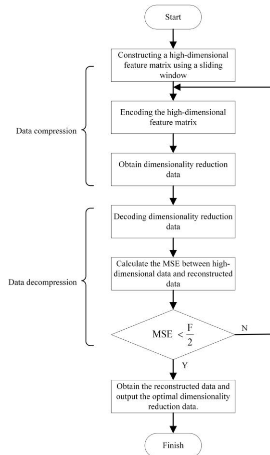
Figure 4. Flowchart of the autoencoder.
