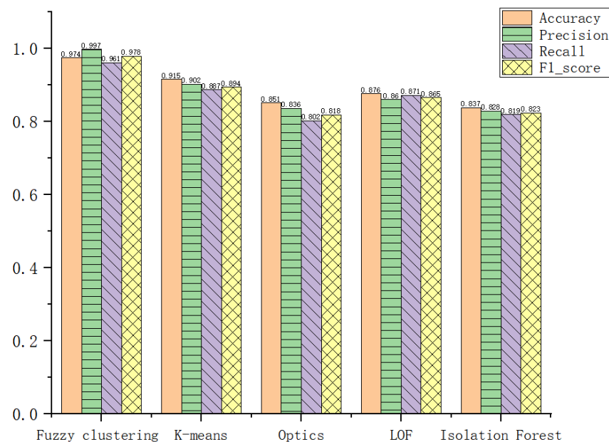
Figure 11. Network anomaly detection results.
