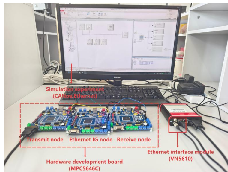
Figure 7. Actual experimental environment.
