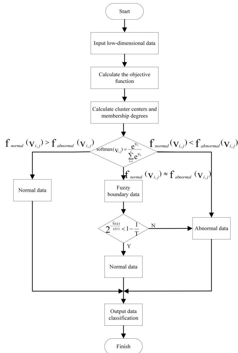
Figure 5. Flowchart for network anomaly detection.
