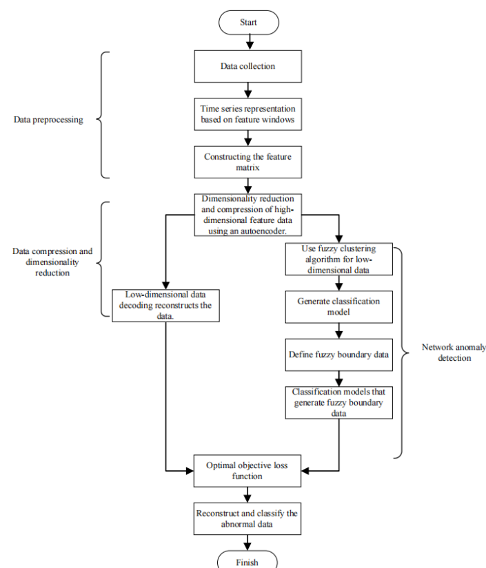
Figure 2. Flowchart of Network Anomaly Detection.
