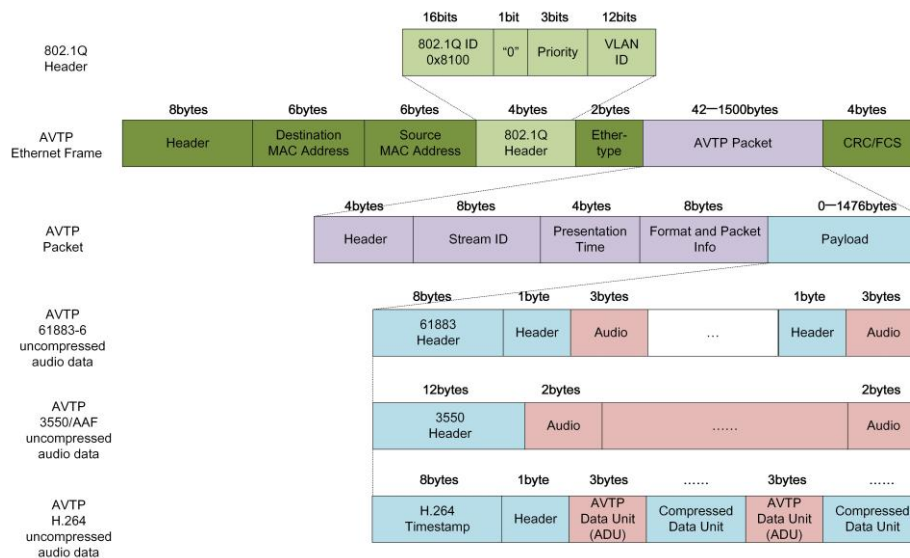
Figure 1. AVTP protocol data frame format.
