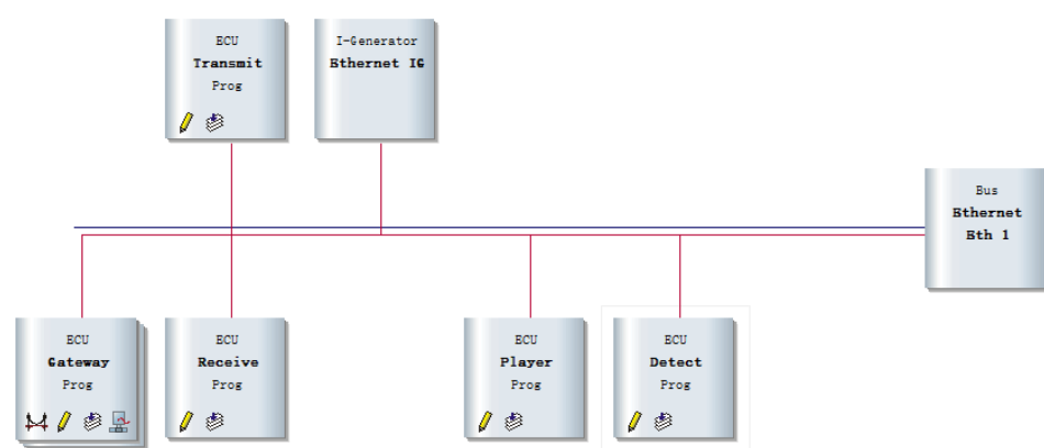
Figure 6. Network topology architecture of In-Vehicle Ethernet.
