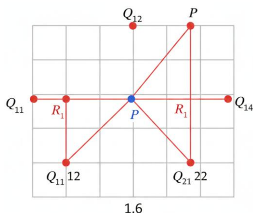
Figure 13. Bilinear Interpolation Method.
