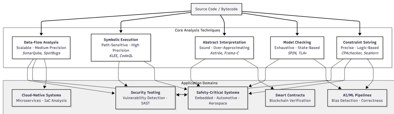
Figure 3. Taxonomy of static analysis techniques and their application domains.
