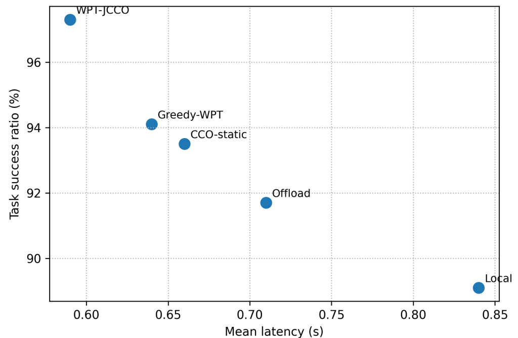
Figure 3. Latency-success trade-off. WPT-JCCO improves both latency and task success by coupling charging with offloading and radio allocation.
