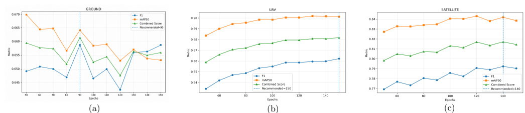
Figure 4. Sensitivity analysis on the performance of YOLO algorithm in ground-based imagery (a), UAV-based imagery (b), and satellite-based imagery (c) across training epochs.
