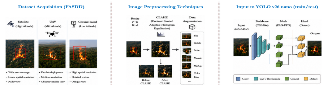
Figure 2. Methodology work-flow for forest fire recognition utilizing YOLO v26 nano in ground-based, UAV, and satellite imagery.
