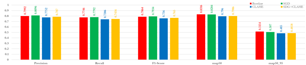
Figure 11. Mean precision, recall, F1-score, mAP_50, and mAP_50–95 after five-fold cross-validation of YOLOv26-nano on satellite imagery.
