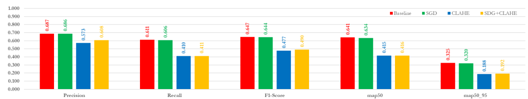
Figure 5. Averaged Precision, Recall, F1-Score, mAP 50 and mAP 50-95 metrics after the five-fold cross validation of YOLO v26 nano on the ground based imagery.
