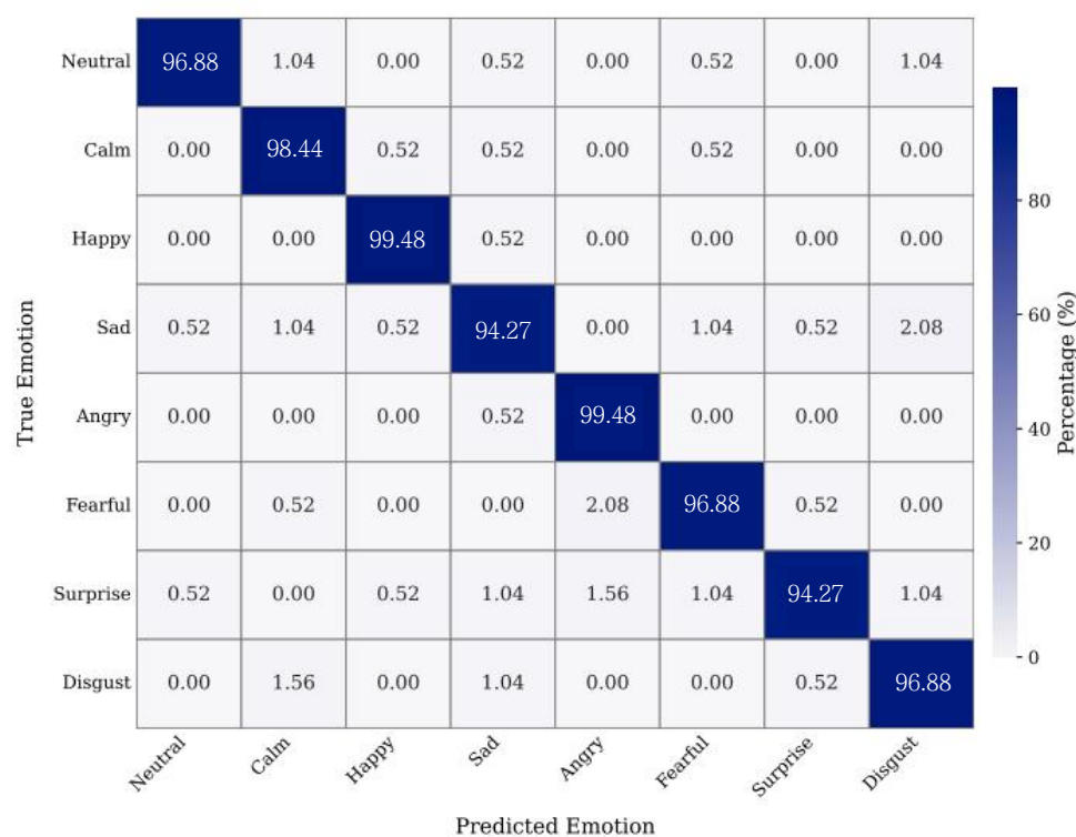
Figure 3. Confusion matrix of the proposed model on the RAVDESS test set.
