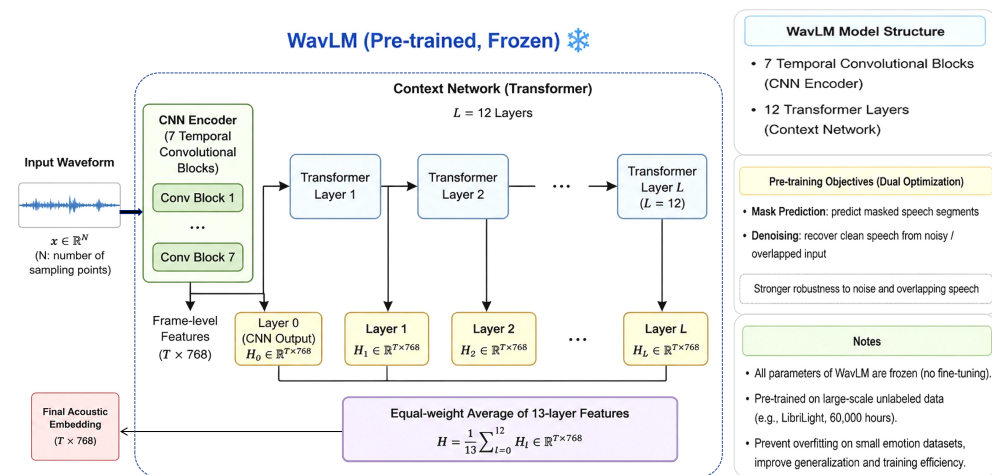
Figure 2. WavLM Feature extraction process.
