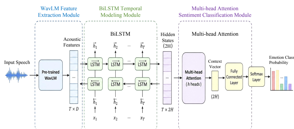
Figure 1. Speech emotion analysis framework.
