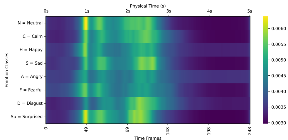
Figure 6. Attention distribution of eight emotion categories on the RAVDESS dataset.
