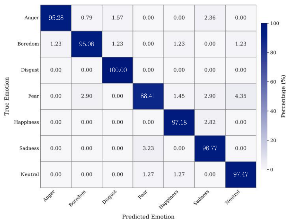
Figure 4. Confusion matrix of the proposed model on the EmoDB test set.
