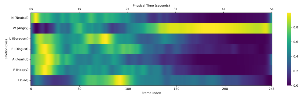
Figure 5. Attention distribution of seven emotion categories on the EmoDB dataset.
