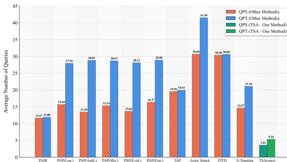
Figure 3. Comparison of query costs across various attack methods on the MiniAdvBench benchmark. This figure illustrates the QPS and QPT of each attack method across nine tested LLMs. The experimental results show that under our experimental conditions, our TSA method achieves the lowest query cost while maintaining the highest ASR. The abbreviations for the five PAP variants are explained in the caption of Table 1.
