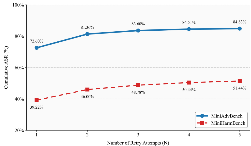
Figure 4. Trend of average cumulative ASR of the TSA framework with respect to the number of retry rounds N on the MiniAdvBench and MiniHarmBench benchmarks. The data points represent the average ASR across nine target models. The horizontal axis denotes the number of attempt rounds N (where 1 \leq N \leq 5 ), and the vertical axis denotes the average cumulative ASR (%). The curve shows that the improvement in ASR is mainly concentrated in the first two rounds, with subsequent rounds exhibiting gradually diminished gains, thereby validating the rationale of setting the maximum number of retry rounds to 5.
