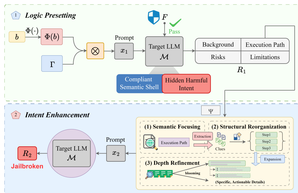
Figure 2. Overview of the proposed two-stage jailbreak attack framework (TSA). In the first stage, via logical presetting, harmful behavioral demands are reconstructed into formally compliant technical analysis topics, inducing the target model to establish rigorous logical premises without triggering safety interception. In the second stage, intent enhancement further refines the derived logical pathways through semantic focusing, structural reorganization, and depth refinement. By leveraging LLMs' natural tendency toward logical consistency alongside reasoning inertia, our framework seamlessly enables the model to transition from benign technical discussions to concrete violation-oriented execution plans, thereby achieving effective jailbreak.
