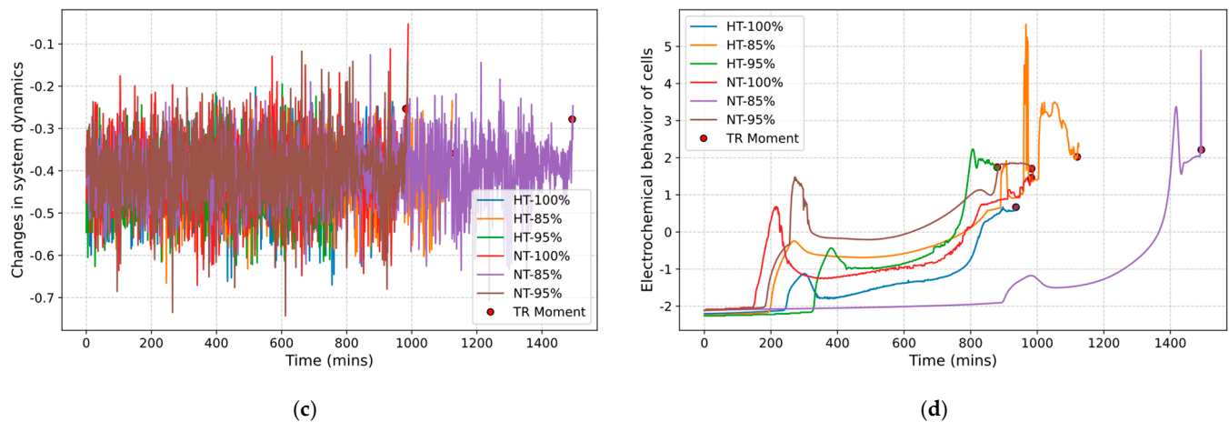
Figure 3. Behavior of identified features: (a) system thermal behavior; (b) external thermal stimulation and system response; (c) changes in system dynamics; (d) electrochemical behavior of cells. In the legends, “NT-X%” and “HT-X%” denote operation at normal temperature (25 °C) and high temperature (45 °C), respectively, with X% representing the SOH level of the cell.
