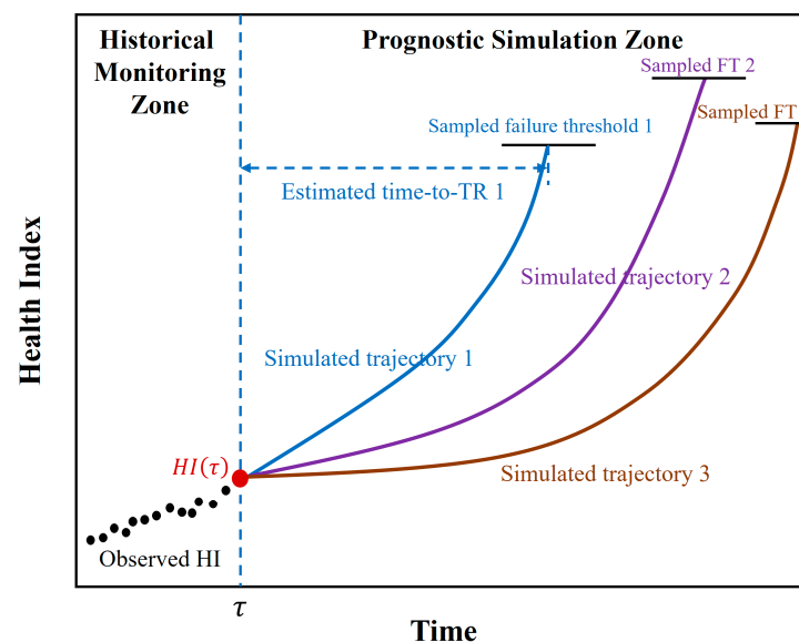
Figure 2. Schematic illustration of time-to-TR estimation.
