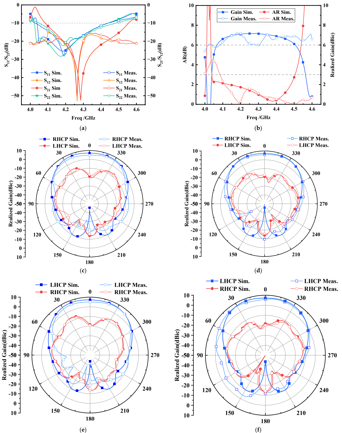
Figure 8. Simulated and measured antenna performance: (a) S-parameters; (b) broadside AR and realized gain under Port 1 excitation; (c) radiation patterns in the xoz plane under Port 1 excitation at 4.3 GHz; (d) radiation patterns in the yoz plane under Port 1 excitation at 4.3 GHz; (e) radiation
