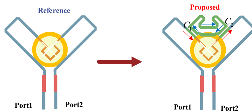
Figure 2. Design evolution from the reference DCP antenna to the proposed antenna with the DFN.
