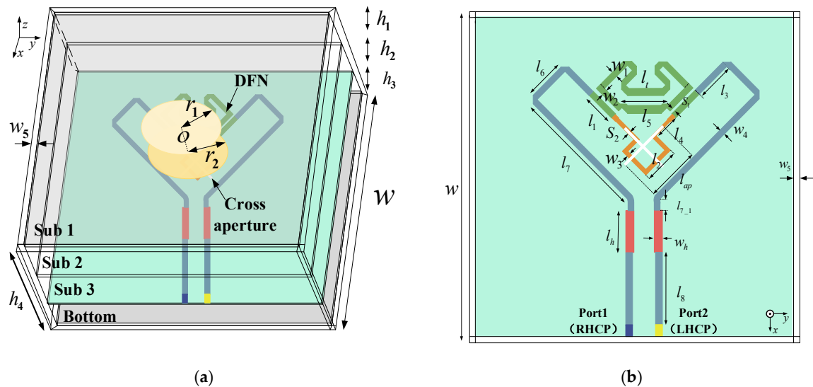
Figure 1. Configuration of the proposed DCP STAR antenna and its cavity-backed integration model: (a) three-dimensional antenna and cavity-backed assembly; (b) top view of the cross-shaped aperture, feeding paths, and DFN.
