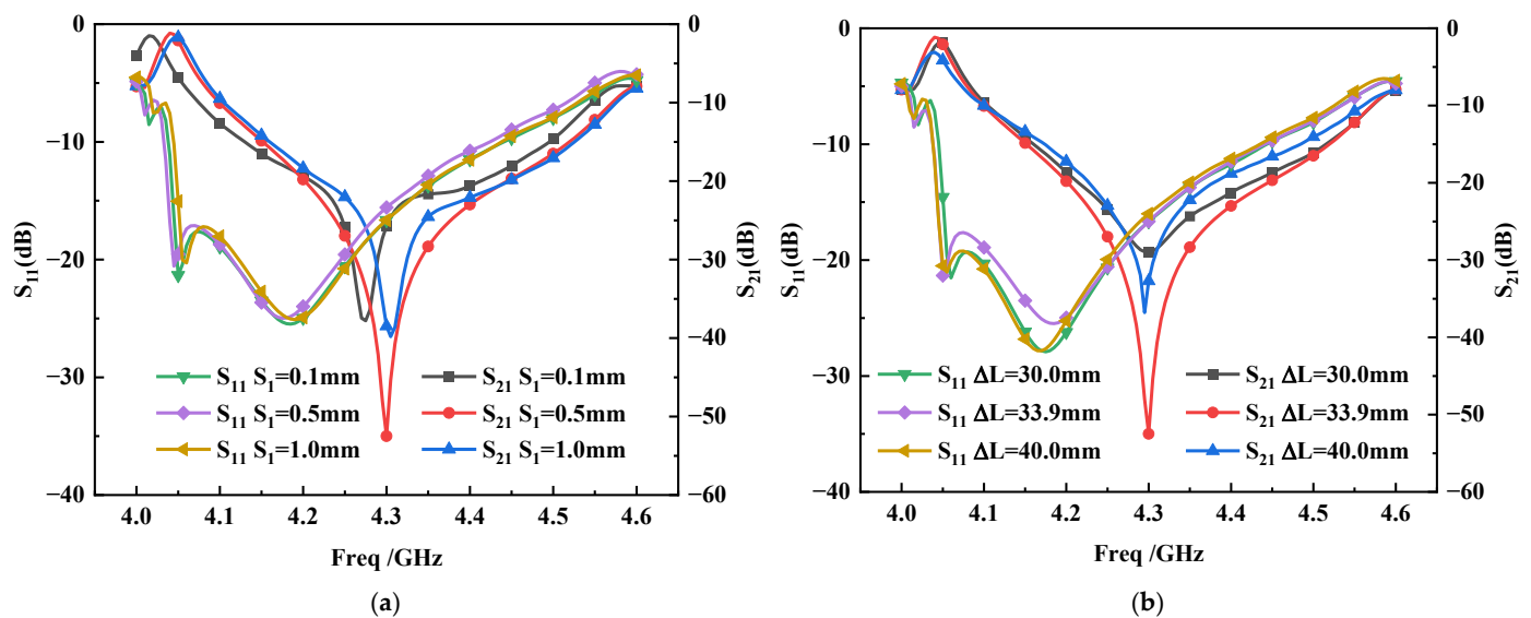
Figure 3. Simulated S_{11} and S_{21} responses for different DFN tuning parameters: (a) coupled-line spacing S_1 ; (b) effective DFN phase-control length \Delta L .
