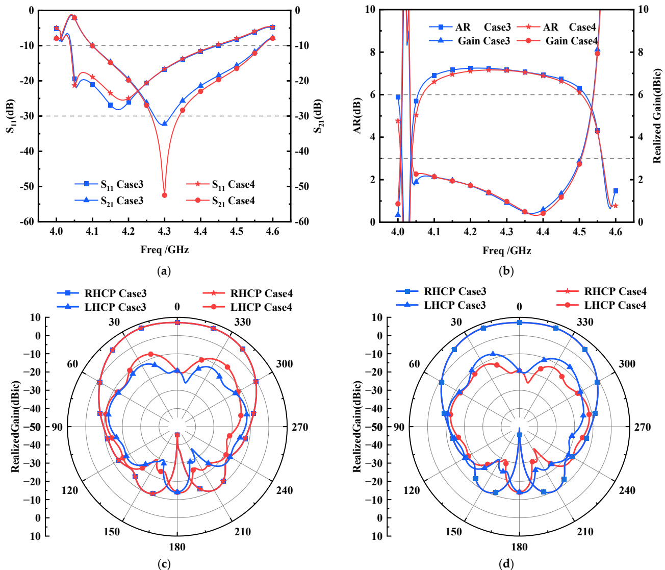
Figure 5. Simulated responses of the cavity-backed antenna without and with the DFN: (a) S_{11} and S_{21} ; (b) AR and realized gain; (c) radiation patterns in the xoz plane at 4.3 GHz; (d) radiation patterns in the yoz plane at 4.3 GHz.
