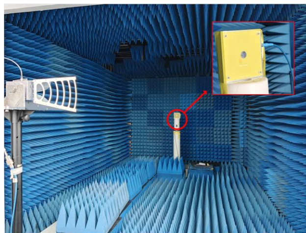
Figure 7. Measurement setup in the microwave anechoic chamber.
