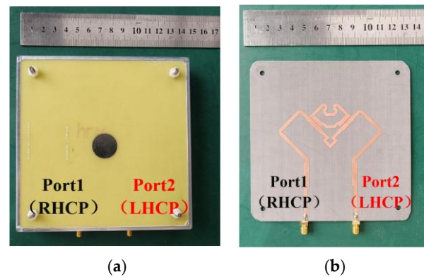
Figure 6. Photographs of the fabricated antenna: (a) top view; (b) bottom view.
