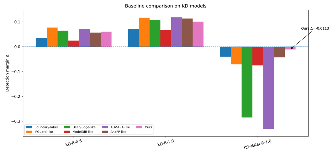
Figure 4. Multi-baseline detection margin comparison on boundary-enhanced distillation models.
