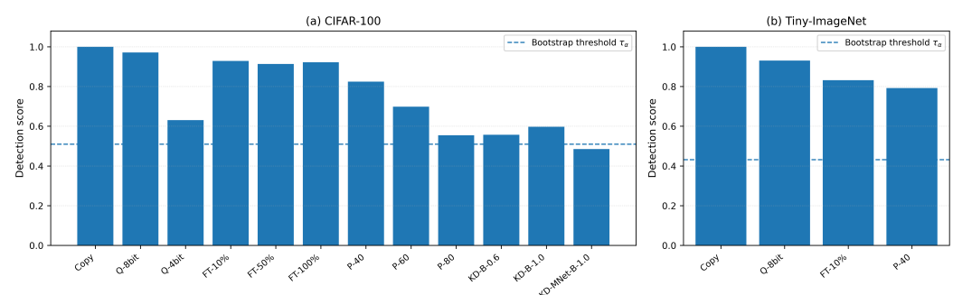
Figure 2. Main detection results on both datasets.
