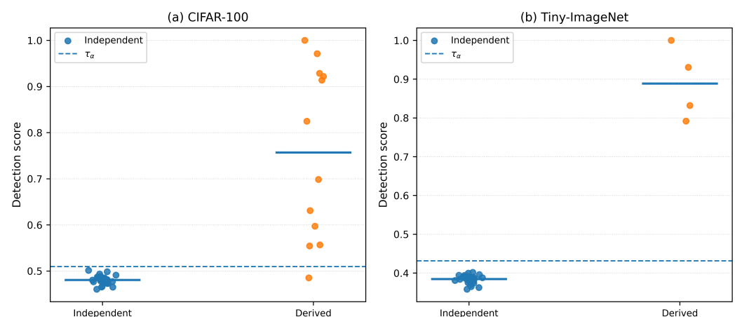
Figure 3. Distribution of detection scores for independent models and derived models.
