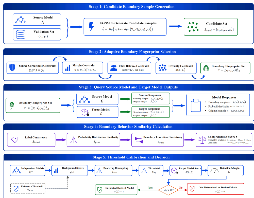
Figure 1. Flowchart of black-box model copyright verification based on adaptive boundary fingerprints.
