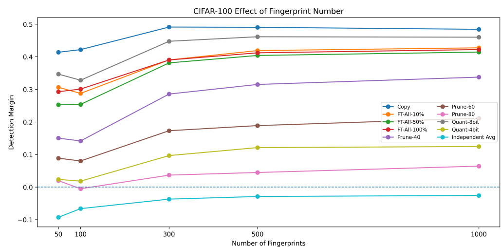
Figure 7. Impact of fingerprint sample size on detection margin.
