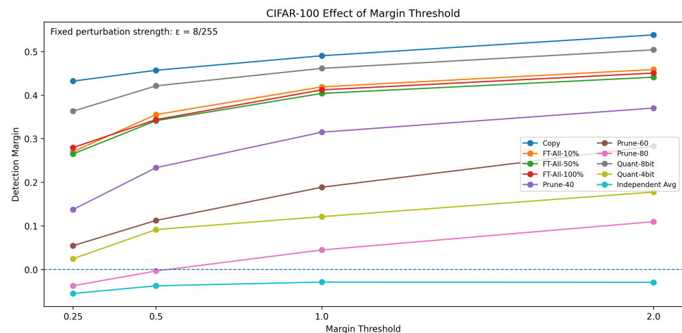
Figure 9. Impact of classification margin threshold on detection margin.
