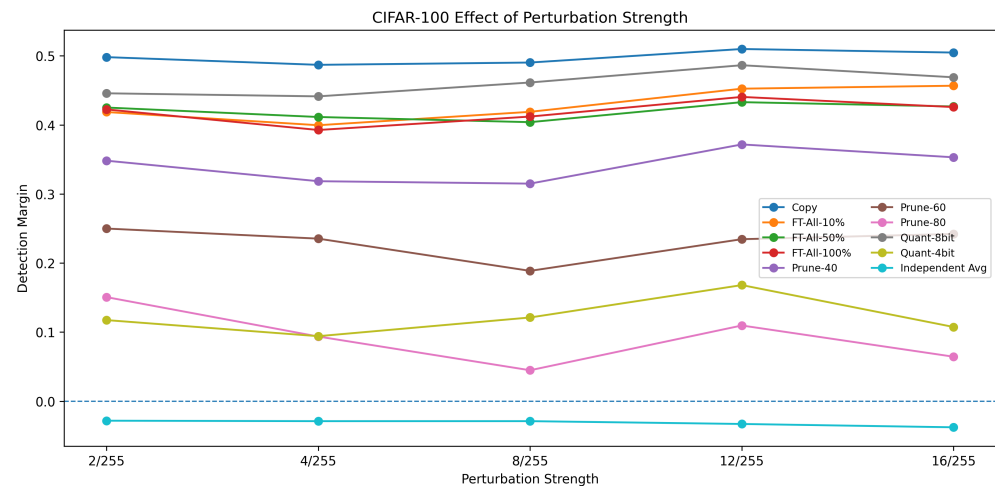
Figure 8. Impact of perturbation strength on detection margin.
