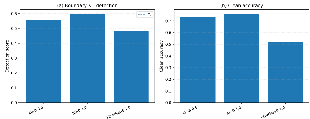
Figure 5. Detection results for boundary-enhanced distillation models.
