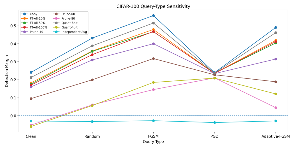
Figure 6. Impact of query sample type on detection margin.
