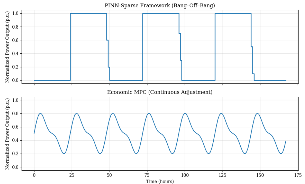
Figure 8. Illustrative comparison of actuation patterns under sparse and continuous control policies. The top panel shows the characteristic bang–off–bang switching profile of the PINN-Sparse framework, while the bottom panel shows the continuously varying profile of Economic MPC. The observed near-binary switching pattern is qualitatively consistent with the quasi-threshold sparse structure suggested by Proposition 1.
