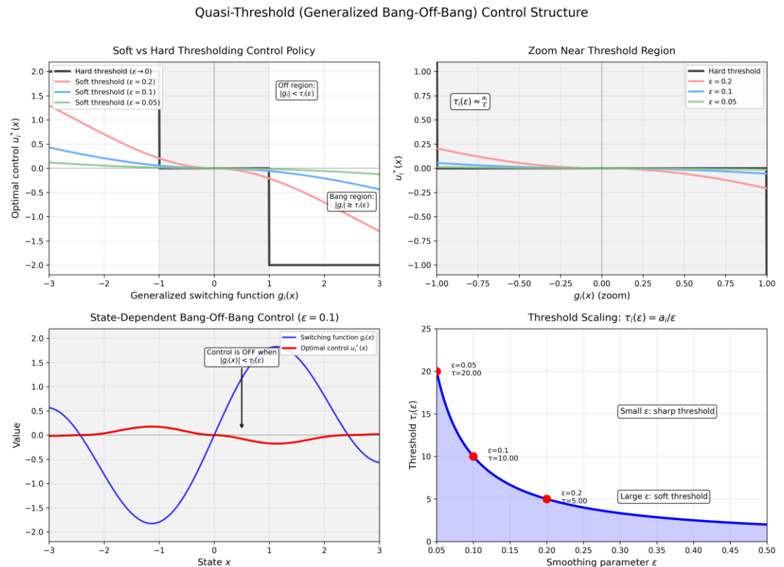
Figure 2. Illustration of the quasi-threshold (generalized bang-off-bang) control structure.
