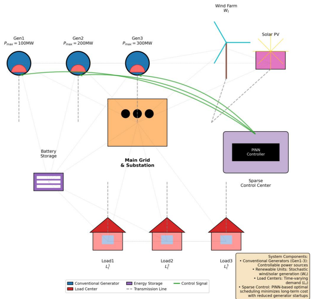
Figure 7. Schematic design of the renewable-integrated smart grid system architecture.
