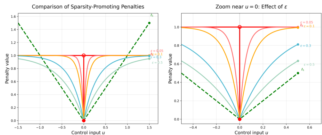
Figure 1. Comparison of Sparsity-Promoting Penalties.
