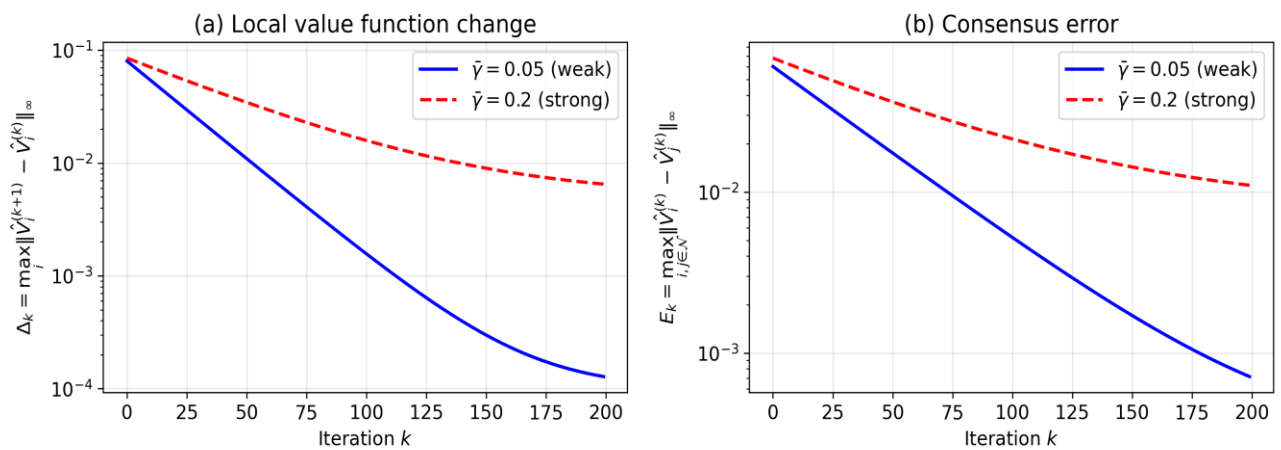
Figure 6. Convergence of the distributed monotone scheme. (a): maximum change \Delta_k in local value functions; (b): consensus error E_k . Blue curves: weak coupling ( \bar{\gamma} = 0.05 ); red dashed curves: strong coupling ( \bar{\gamma} = 0.2 ).
