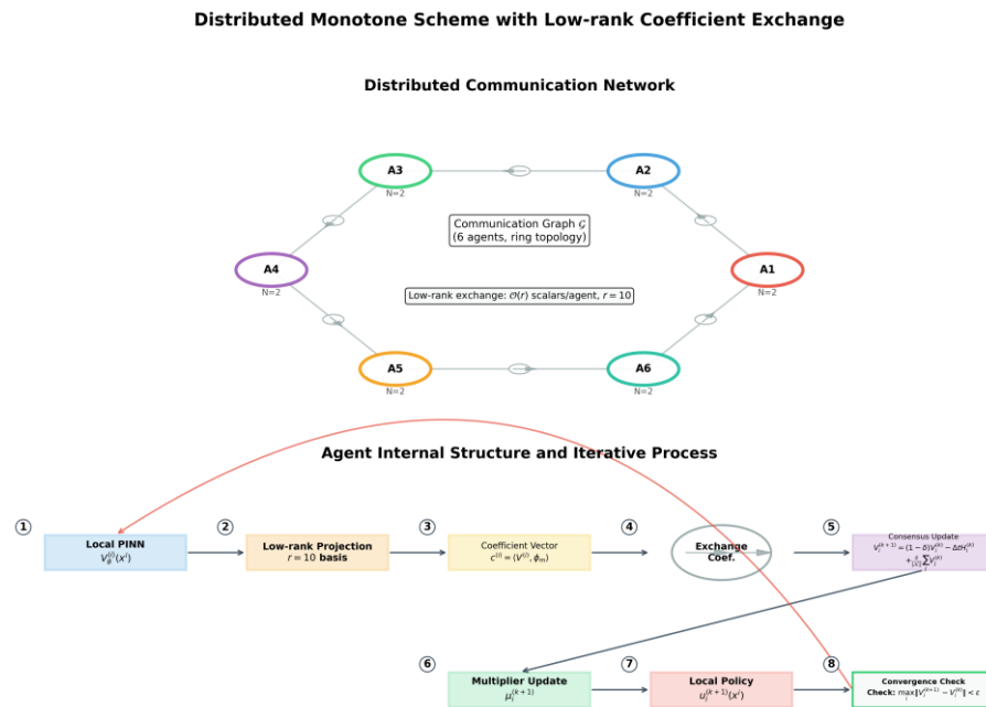
Figure 4. Distributed monotone scheme with low-rank coefficient exchange.
