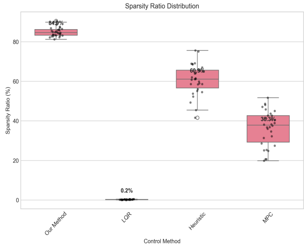
Figure 11. Sparsity Ratio Distribution.
