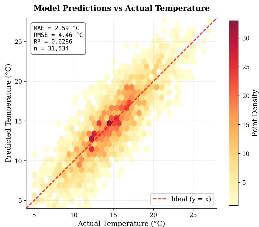
Figure 5. Scatter plot of model predictions versus actual temperature values on the temporal validation set (31,534 samples).
