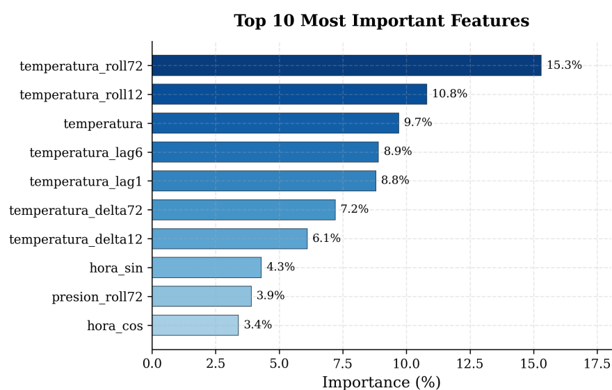
Figure 4. Top 10 most important features of the Random Forest model.
