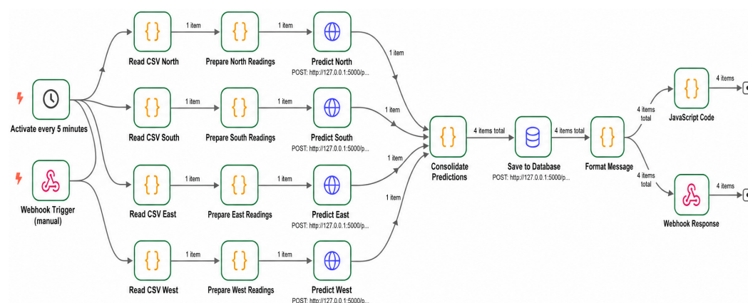
Figure 3. n8n orchestration workflow for ClimaBogotá v1.2.
