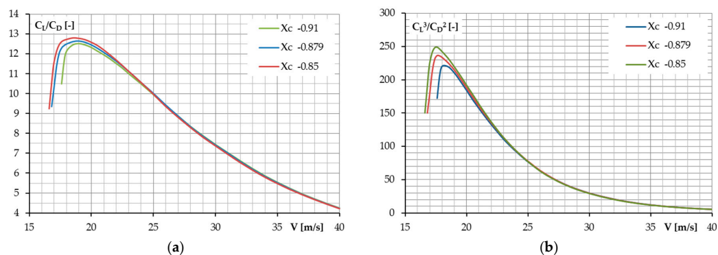
Figure 15. The airplane’s aerodynamic characteristics’ variation with the centre of gravity (CG) position: (a) C_L/C_D ratio; and (b) power coefficient C_L^3/C_D^2 with respect to the airspeed.
