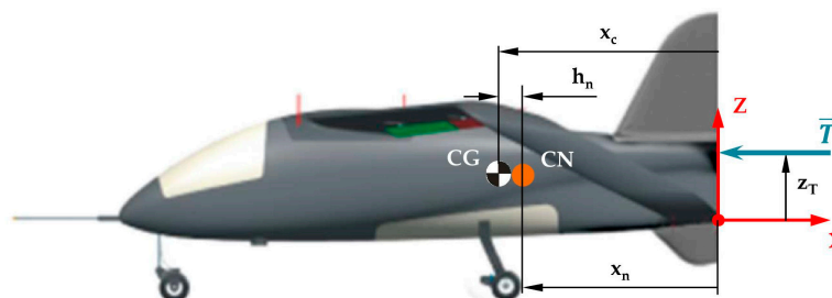
Figure 12. Center of gravity, neutral point position, and local axis system convention (Łukasz Stefanek).
