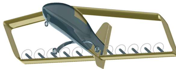
Figure 11. Concept of the inverted joined wing airplane with distributed propulsion.
