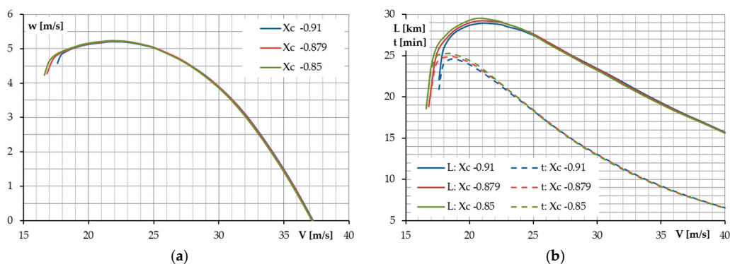
Figure 16. Variation in the airplane’s performance with the CG position: (a) maximum climb rate; and (b) range and flight duration with respect to the airspeed.
