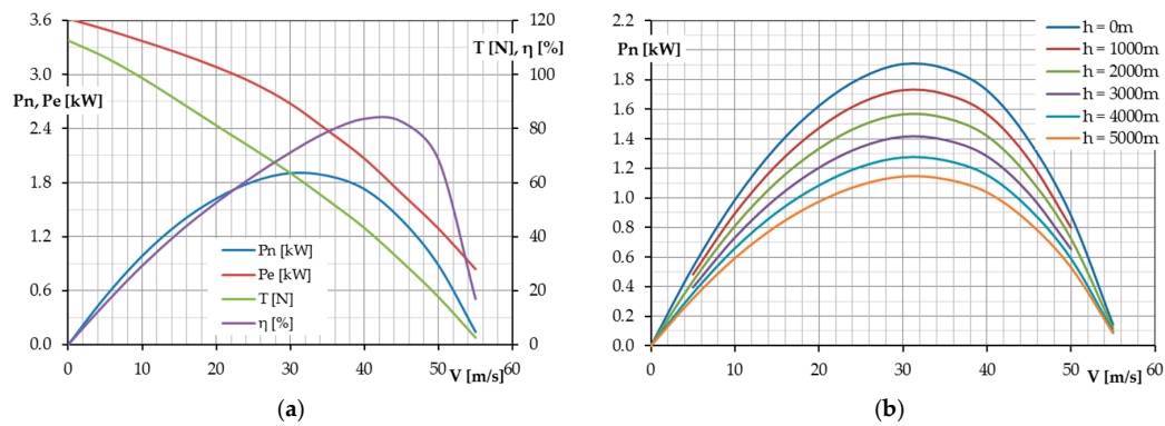
Figure 3. (a) Propulsion unit characteristics: P_e —motor electric power, P_n —effective power, \eta —total efficiency, T —thrust; and (b) power available versus airspeed for several flight altitudes.
