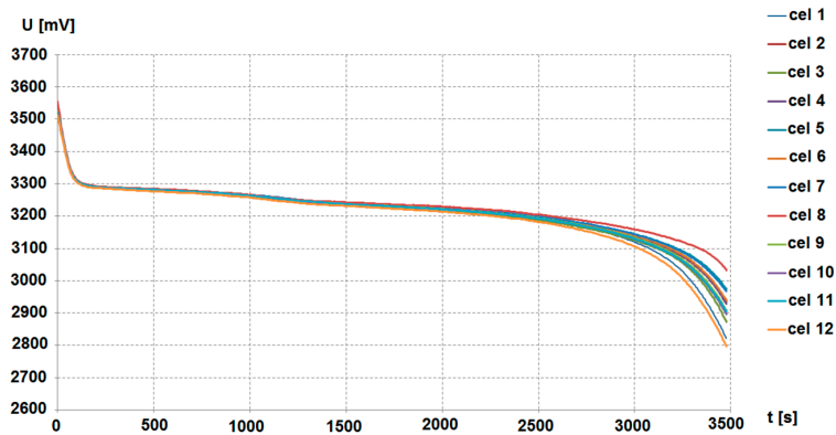
Figure 8. Example of discharge characteristics of the propulsion battery after 1.5 years of use. Discharge current: 2.3 A.
