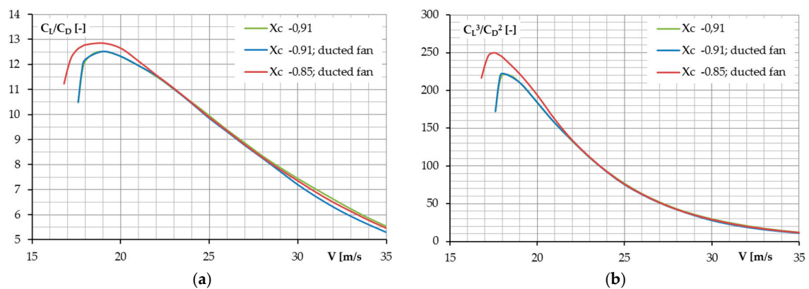
Figure 23. Variation in the airplane's aerodynamic characteristics with CG position for the configuration with a ducted fan: (a) C_L/C_D ratio; and (b) power coefficient C_L^3/C_D^2 with respect to the airspeed.
