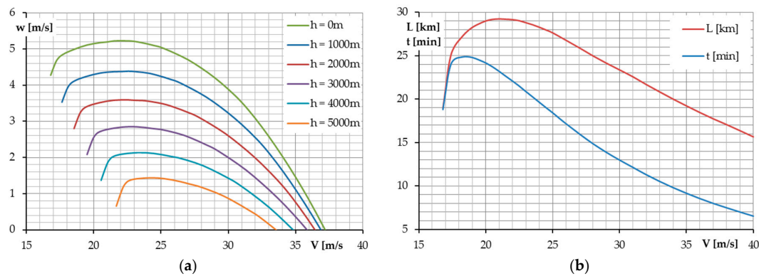
Figure 4. (a) Maximum climb rate versus airspeed for several flight altitudes; and (b) maximum range and endurance versus airspeed for simple cruise mission.
