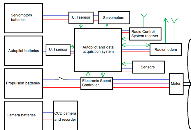
Figure 5. Electric/electronic system architecture of the demonstrator. CCD: charge-coupled device.
