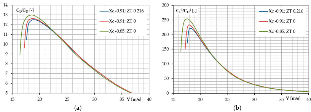
Figure 19. Variation in the airplane's aerodynamic characteristics with the CG position: (a) C_L/C_D ratio; and (b) power coefficient C_L^3/C_D^2 with respect to the airspeed.
