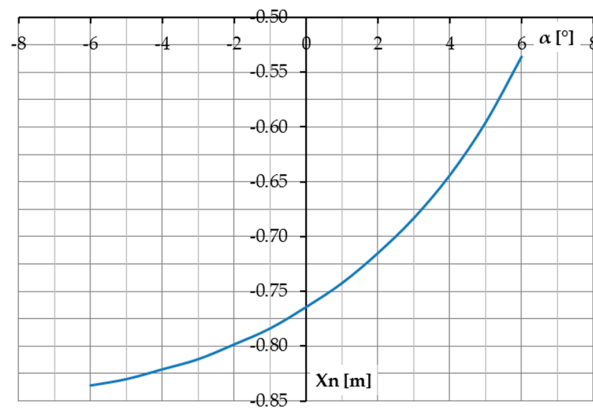
Figure 14. Neutral point position variation with the angle of attack (note that reference system begins at the “engine frame”, see Figure 12).
