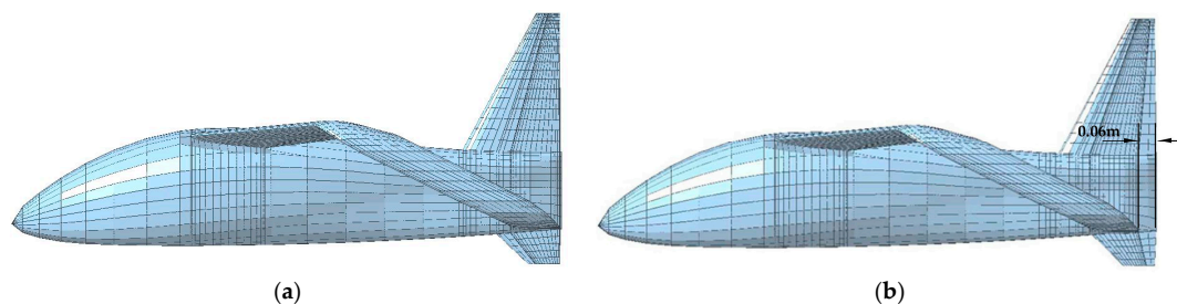
Figure 17. The airplane geometry mesh used for aerodynamic calculations: (a) baseline geometry; and (b) vertical stabilizer moved 0.06 m aft.
