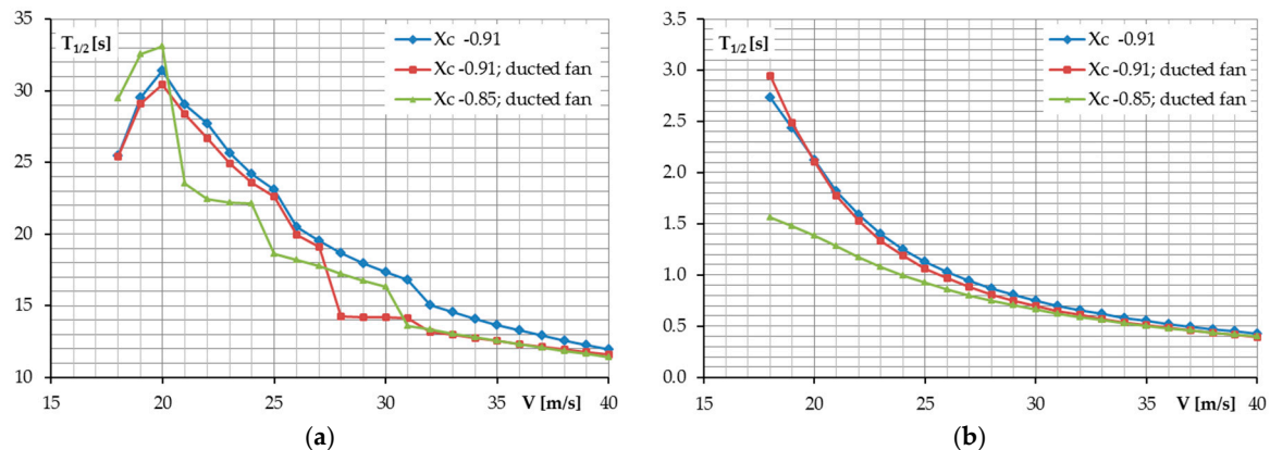
Figure 25. Dynamic stability characteristics of the airplane with ducted fan propulsion. Time to halve the amplitude of oscillations: (a) phugoid motion; and (b) Dutch roll motion.
