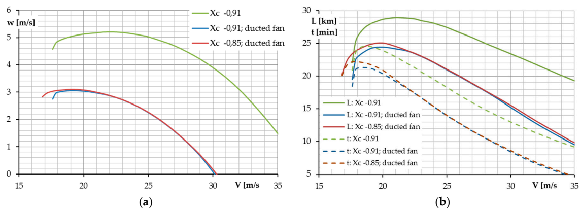
Figure 24. Variation in the airplane's performance with the thrust vector position: (a) maximum climb rate; (b) range and flight duration with respect to the airspeed.
