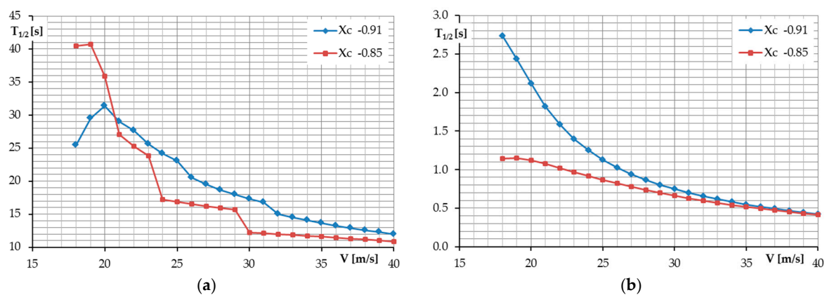
Figure 18. Dynamic stability characteristics of the airplane with the most aft CG and vertical stabilizer location. Time to halve the amplitude of the oscillations: (a) phugoid motion; and (b) Dutch roll motion.
