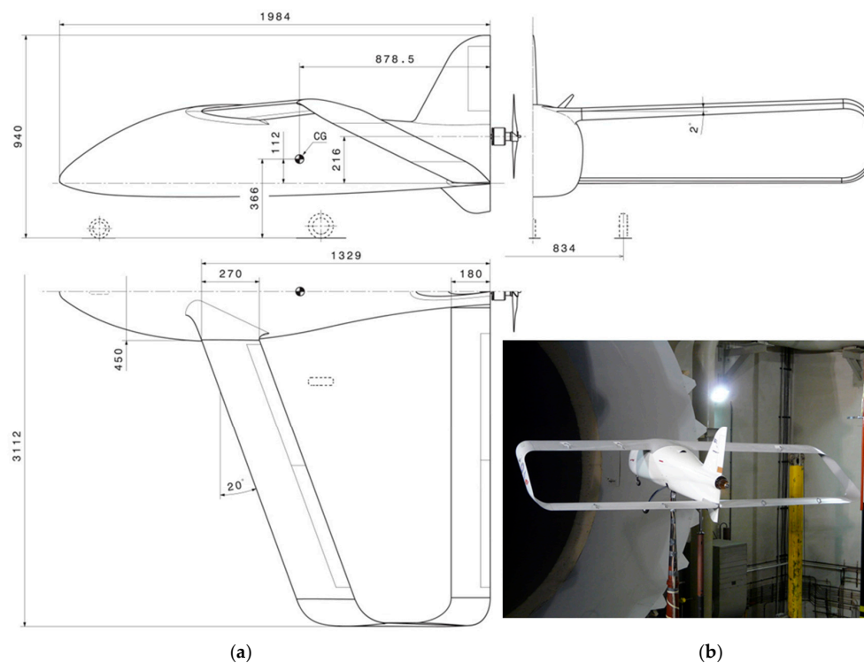
Figure 2. (a) Three views of the inverted joined wing demonstrator; and (b) demonstrator in the wind tunnel.
