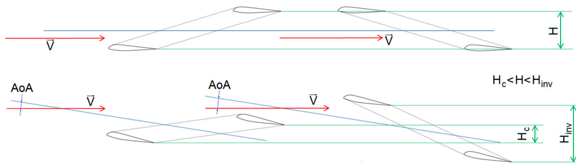
Figure 1. Distance between wings in conventional and inverted joined wings. Variation with angle of attack.
