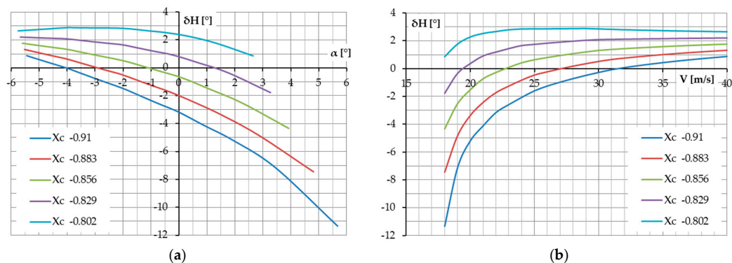
Figure 13. Elevator deflection required to trim the airplane in steady level powered flight: (a) with respect to the angle of attack; and (b) with respect to the airspeed.
