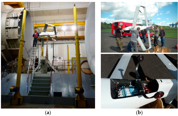
Figure 7. (a) Replacement of the batteries in the wind tunnel; and (b) replacement of the batteries during flight testing—compartment previously used for the aerodynamic balance was now used for the battery installation (photos took by Adam Dziubiński).
