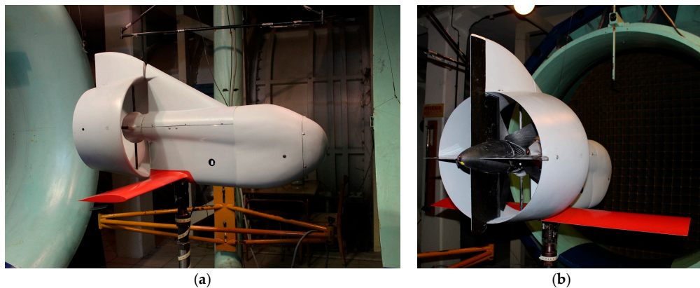
Figure 10. Test stand for propulsion testing. (a) Side view; and (b) aft view.
