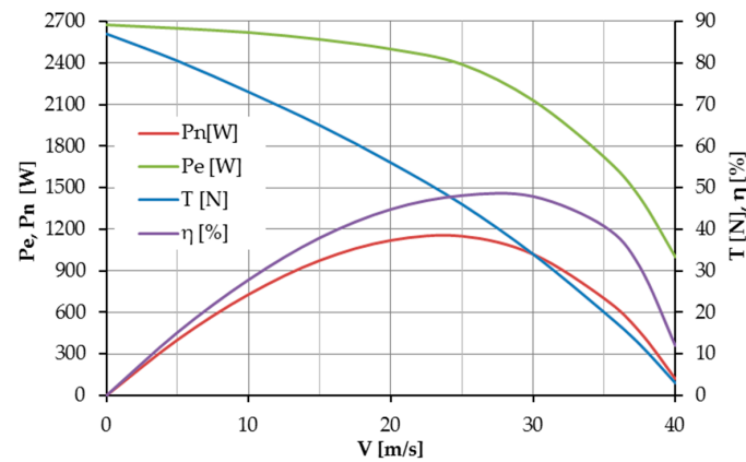
Figure 22. The ducted fan propulsion performance: P_N —effective power, P_e —motor electric power, \eta —total efficiency, T —thrust.
