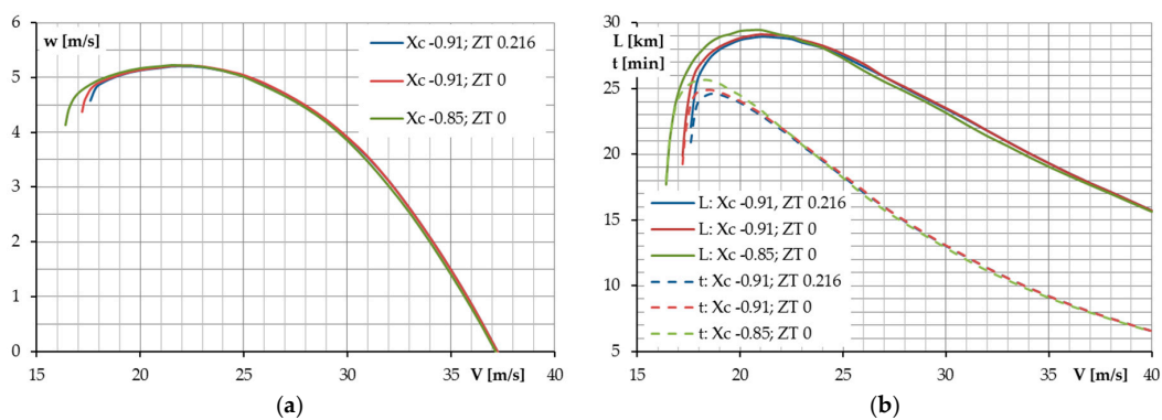
Figure 20. Variation in the airplane's performance with the thrust vector position: (a) maximum climb rate; and (b) range and flight duration with respect to the airspeed.
