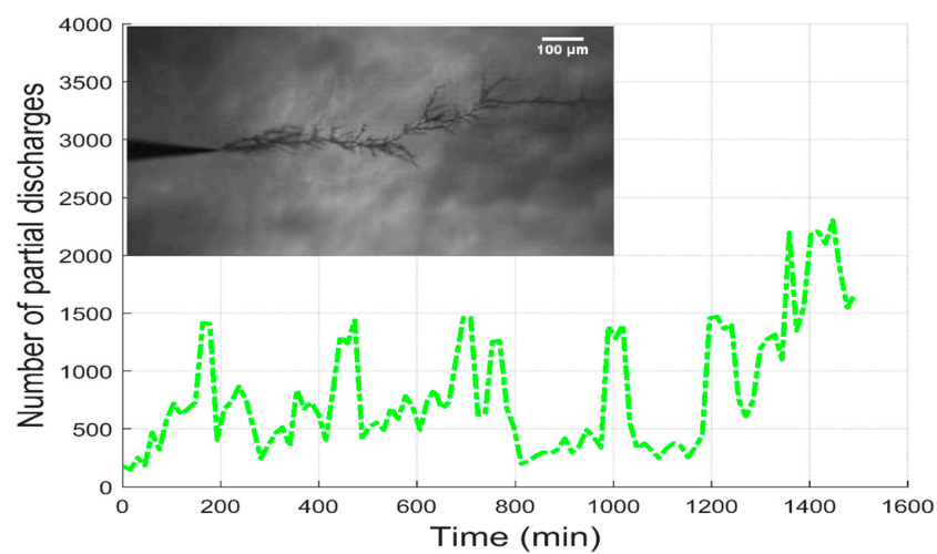
Figure 14. Partial discharge activities of ET growth under polarity reversal for case (III) in Table 4.
