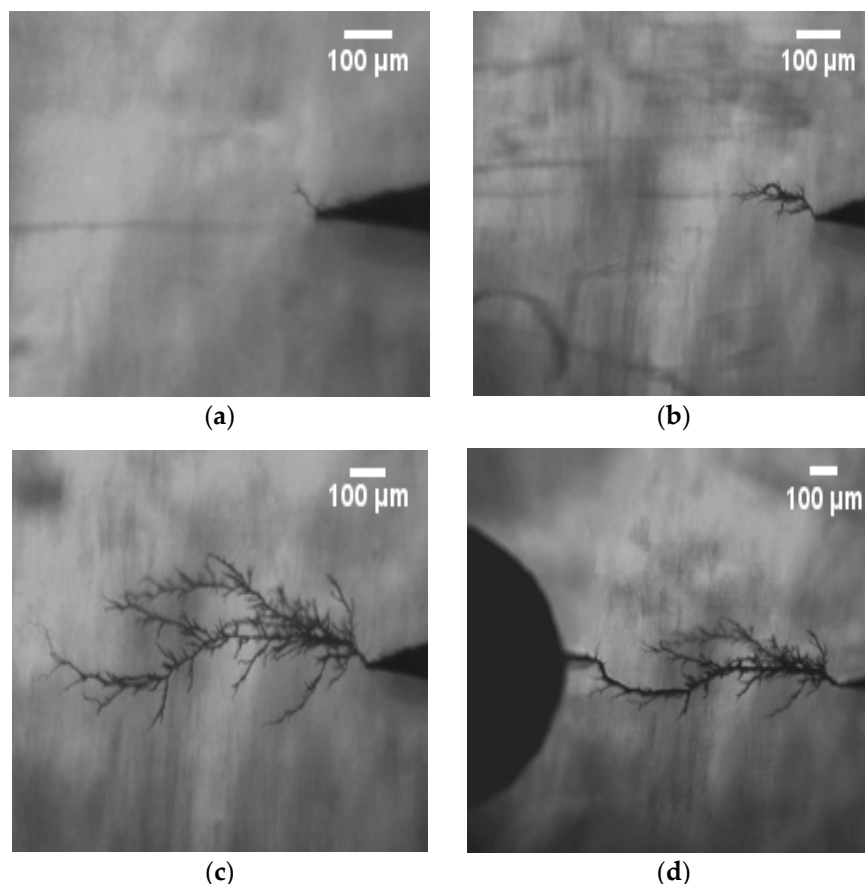
Figure 6. ET: (a) initiation; (b) development; (c) propagation; and (d) breakdown at polarity reversal of 28 kV.
