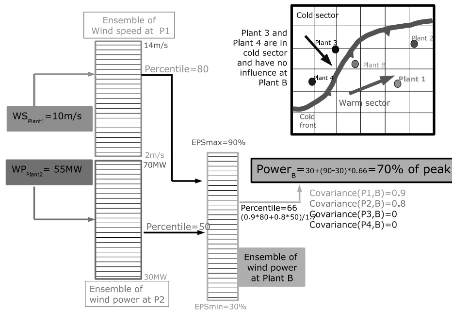
Figure 7. Functionality of the inverted Ensemble Kalman Filter when using different kind of measurements. P stands for Plant.
