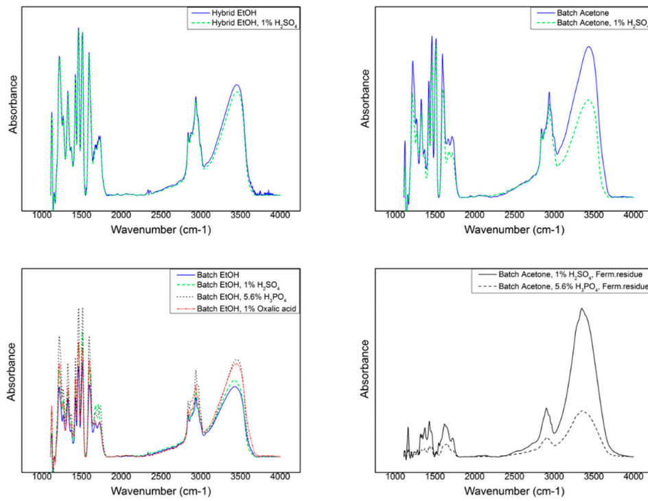
Figure S1. FTIR spectra of organosolv retrieved beechwood lignins.
